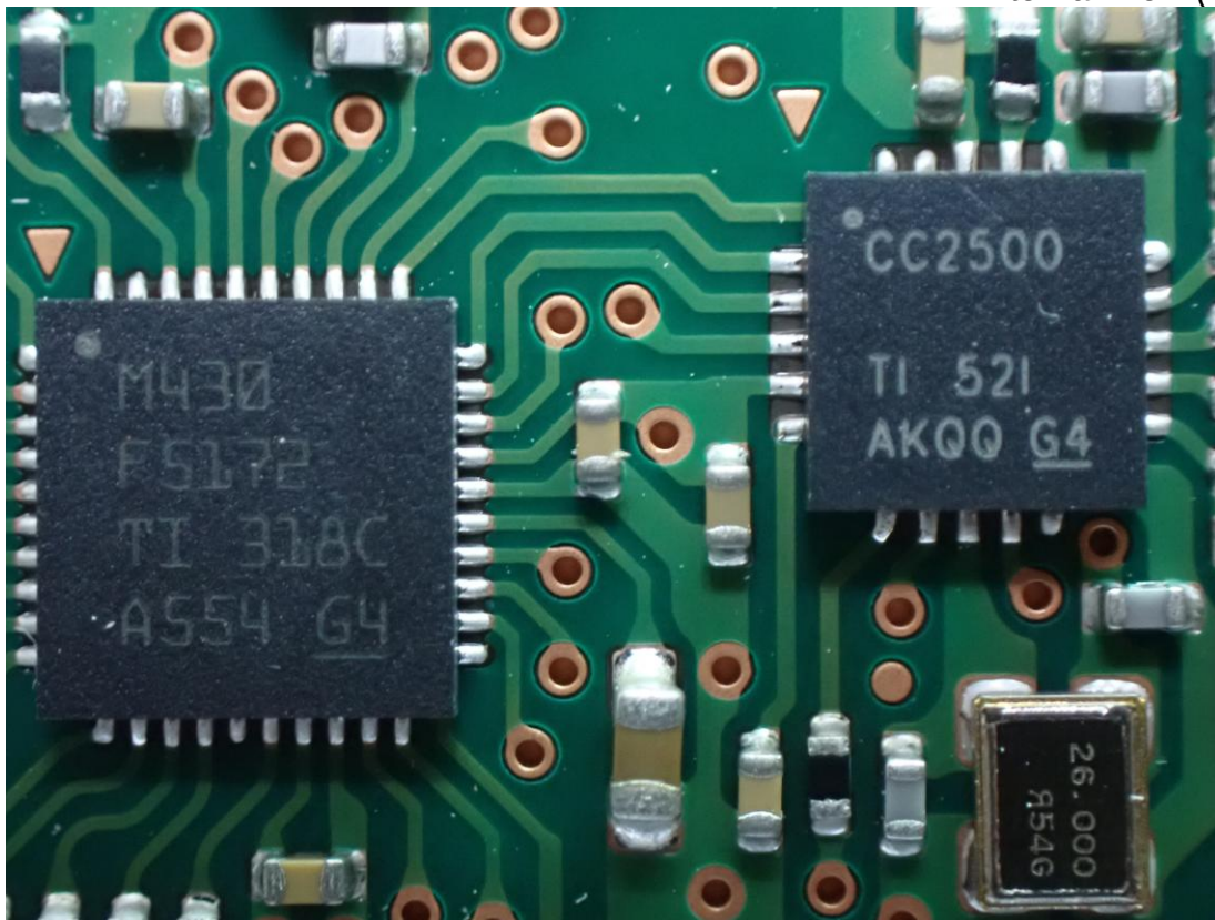
Figure 13 Internal View (RF Chip)
