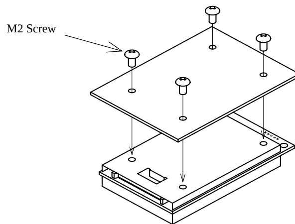
Figure 2–2: Mounting Method 2
