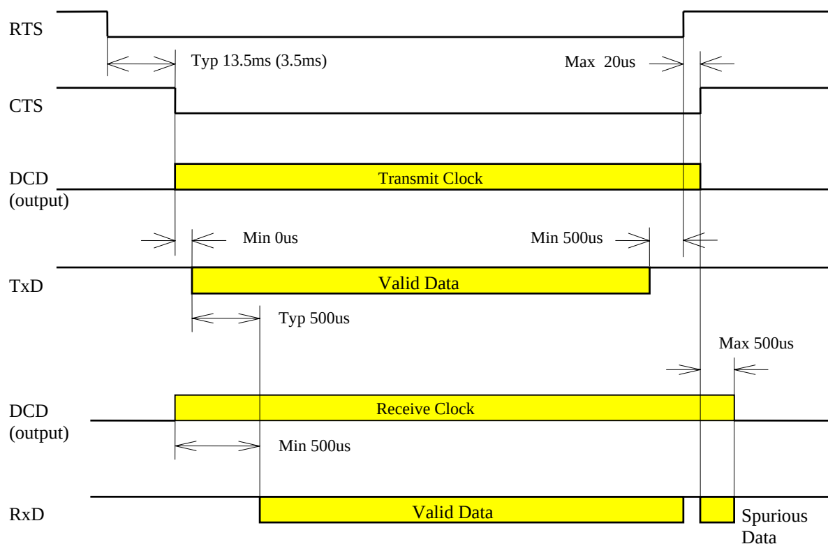
Figure 7-4: timing chart of synchronizing clock
