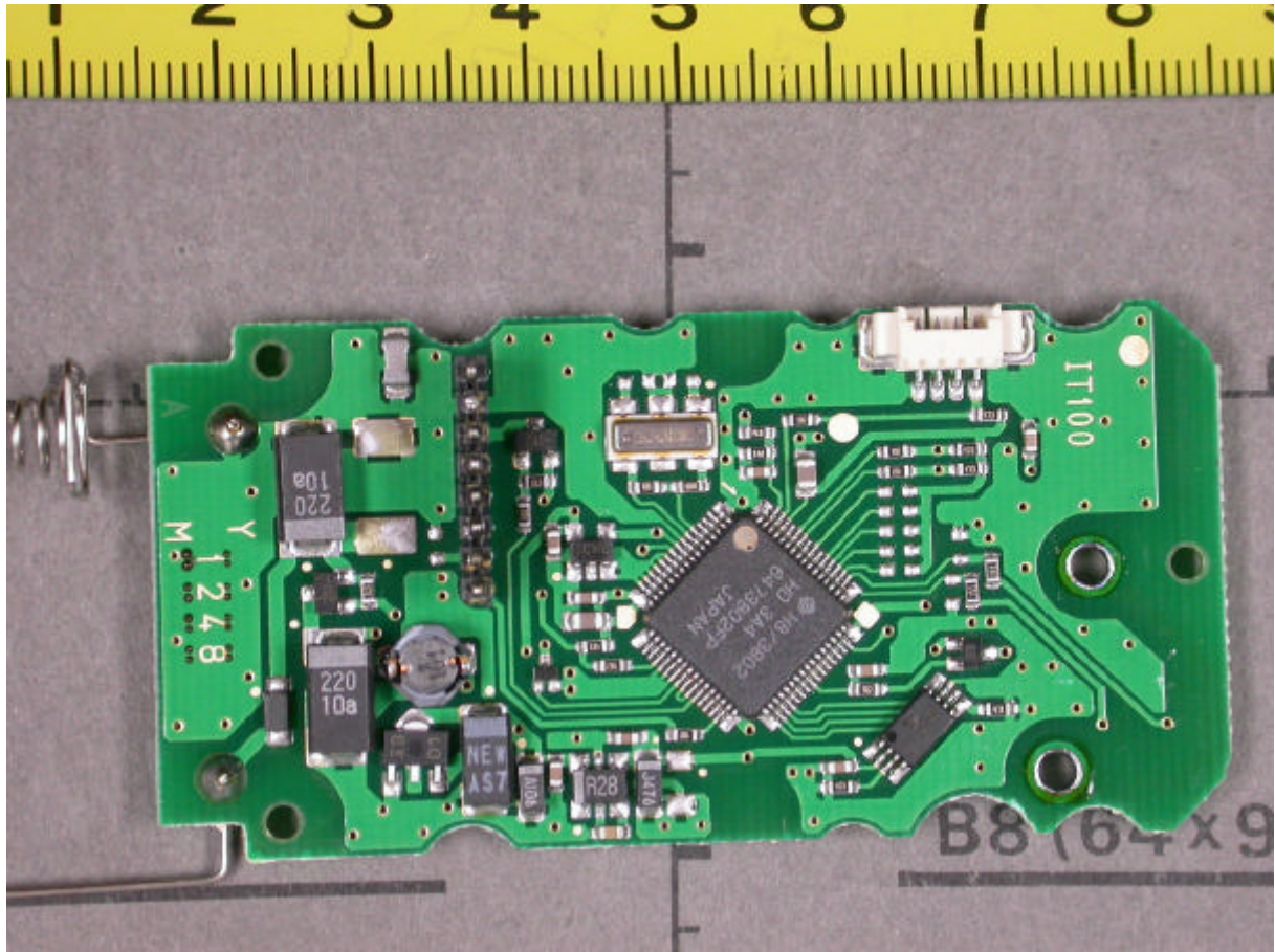
Transmitter control board top view
