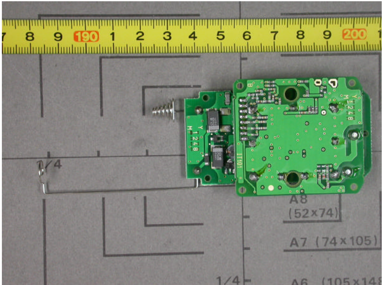
Transmitter board bottom view
