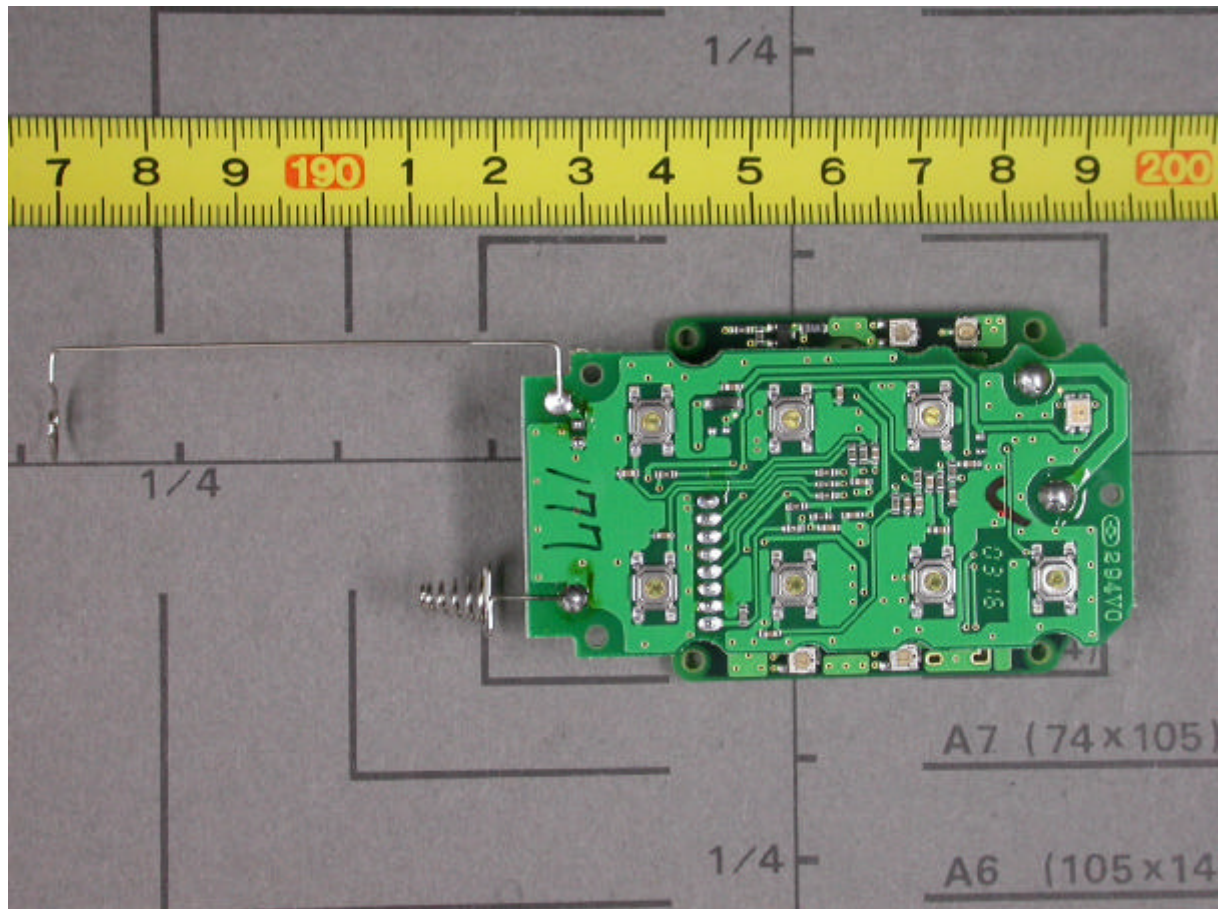
Transmitter board top view
