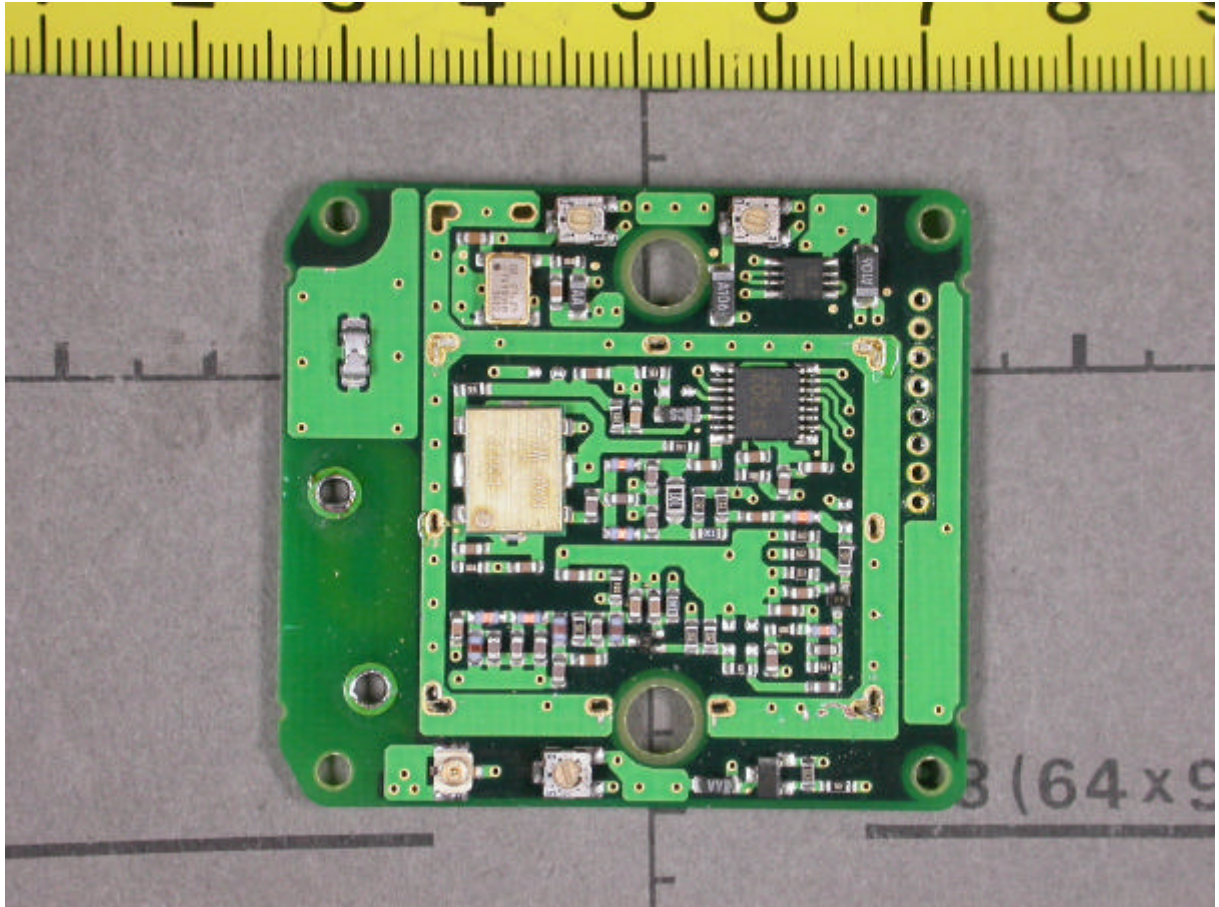
Transmitter RF board top view
