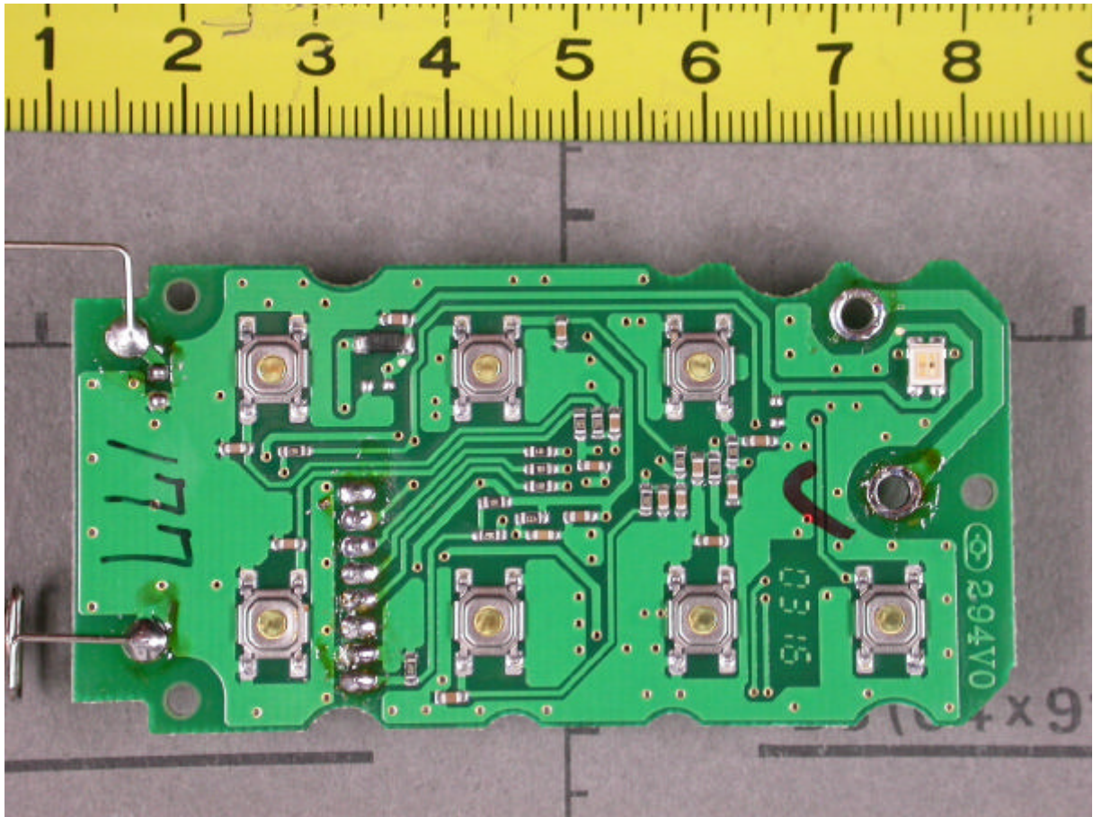
Transmitter control board bottom view
