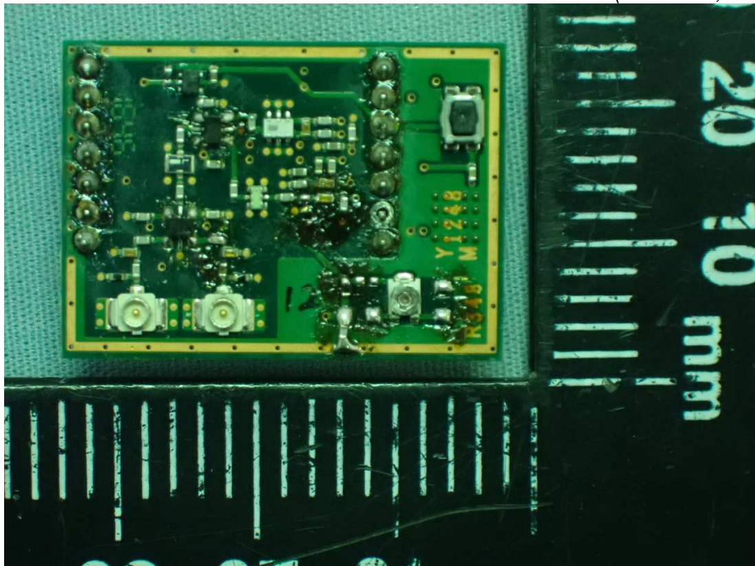
Figure 7 Internal View (RF Board, Back View)
