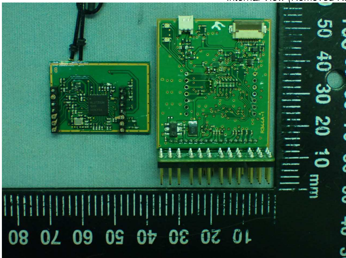
Figure 5 Internal View (Removed RF Board)
