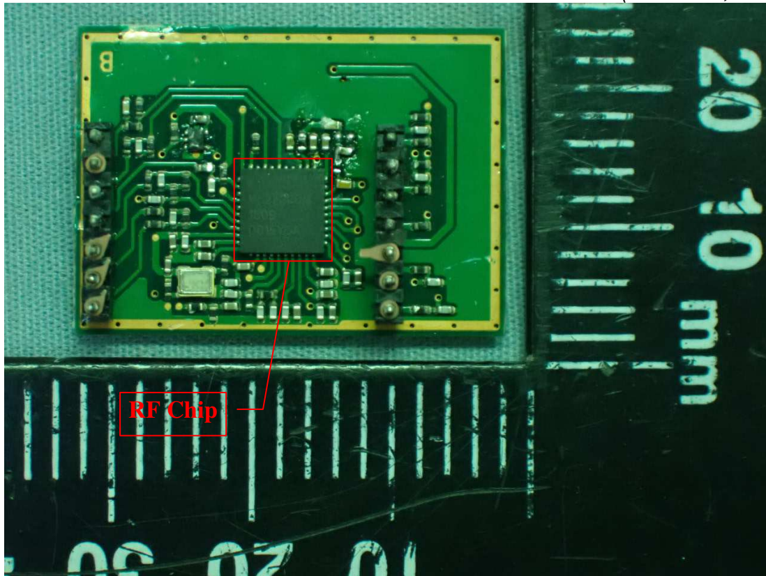
Figure 6 Internal View (RF Board, Front View)
