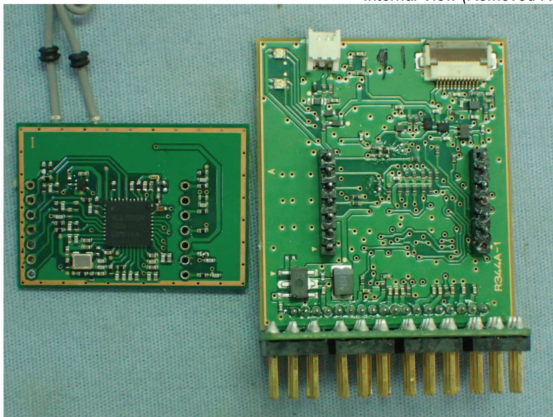
Figure 6 Internal View (Removed RF Board)
