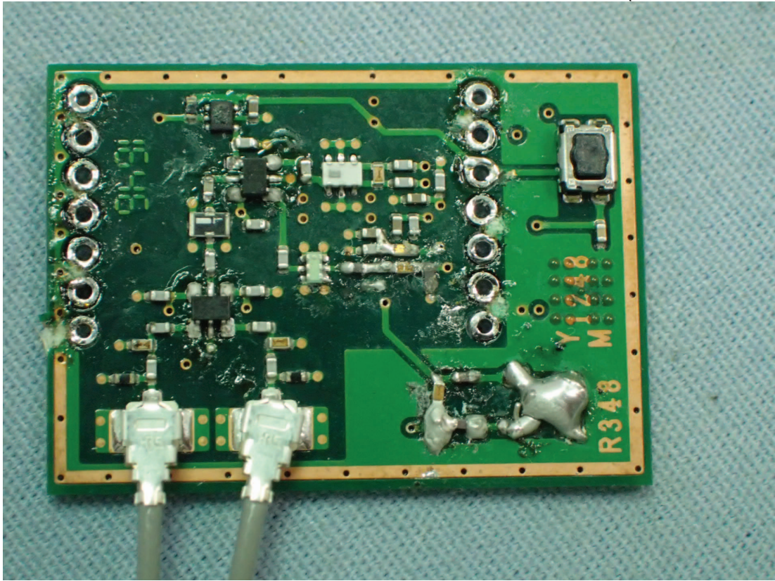
Figure 9 Internal View (RF Board, Back View)
