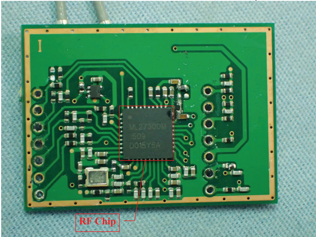
Figure 8 Internal View (RF Board, Front View)
