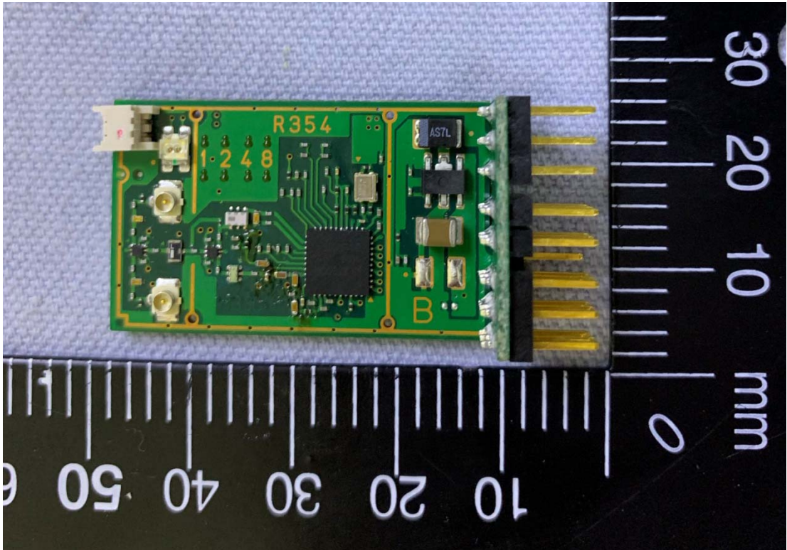
Figure 9 Main Board, Front View
