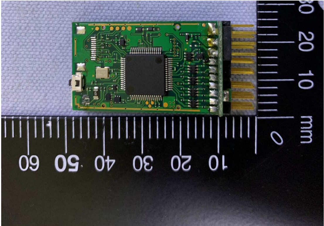
Figure 10 Main Board, Back View
