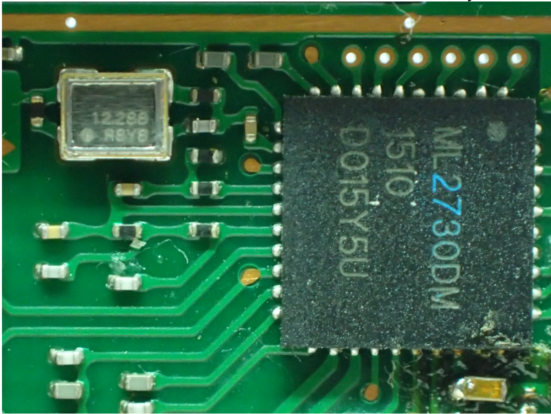
Figure 11 Crystal View
