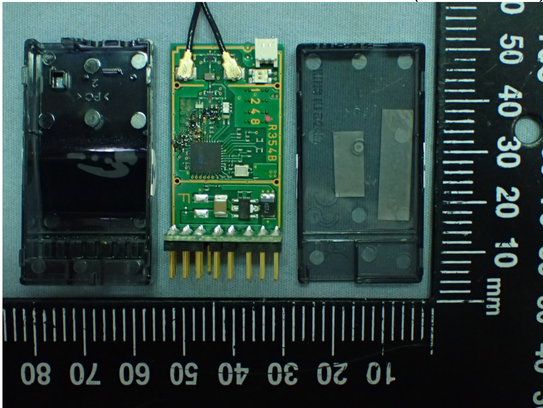
Figure 7 Internal View (Removed Covers)
