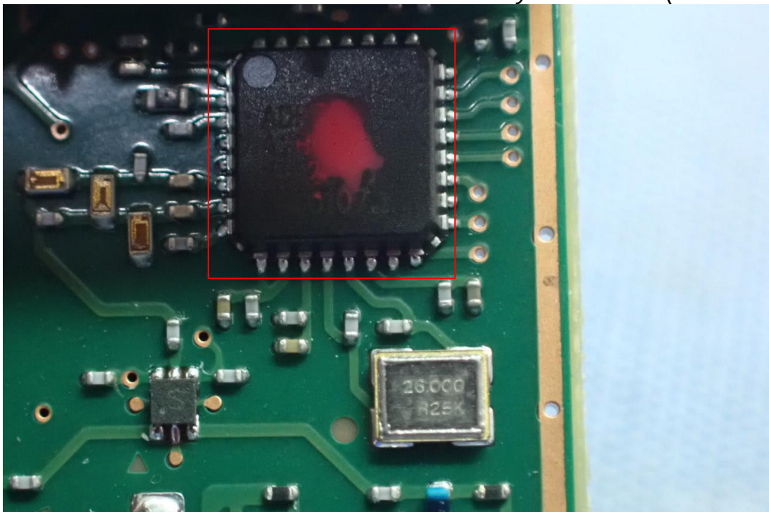
Figure 26 Crystal & RF IC (ADF7242) View
