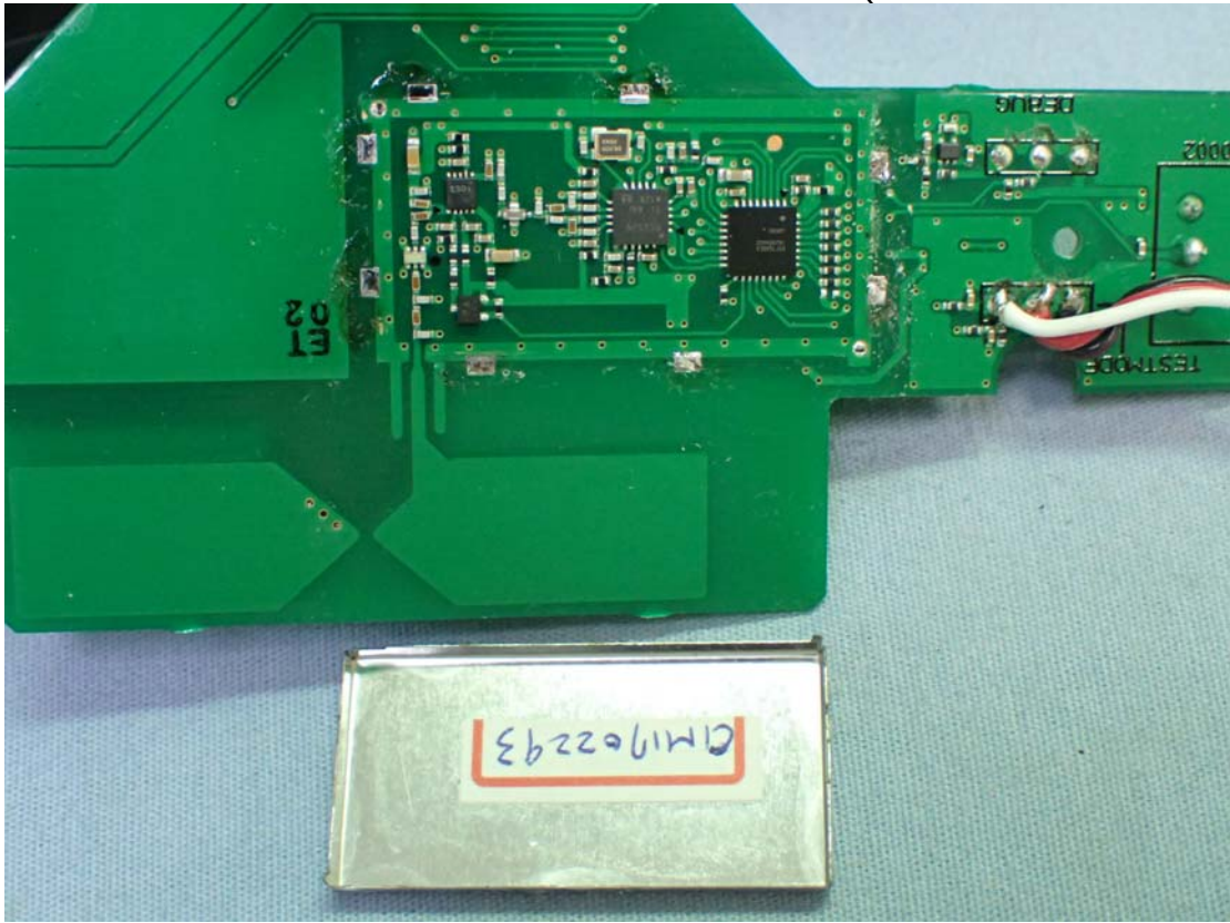
Figure 7 Internal View (Removed Metal Cover)
