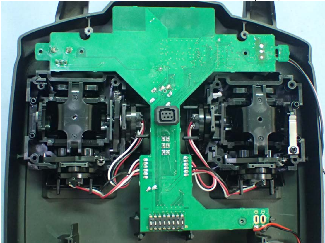
Figure 5 Internal View (PCB, Front View)
