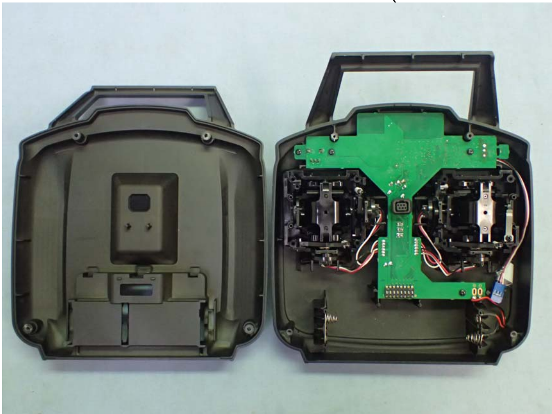
Figure 4 Internal View (Removed Back Cover)
