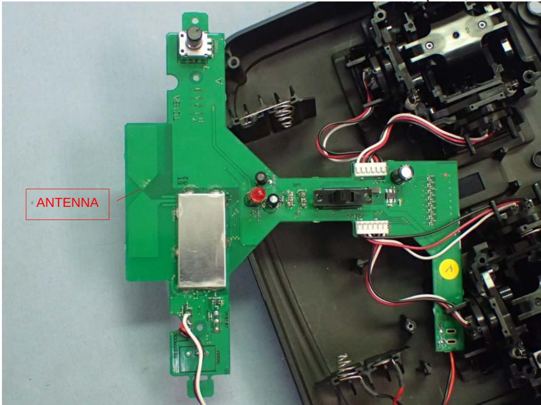
Figure 6 Internal View (PCB, Back View)
