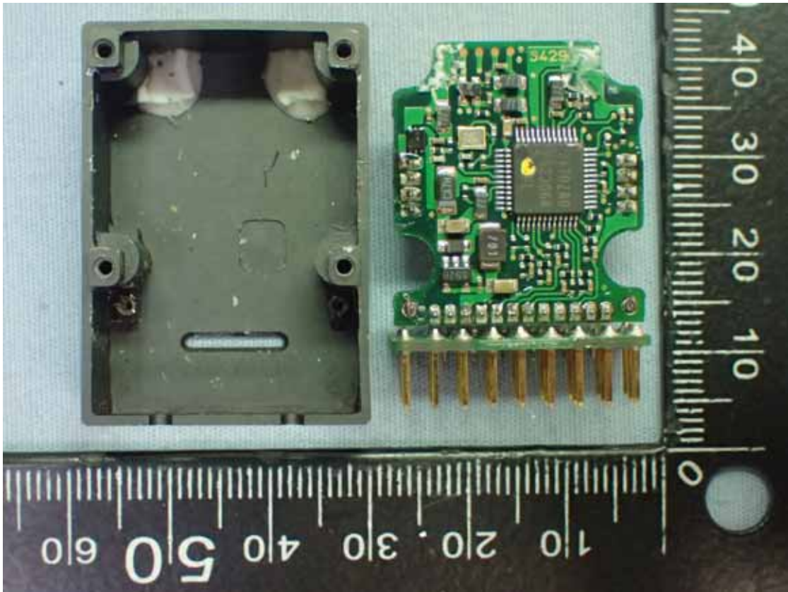
Figure 5 Internal View
