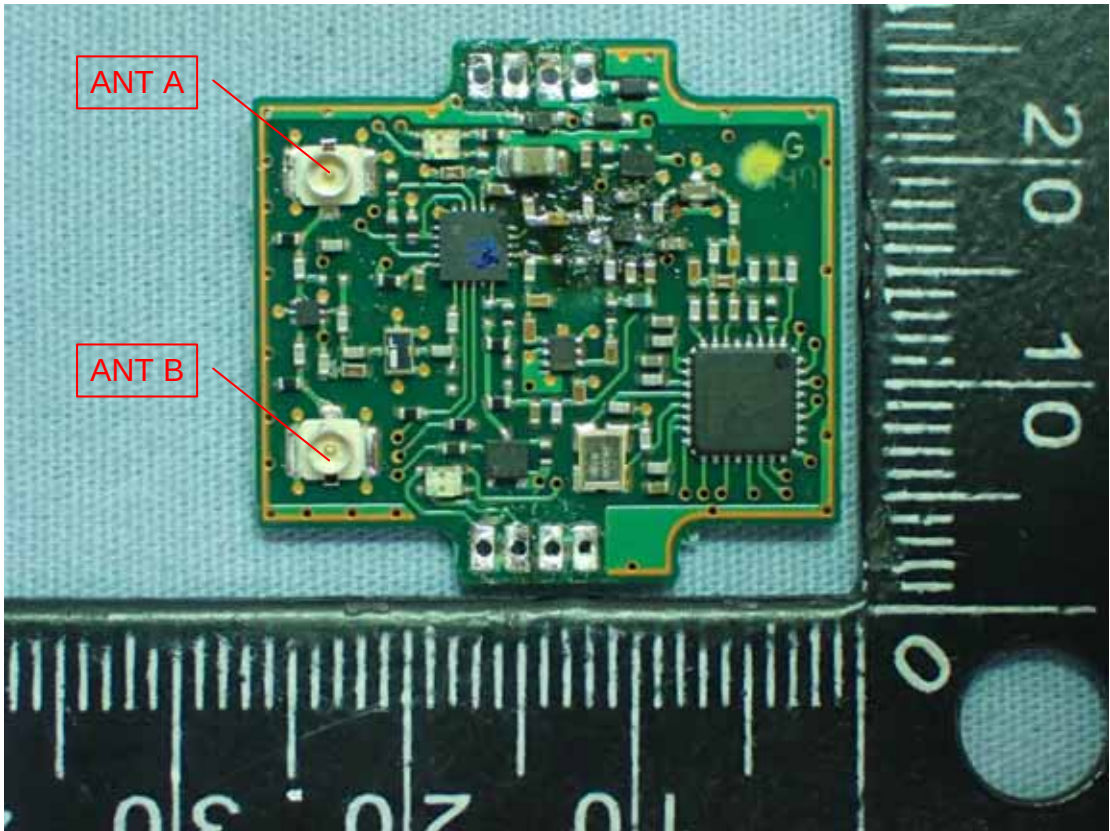
Figure 8 R341B RF Board, Back View
