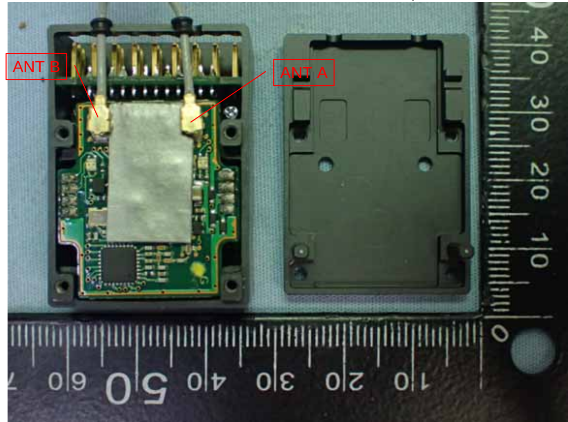
Figure 3 Internal View (Remove Cover View)
