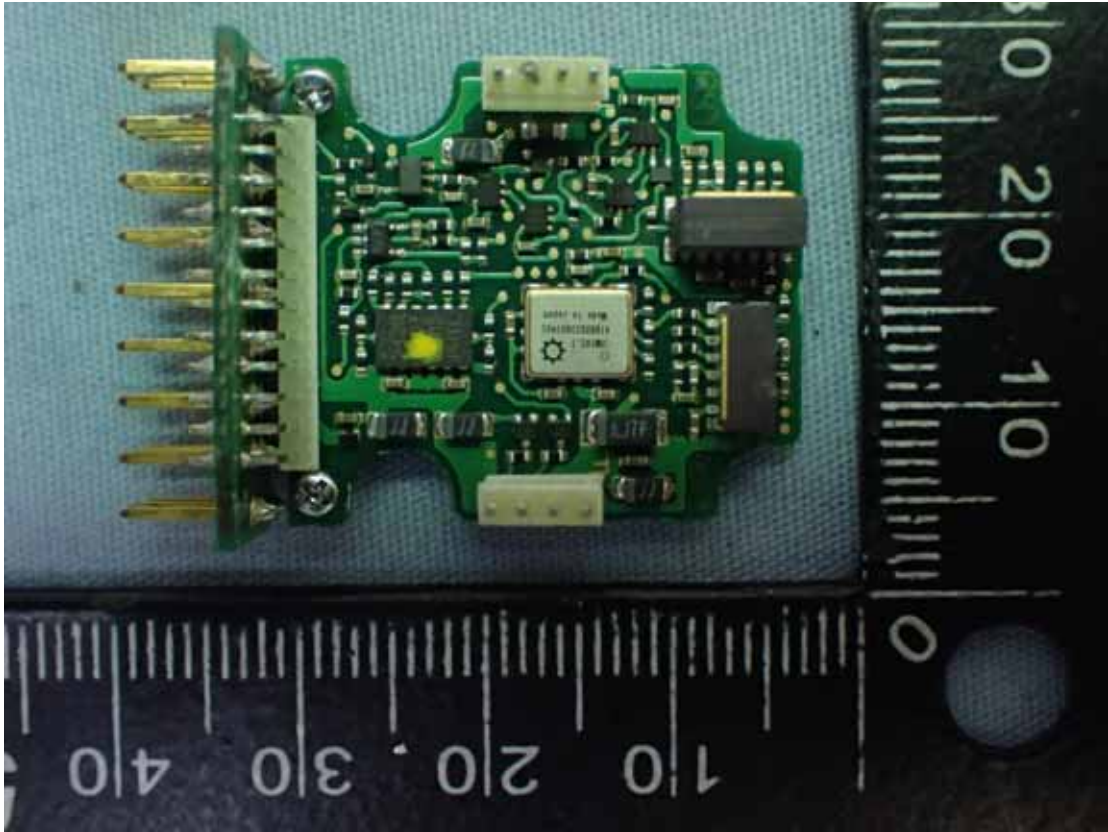
Figure 10 S429 Main Board, Back View
