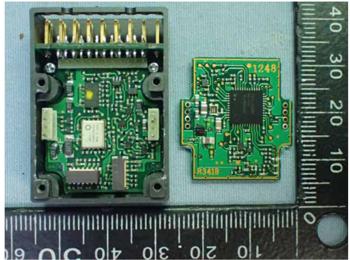
Figure 4 Internal View
