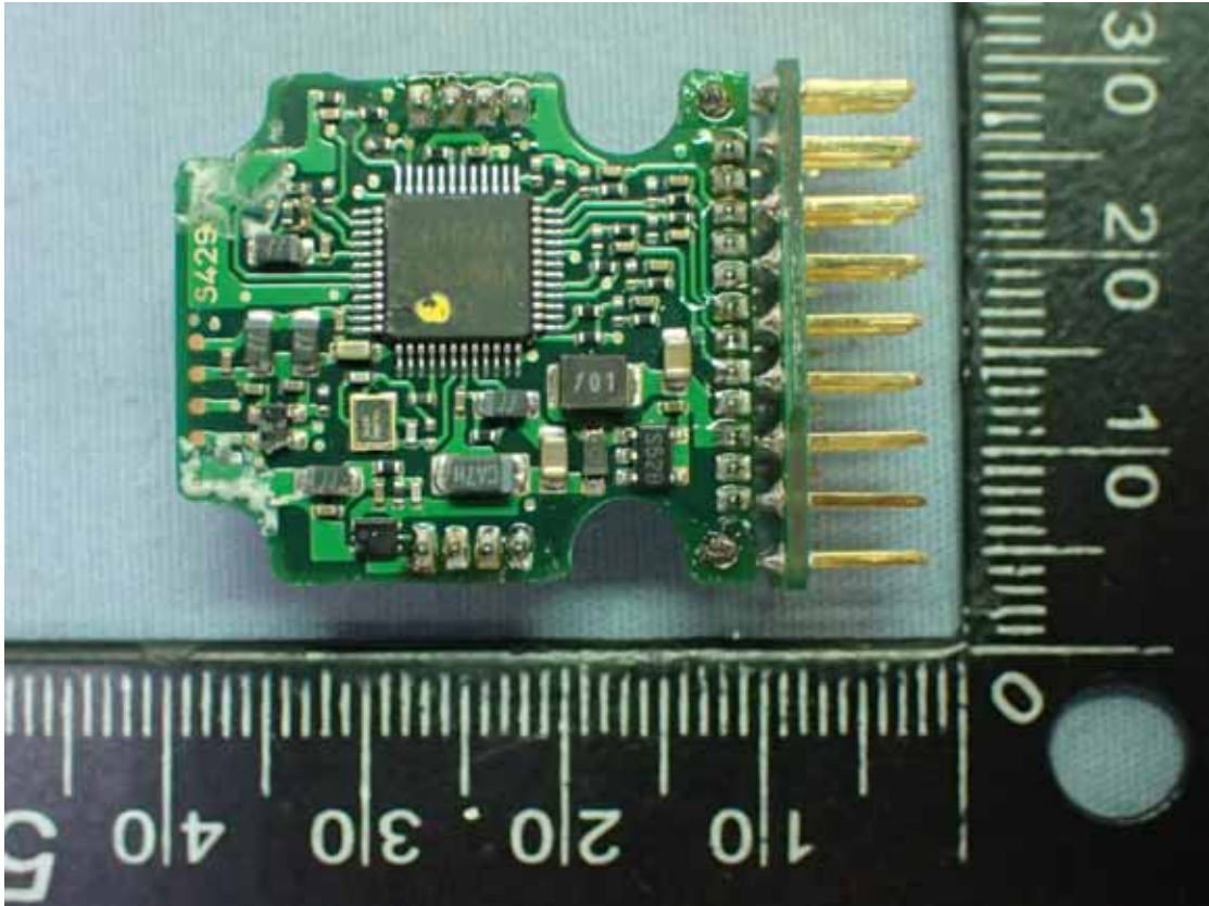
Figure 9 S429 Main Board, Front View
