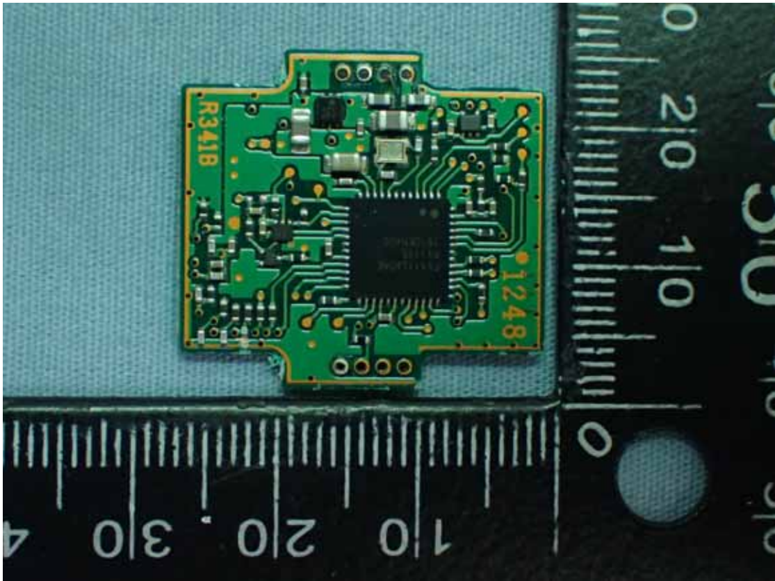
Figure 7 R341B RF Board, Front View
