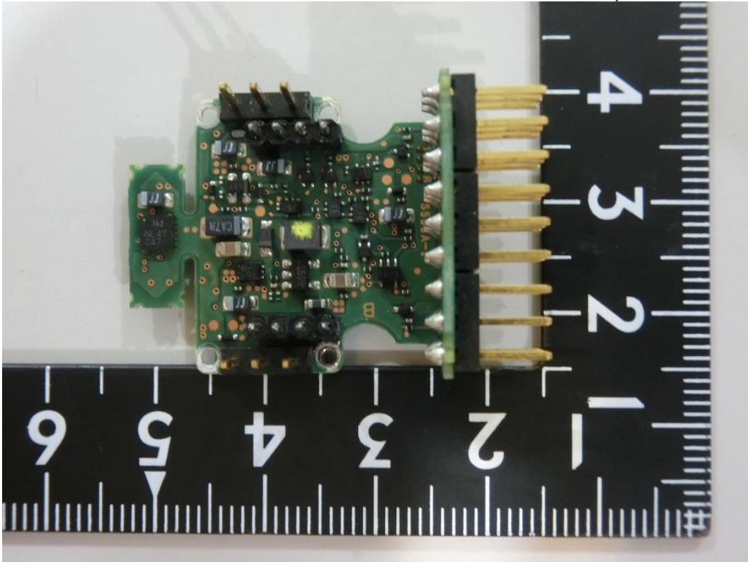
Figure 11 Internal View (RF Board, Back View)
