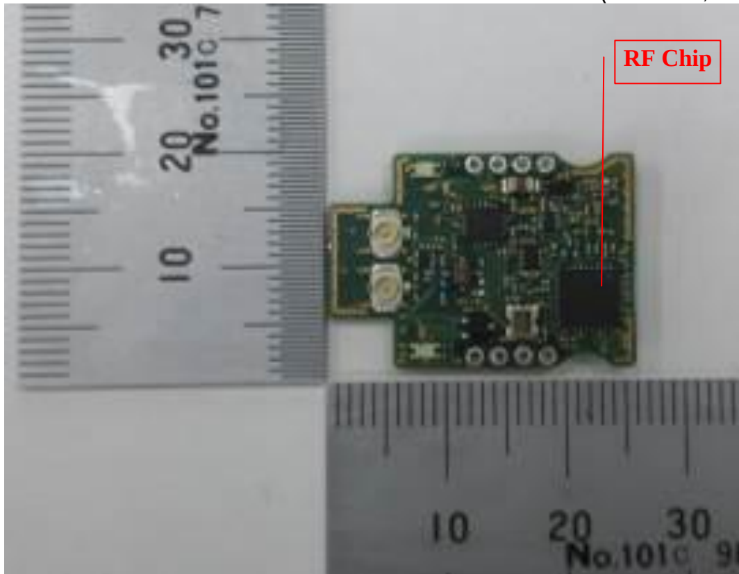
Figure 9 Internal View (RF Board, Back View)
