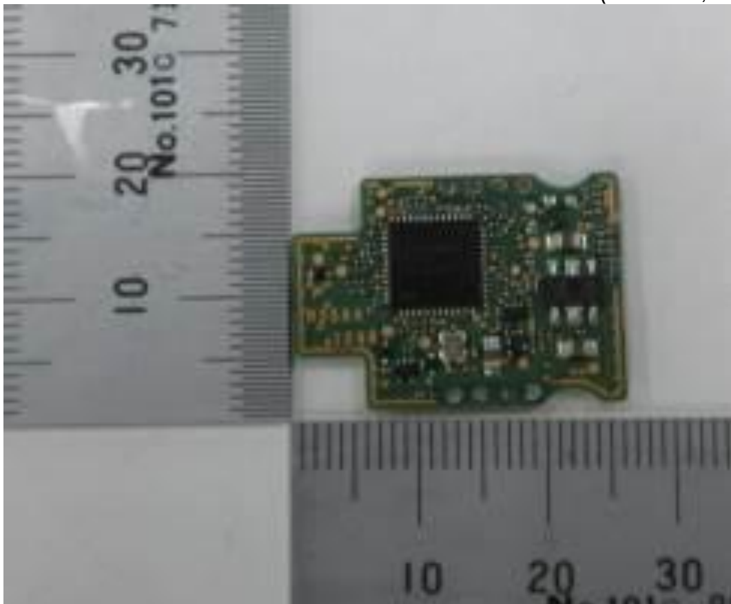
Figure 9 Internal View (RF Board, Back View)
