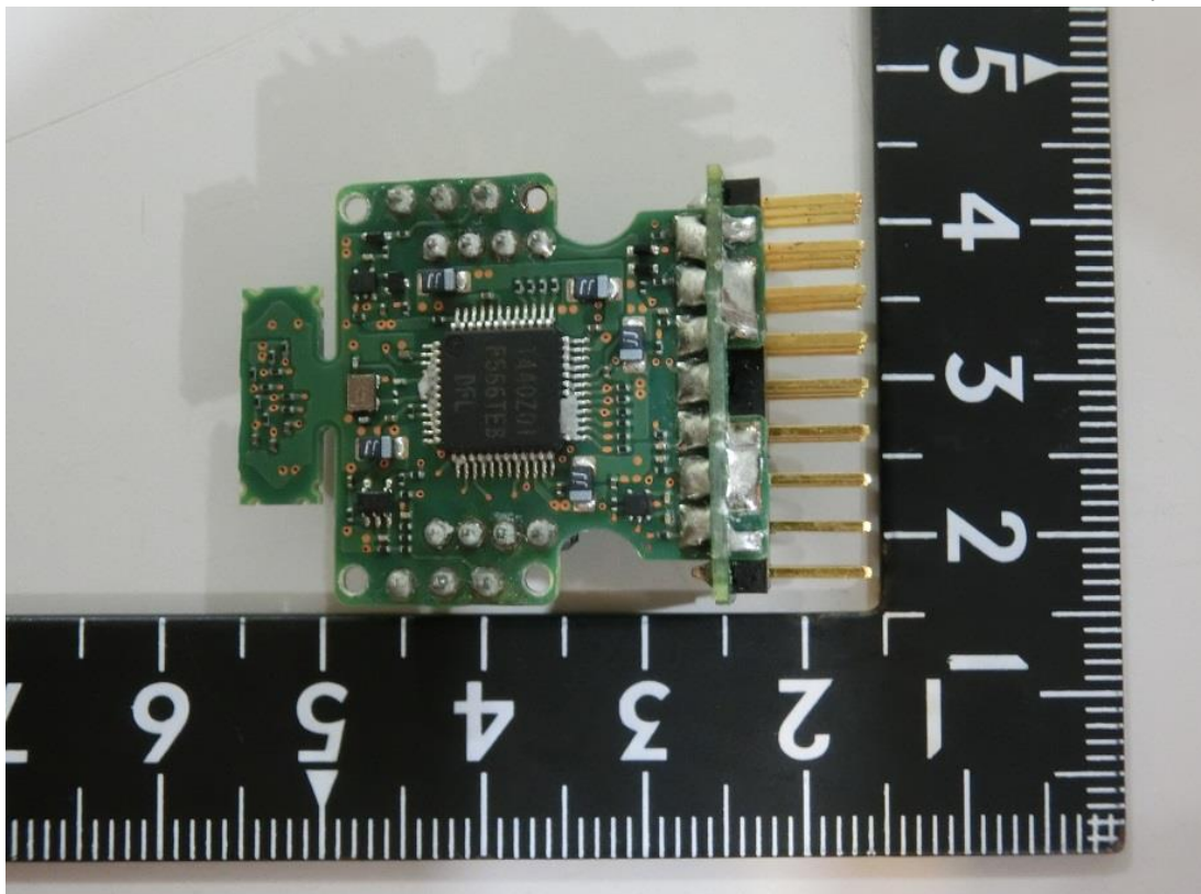
Figure 11 PCB, Back View
