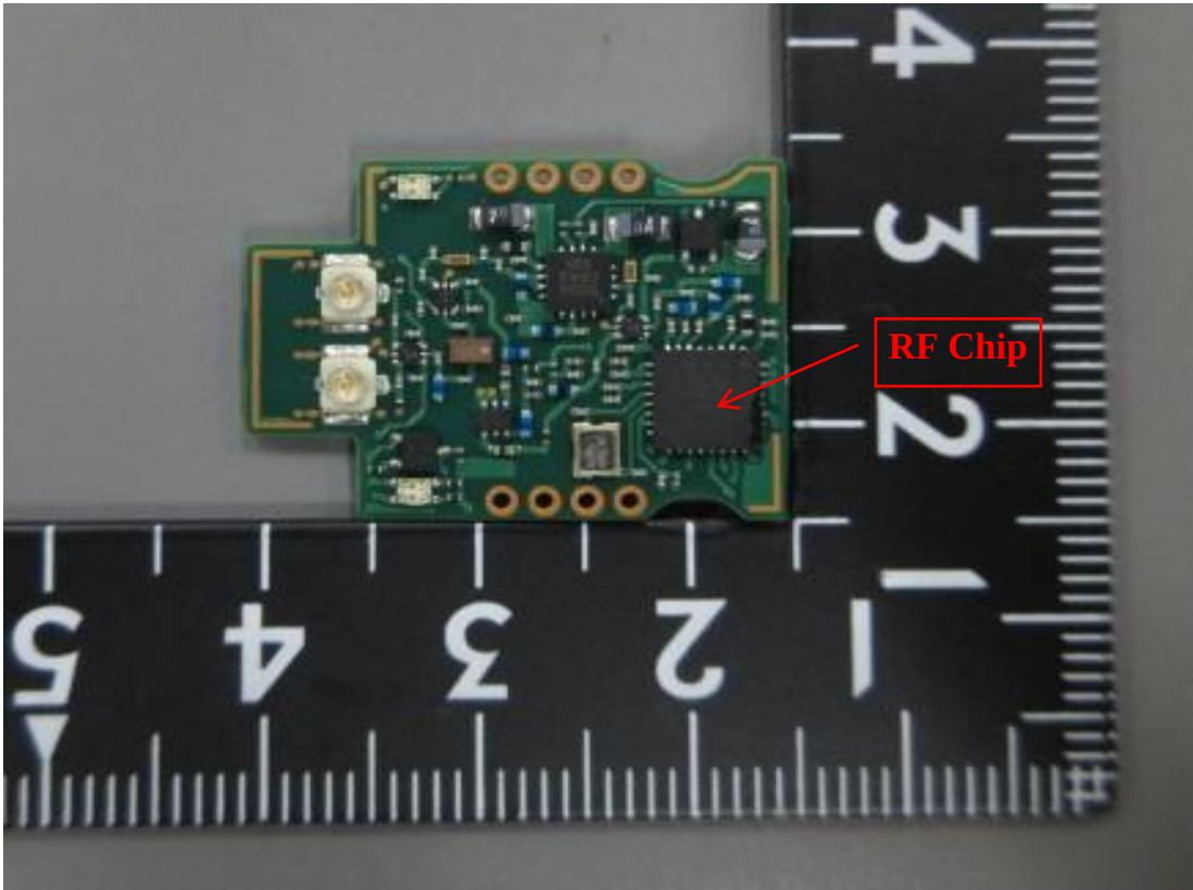
Figure 13 Internal View (RF Board, Back View)
