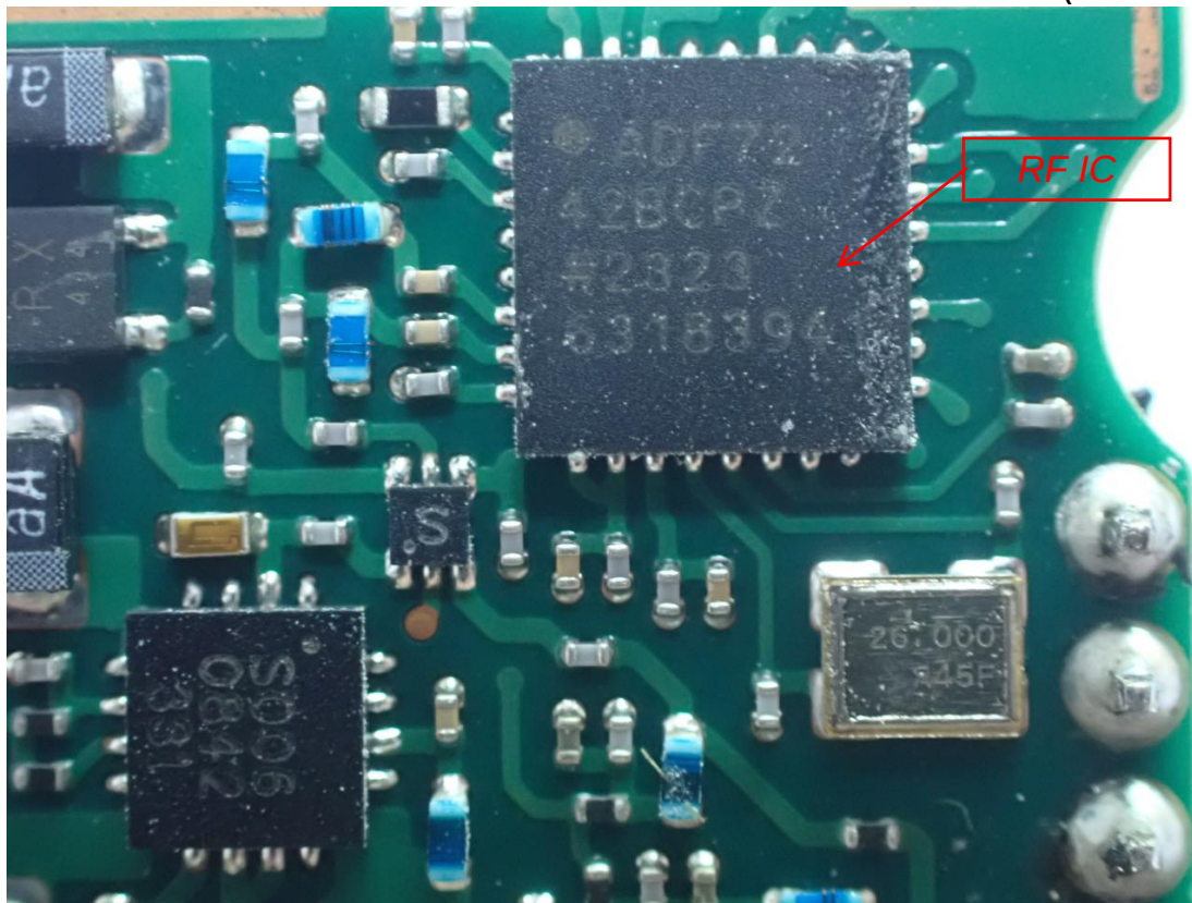
Figure 14 RF IC (ADF7242) View
