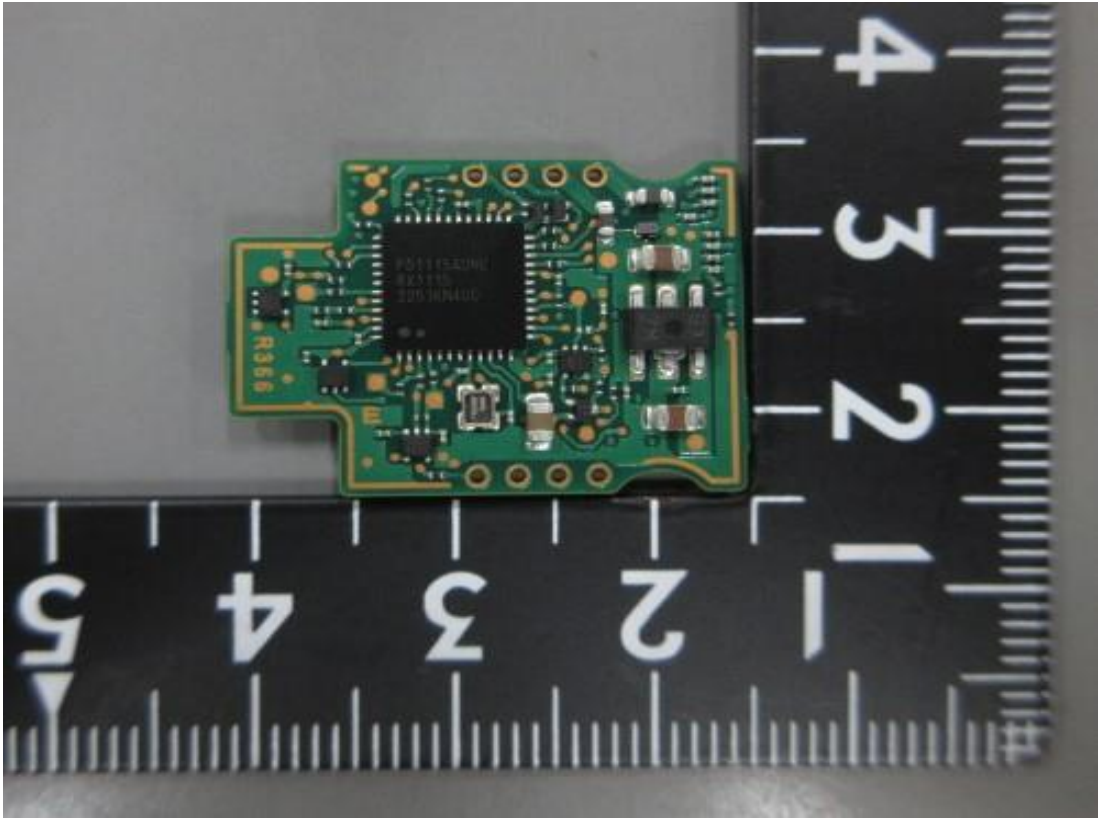
Figure 12 Internal View (RF Board, Front View)
