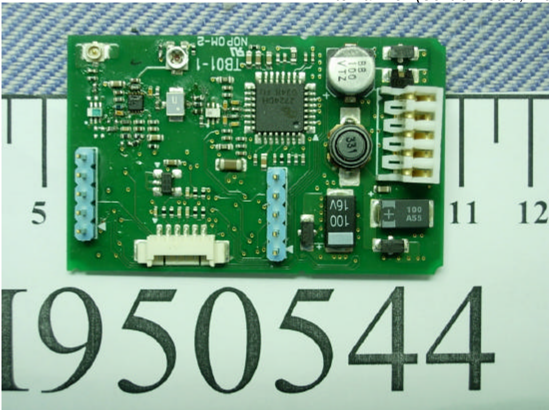
Figure 6 Internal View(Control Board, Front View)
