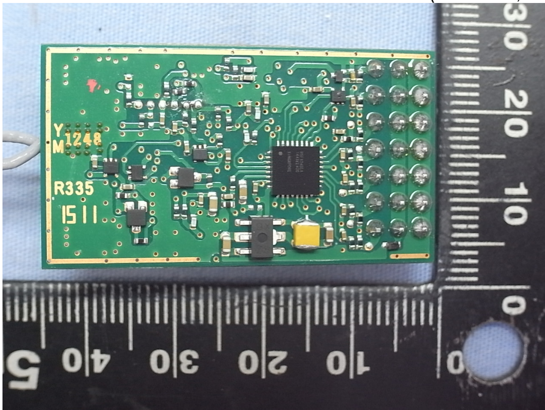
Figure 5 Internal View (Main Board, Back View)
