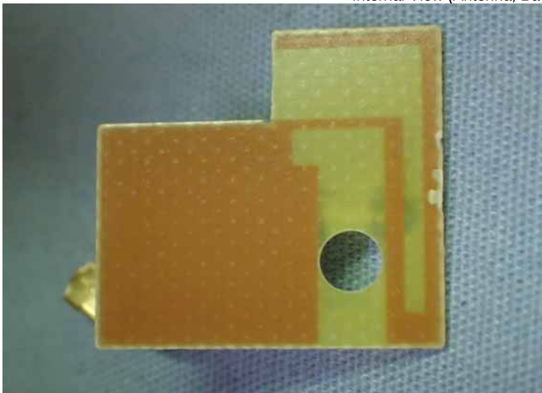
Figure 8 Internal View (Antenna, Back View)
