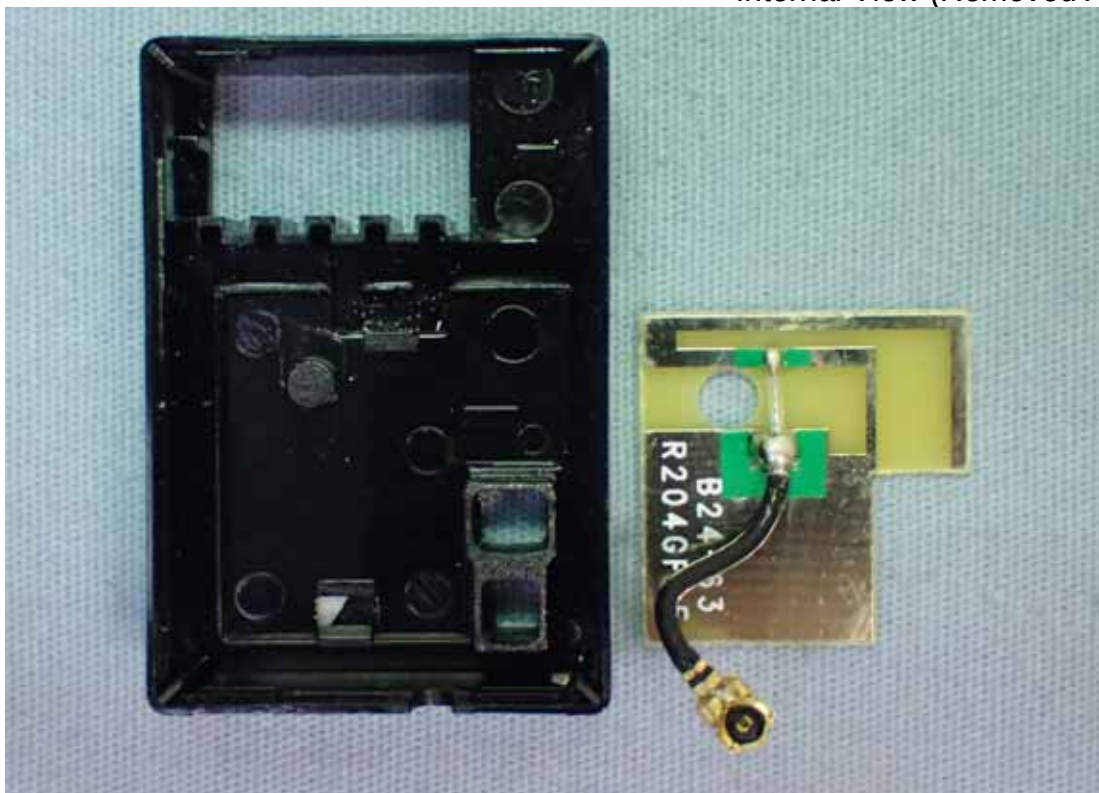
Figure 6 Internal View (Removed Antenna)
