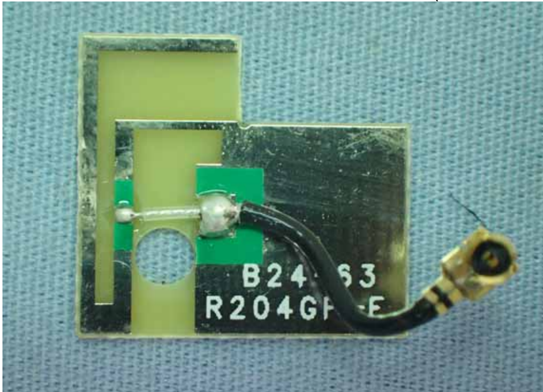
Figure 7 Internal View (Antenna d, Front View)
