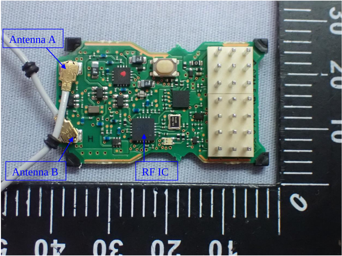
Figure 7 Internal View (Main Board)
