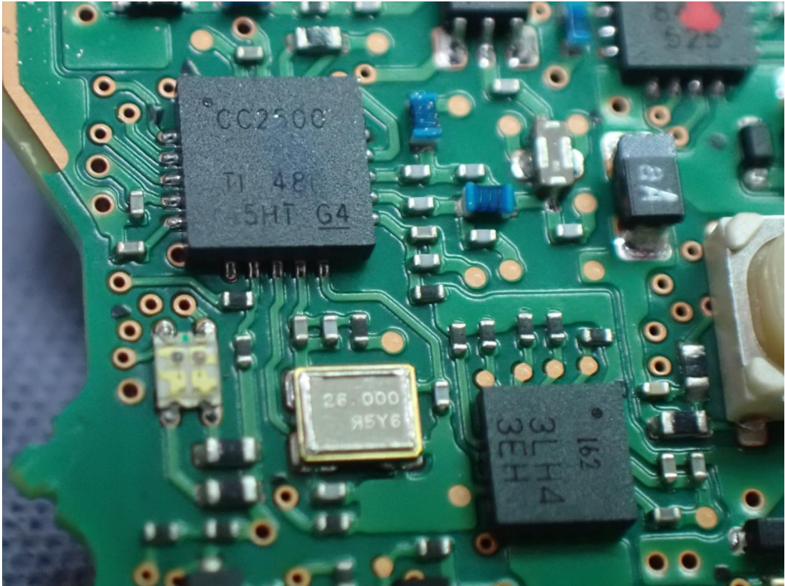
Figure 8 Internal View (RF IC: CC2500)
