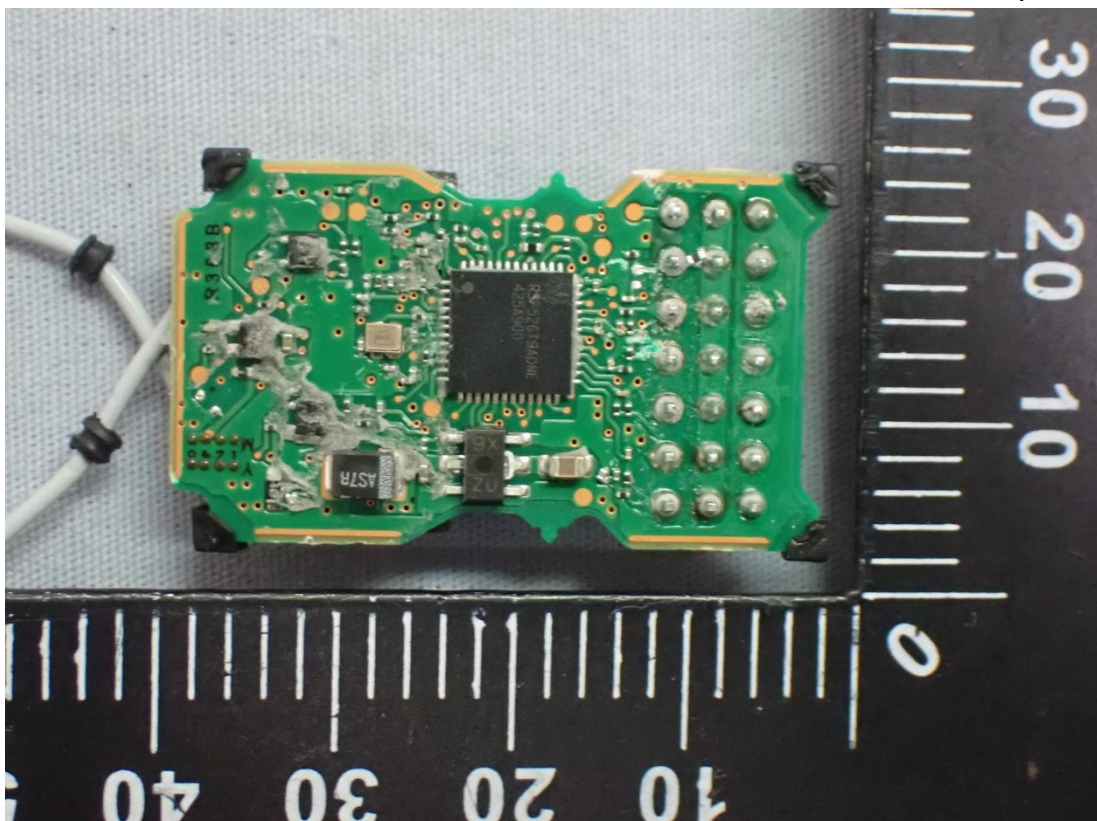
Figure 6 Internal View (Main Board)
