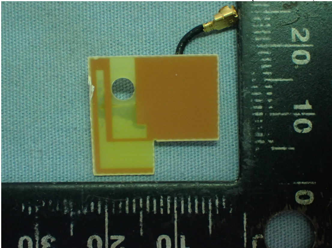
Figure 8 Internal View (PCB Antenna, Back View)
