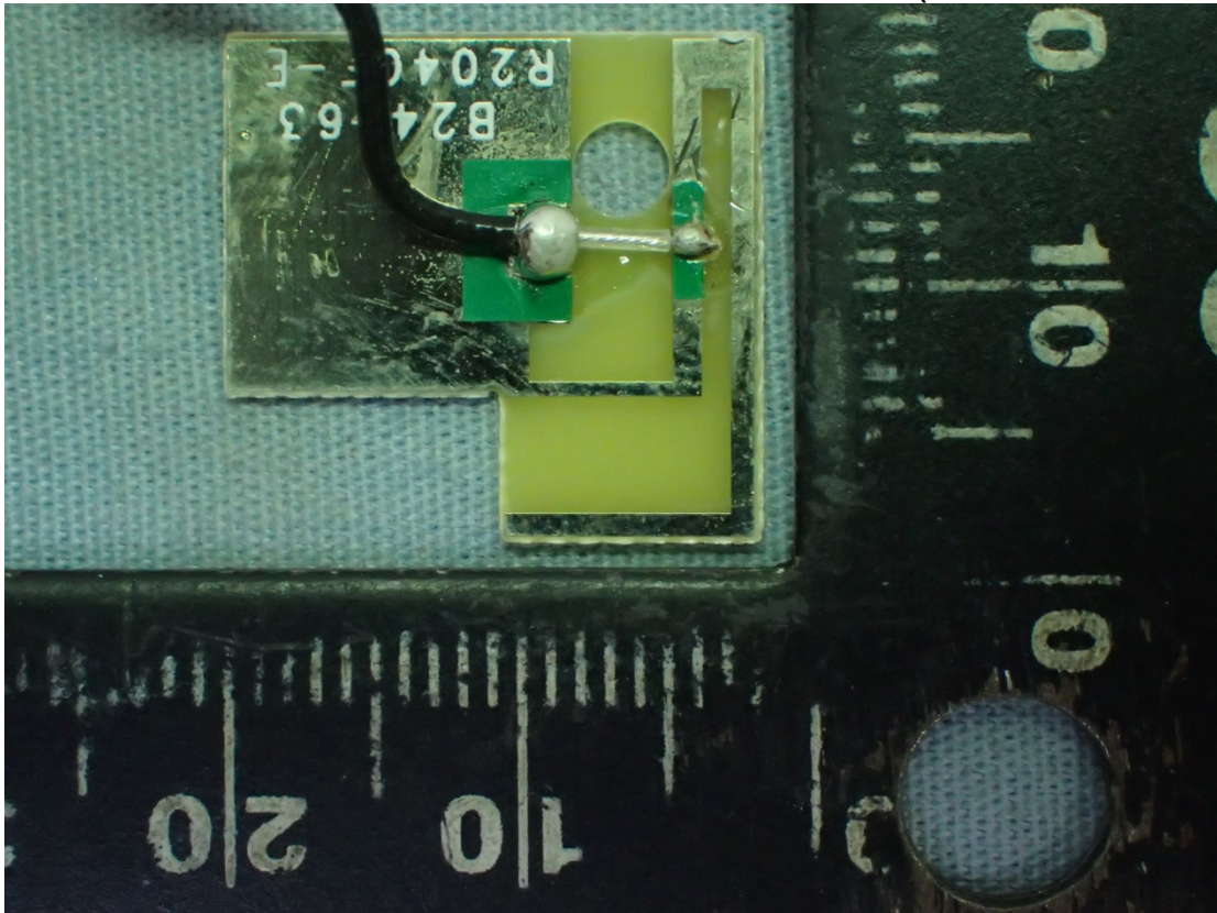
Figure 7 Internal View (PCB Antenna, Front View)
