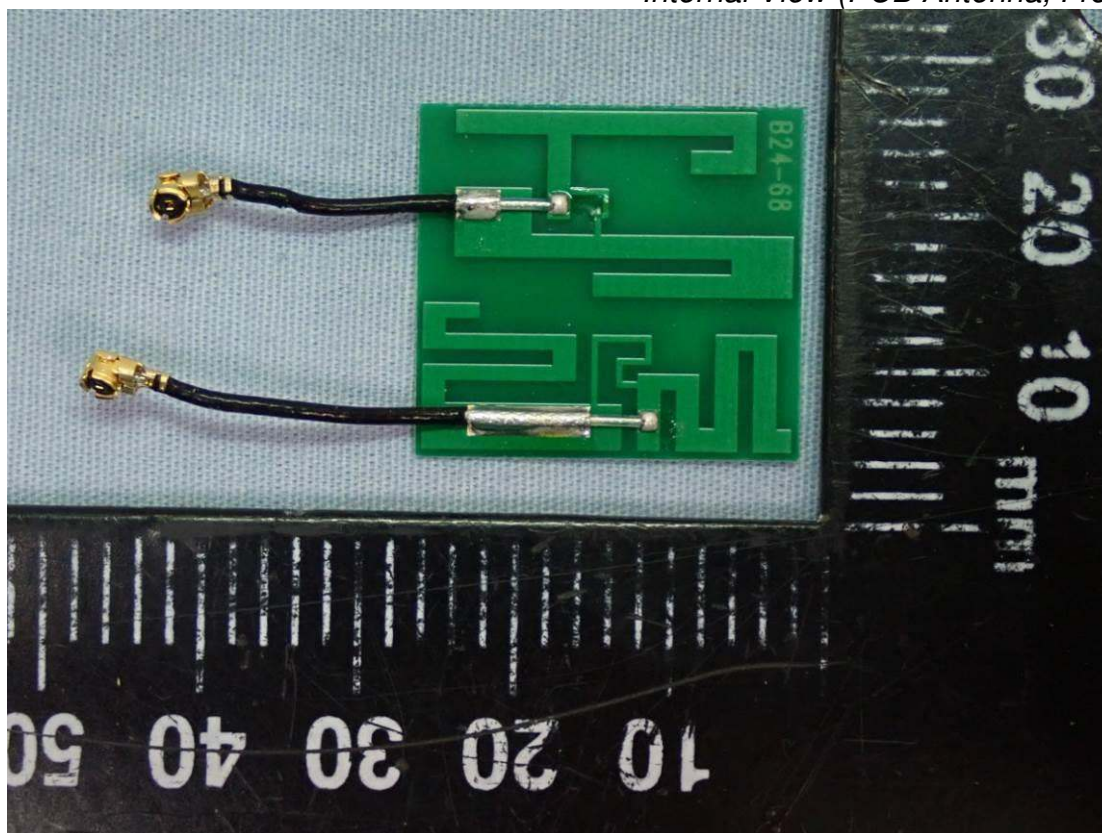
Figure 24 Internal View (PCB Antenna, Front View)
