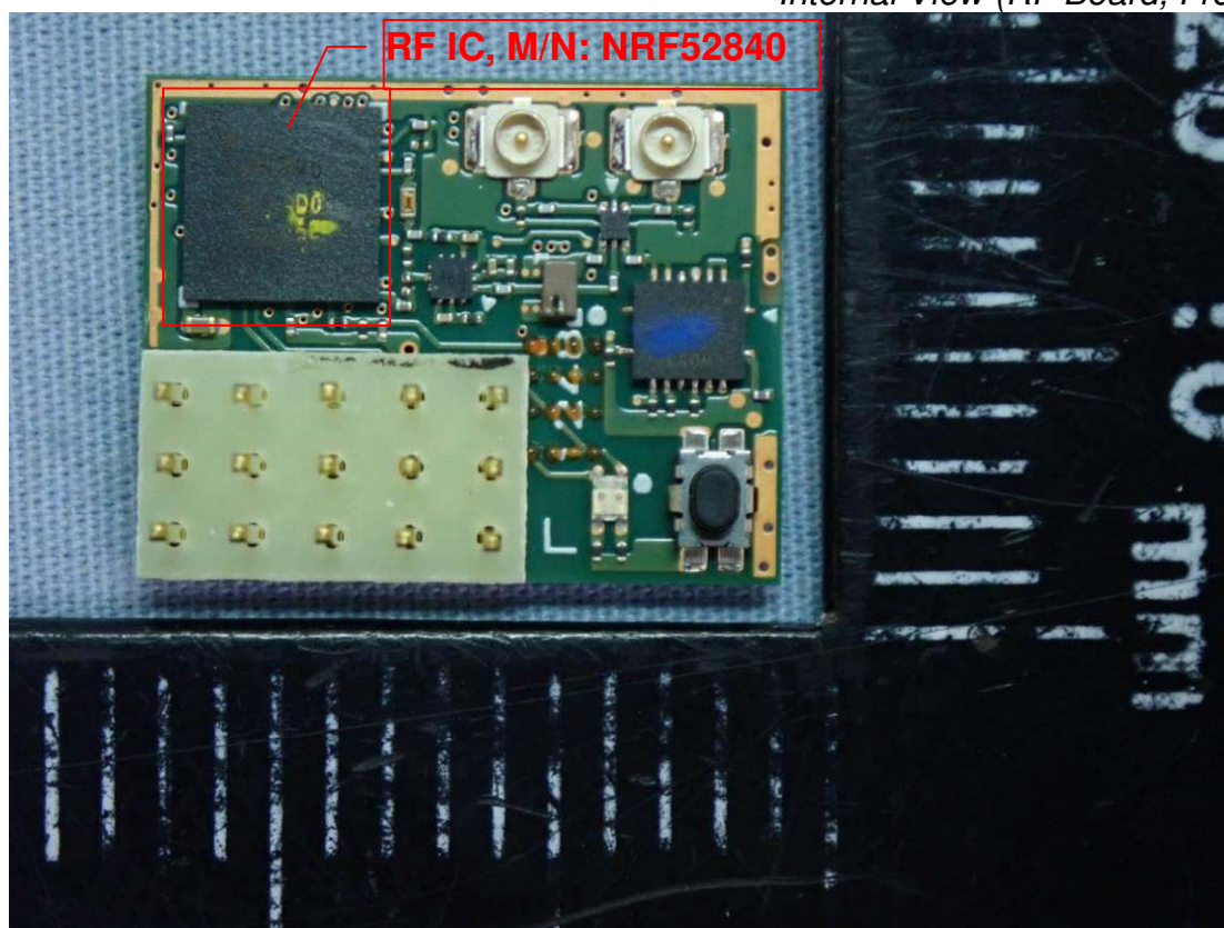
Figure 22 Internal View (RF Board, Front View)
