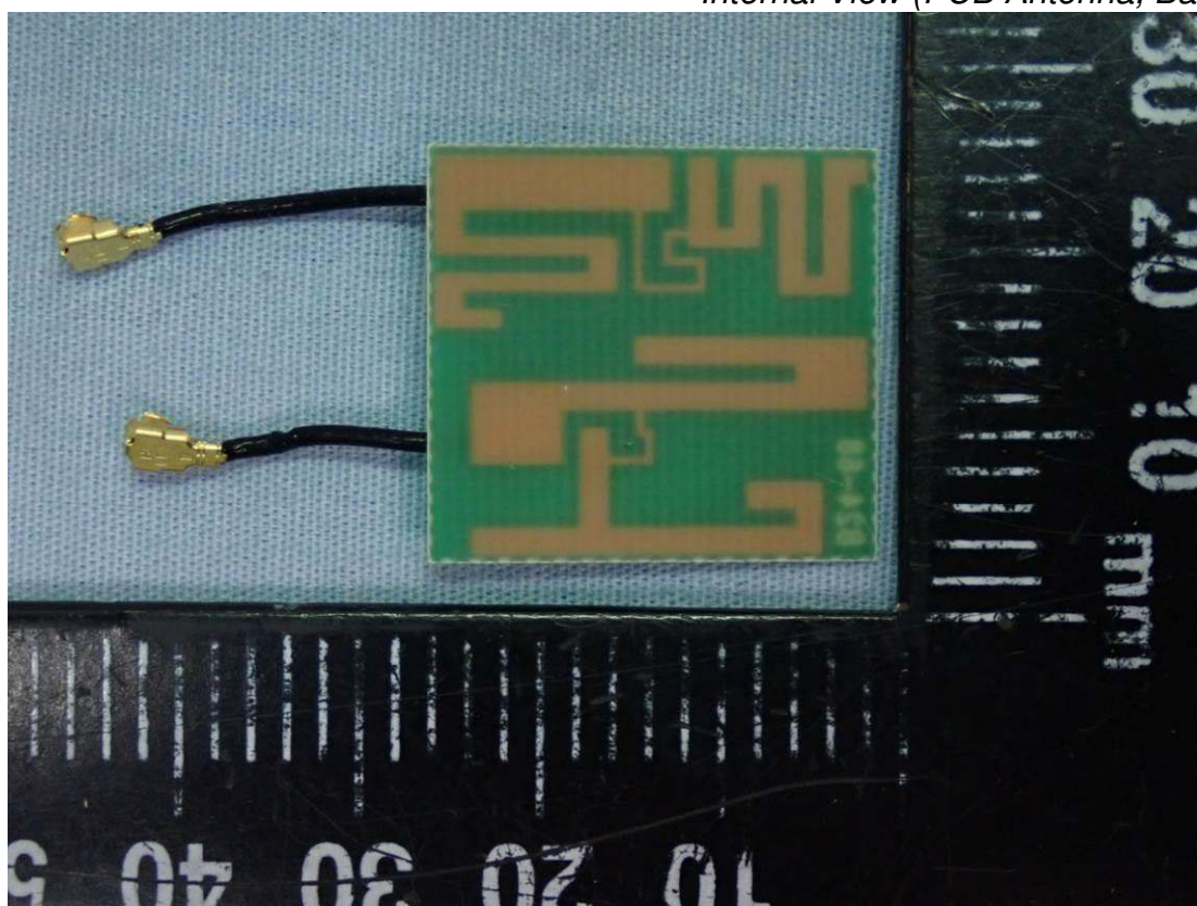
Figure 25 Internal View (PCB Antenna, Back View)
