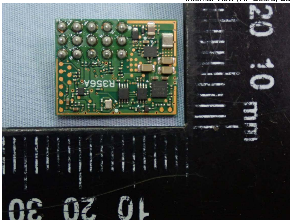
Figure 23 Internal View (RF Board, Back View)
