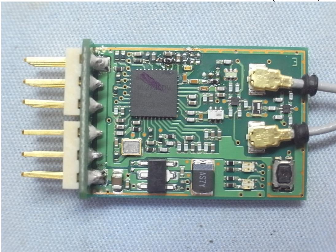
Figure 4 Internal View (RF Board, Front View)
