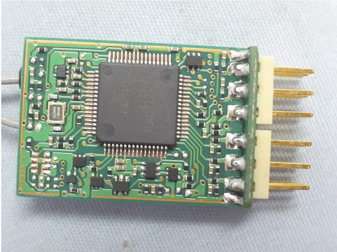
Figure 5 Internal View (RF Board, Back View)
