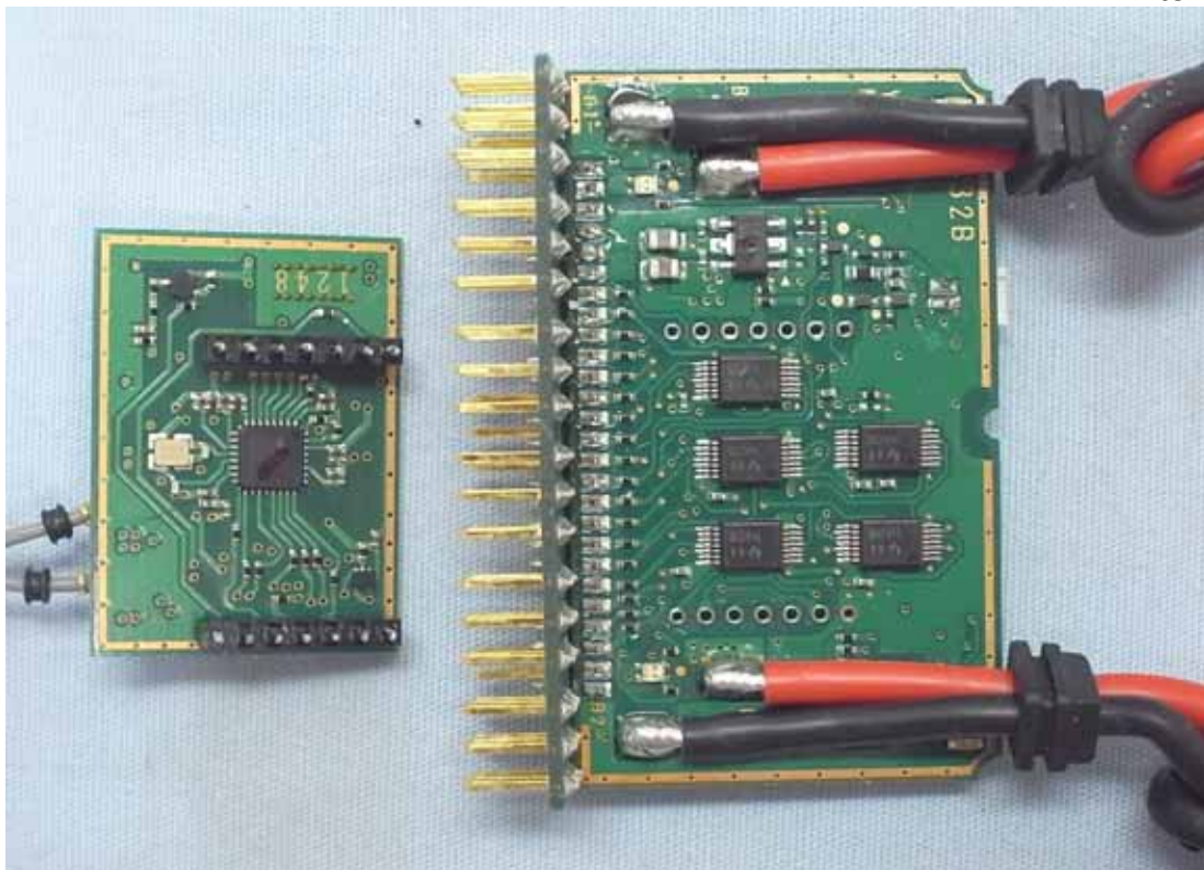
Figure 4 Internal View
