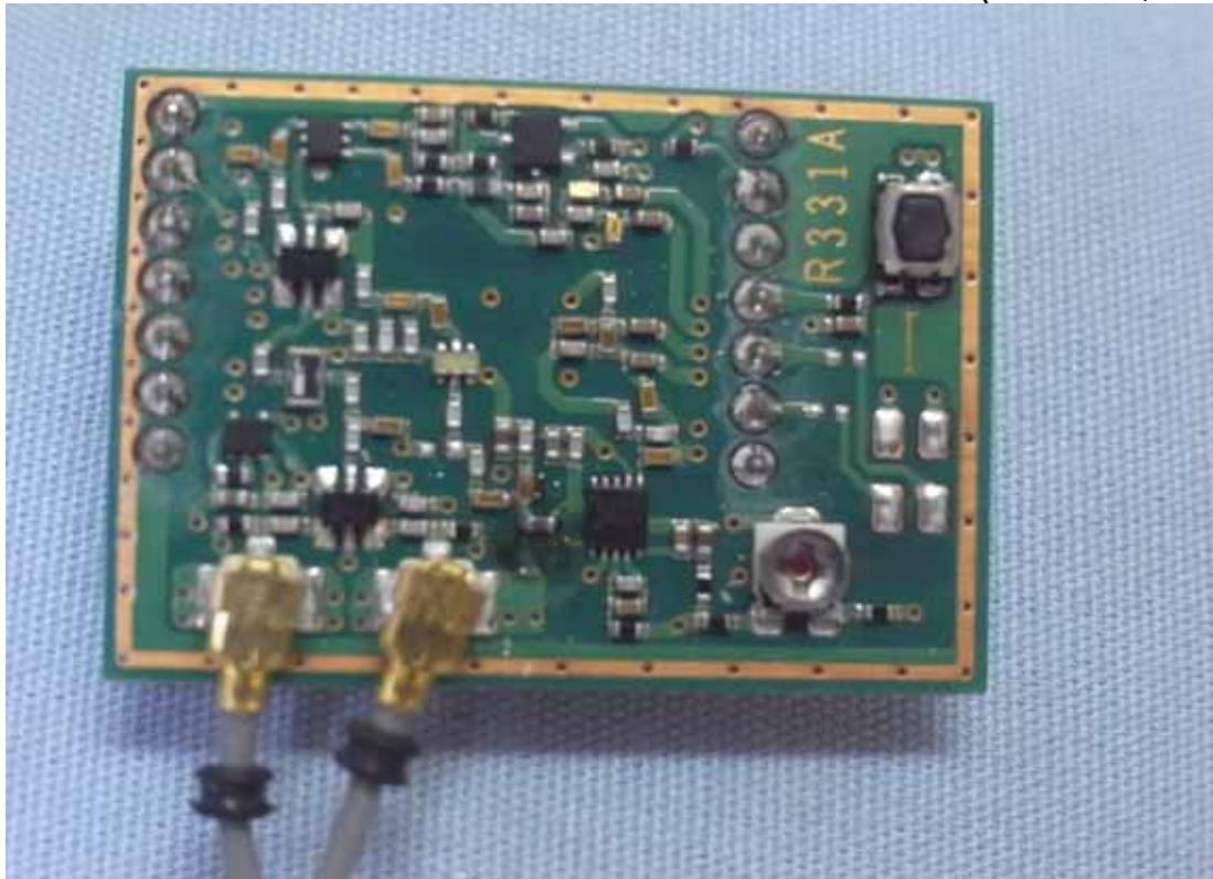
Figure 6 Internal View (RF Board, Back View)
