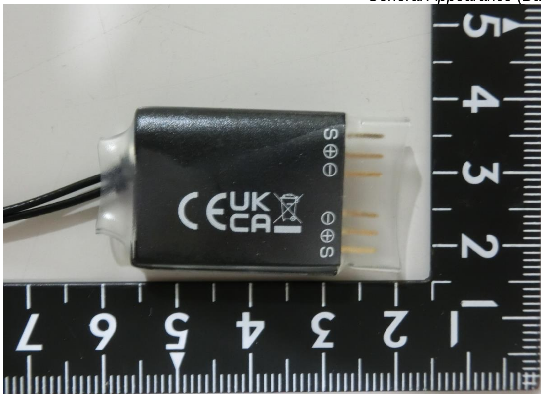
Figure 10 General Appearance (Back View)
