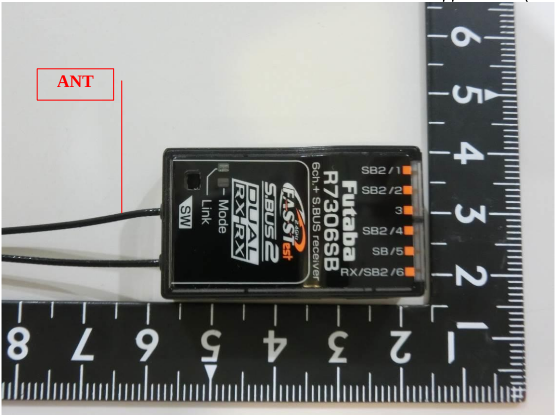
Figure 8 General Appearance (Front View)
