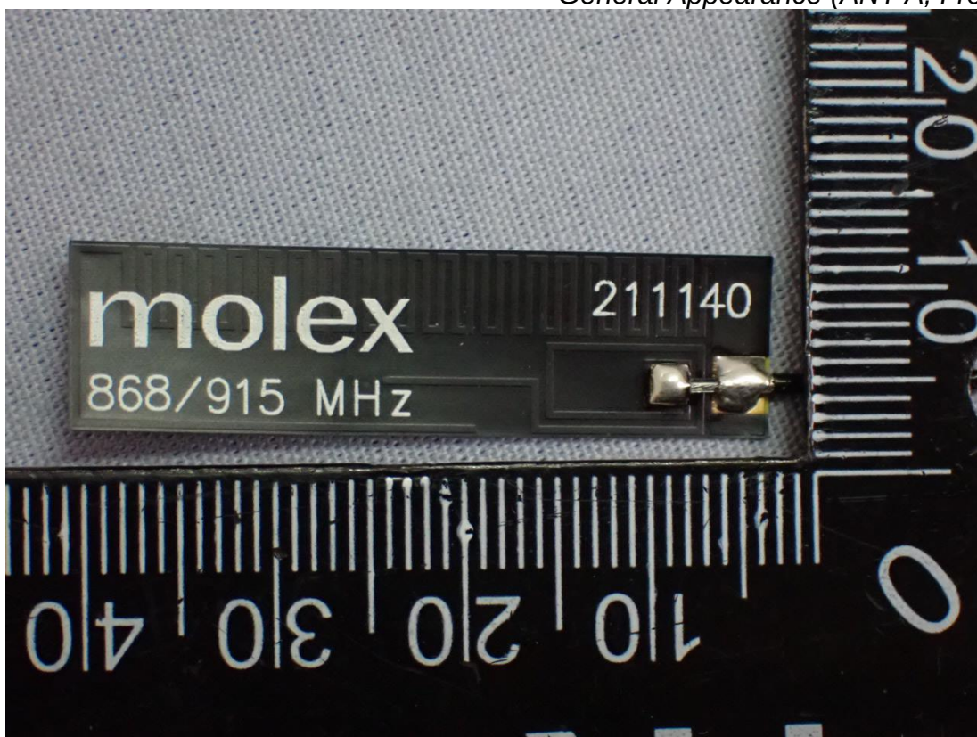
Figure 4 General Appearance (ANT A, Front View)
