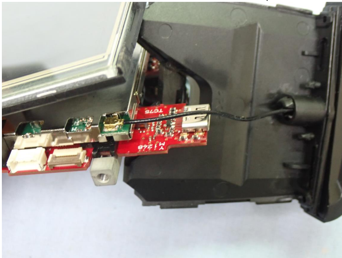
Figure 26 Internal View (Antenna Connect View)
