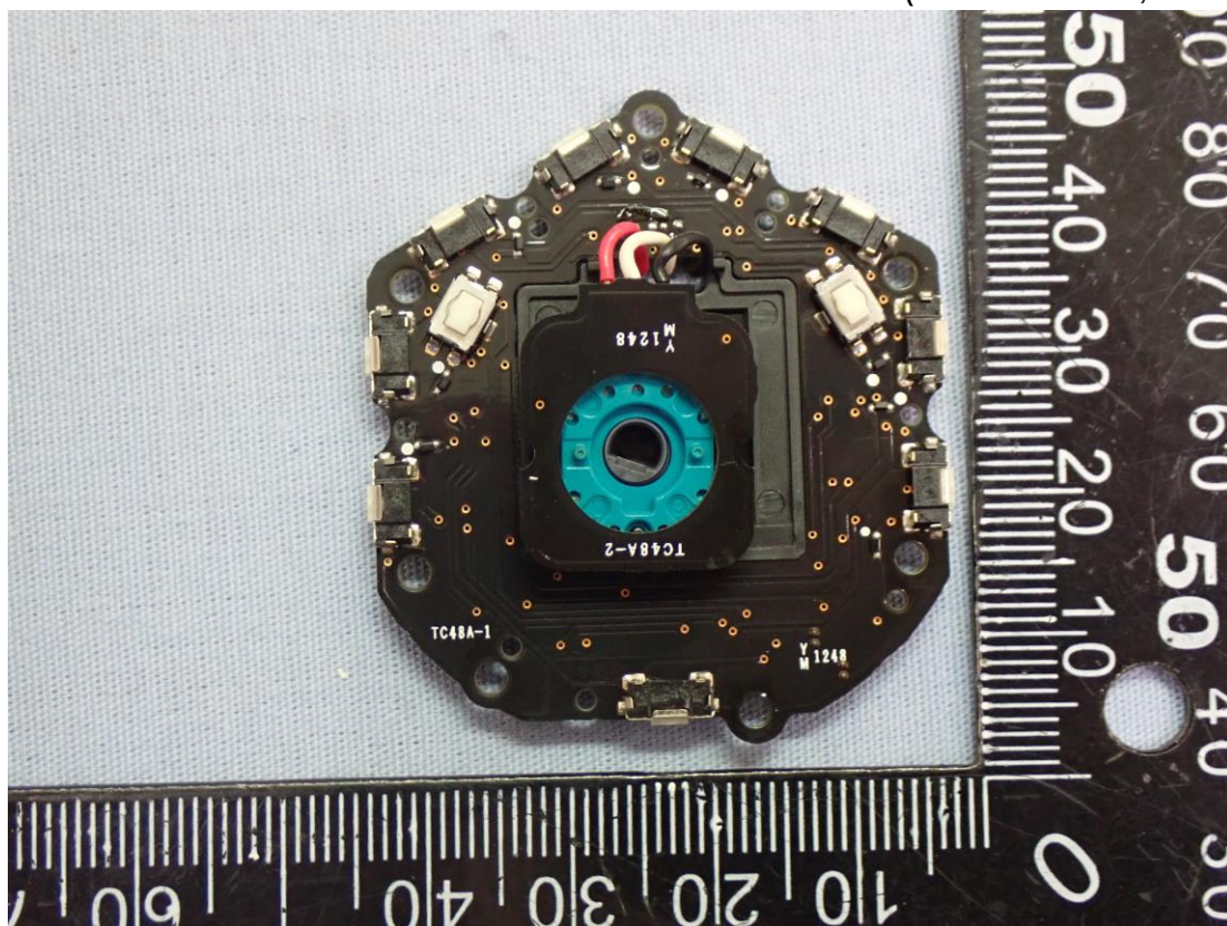
Figure 19 Internal View (Internal Board, Back View)
