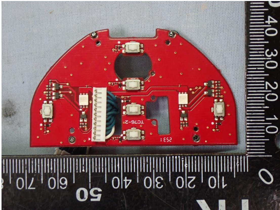
Figure 22 Internal View (Internal Board, Front View)
