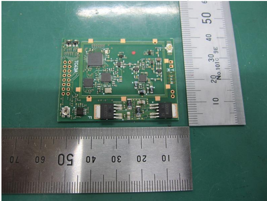
Figure 36 Internal View (Wireless Module, Front View)
