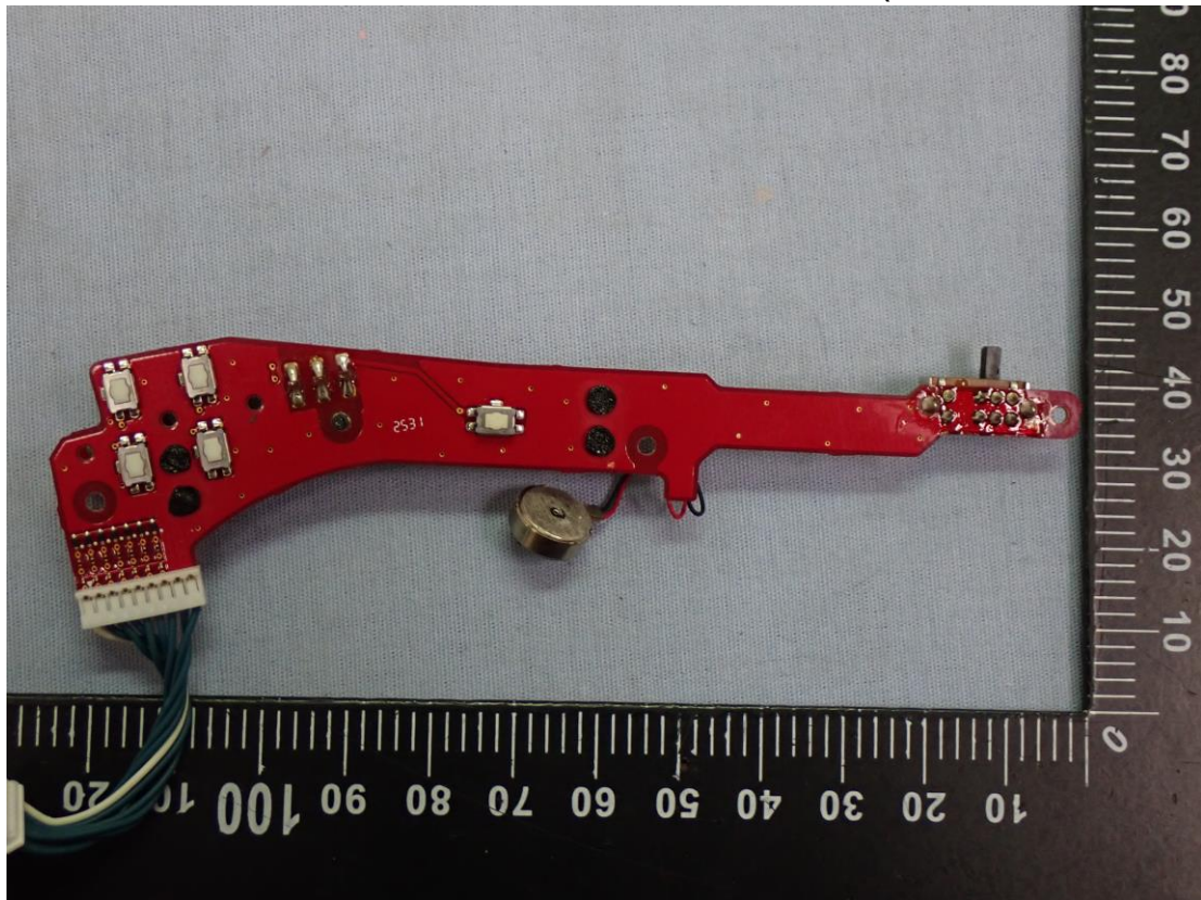
Figure 41 Internal View (Internal Board, Back View)
