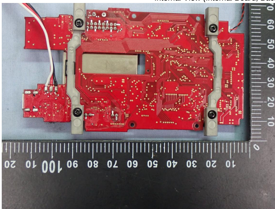
Figure 35 Internal View (Internal Board, Back View)
