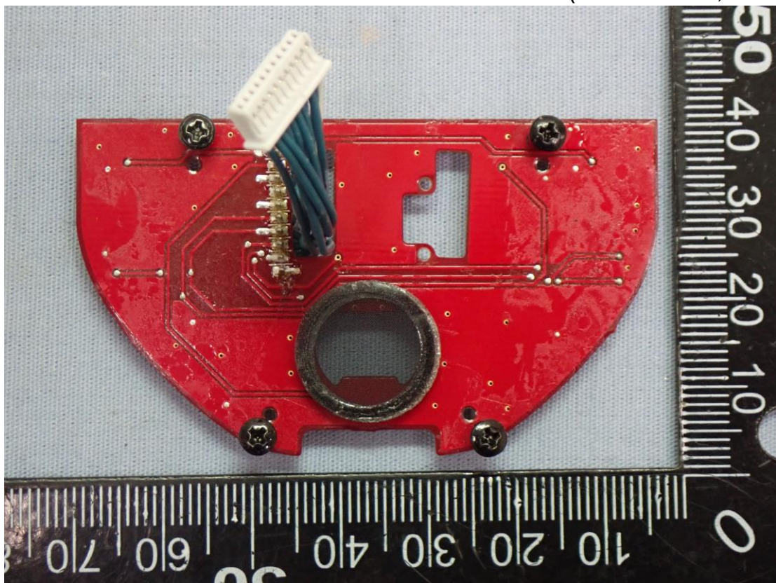
Figure 23 Internal View (Internal Board, Back View)
