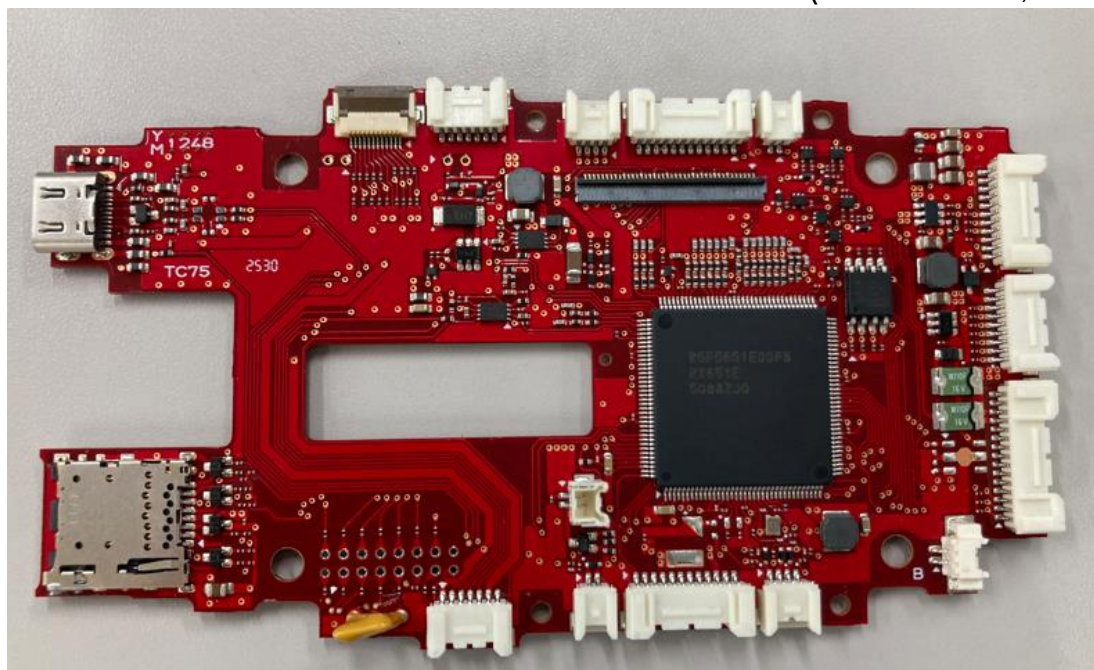
Figure 34 Internal View (Internal Board, Front View)
