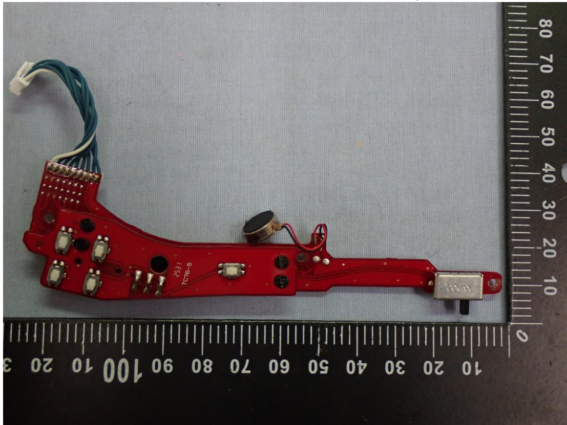
Figure 40 Internal View (Internal Board, Front View)
