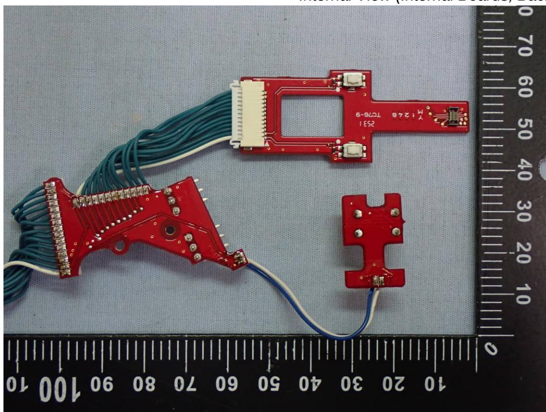
Figure 43 Internal View (Internal Boards, Back View)
