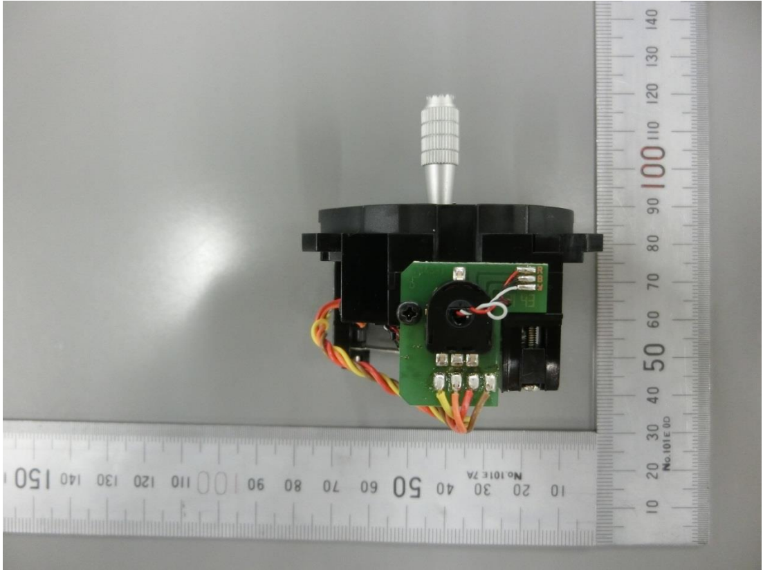
Figure 30 Internal View
