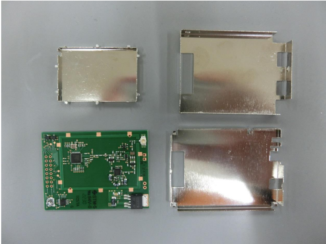
Figure 27 Wireless Module, Internal View, Front View
