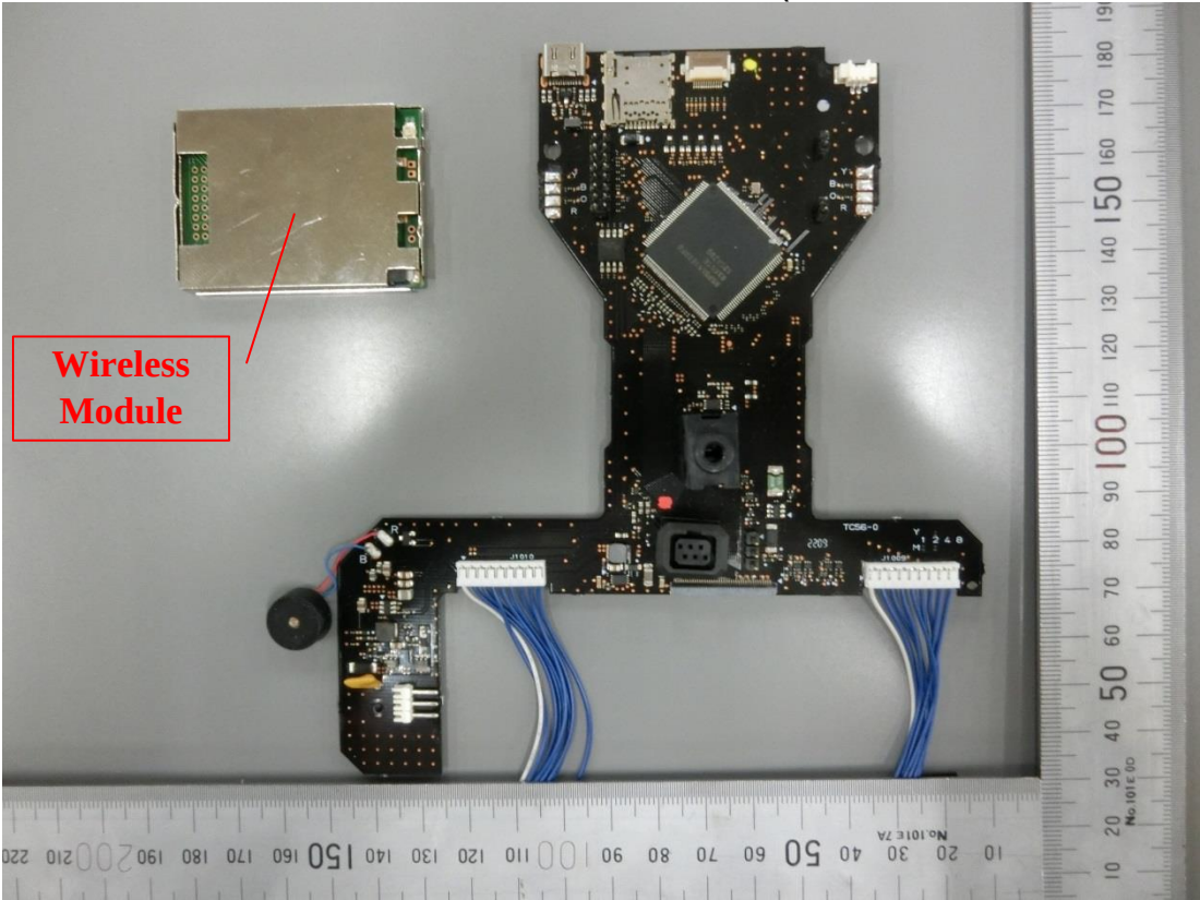
Figure 25 PCB, Front View (Removed Wireless Module)
