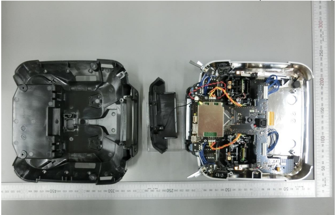
Figure 15 Internal View (Removed Cover)
