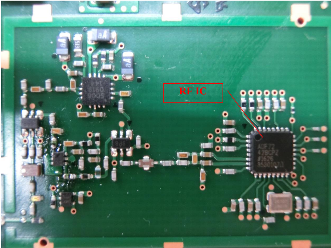
Figure 29 RF IC View
