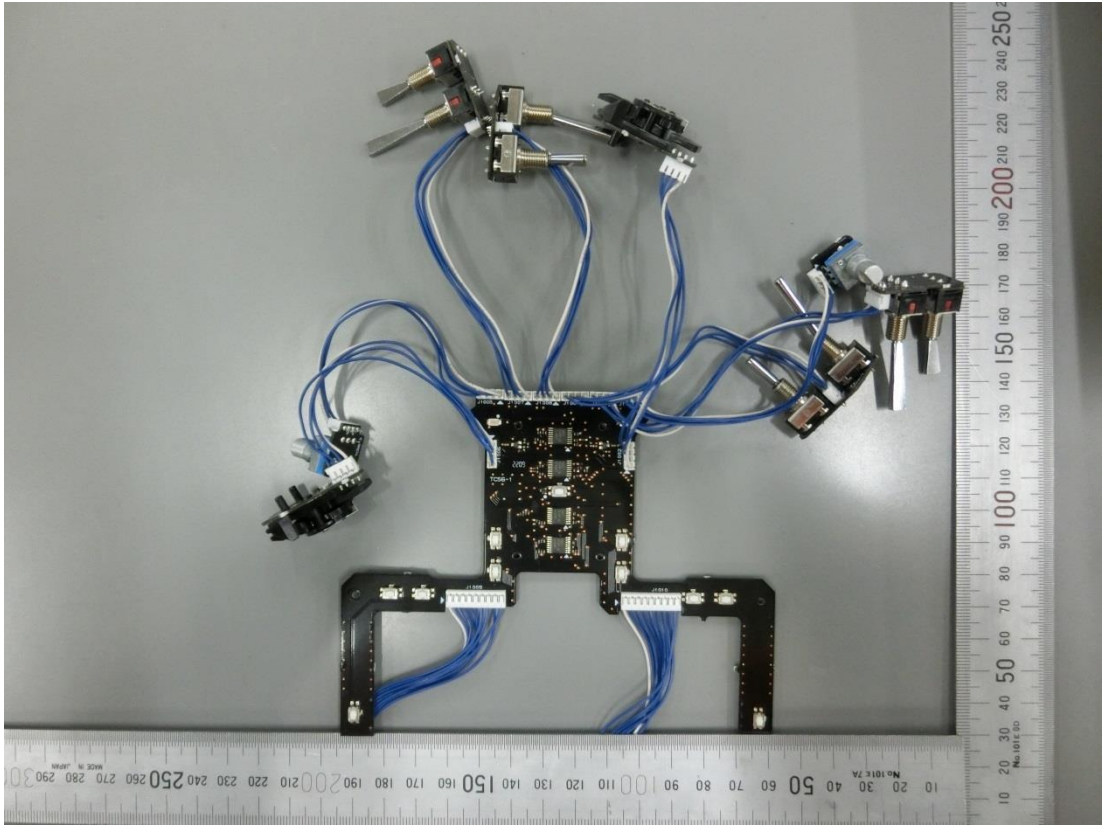
Figure 23 PCB, Front View
