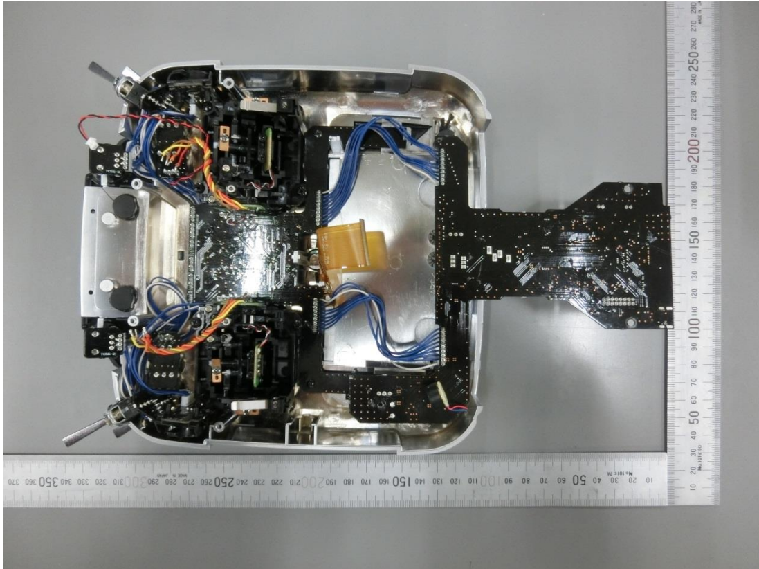
Figure 17 Internal View
