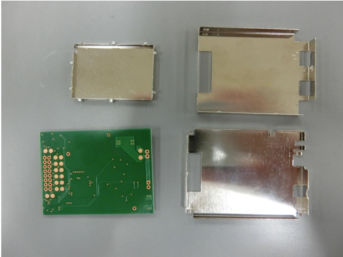
Figure 28 Wireless Module, Internal View, Back View
