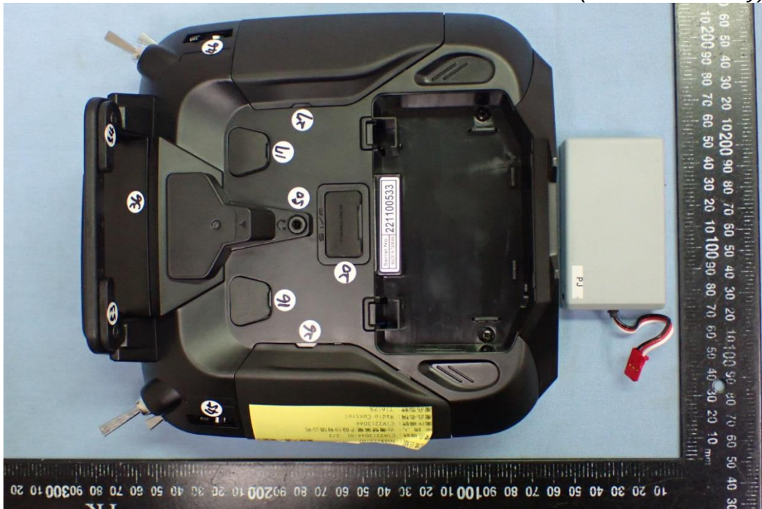
Figure 14 Internal View (Removed Battery)
