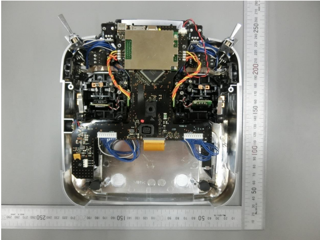
Figure 16 Internal View
