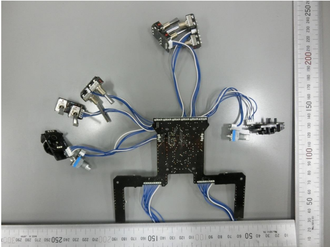
Figure 24 PCB, Back View
