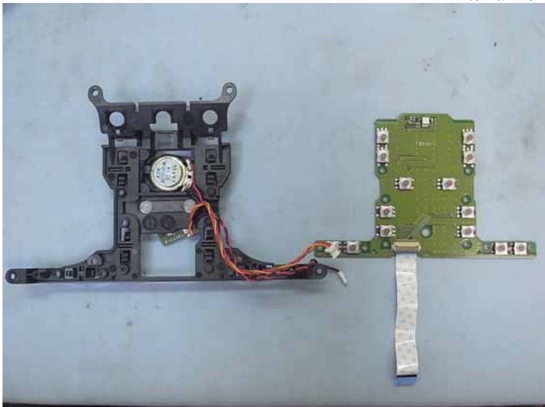
Figure 16 Internal View
