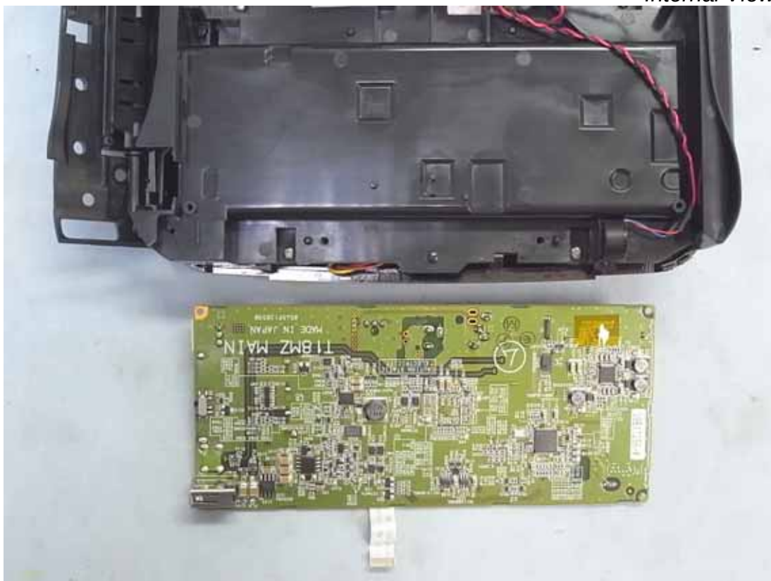
Figure 11 Internal View
