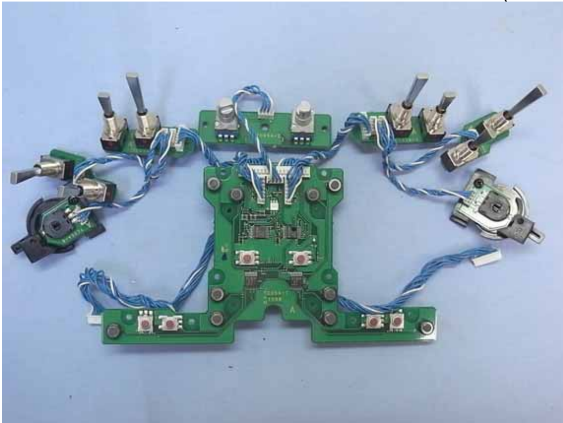
Figure 15 Internal View (Control Boards)
