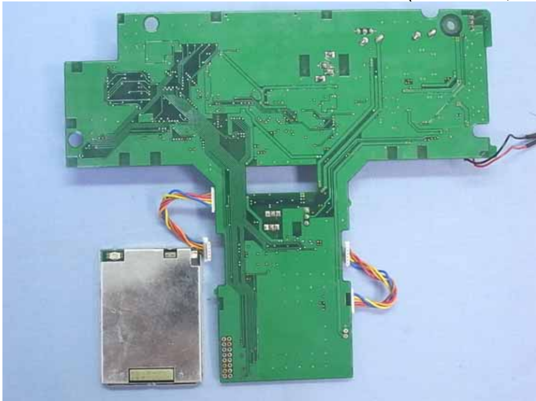
Figure 9 Internal View (TB77B Board, Back View)
