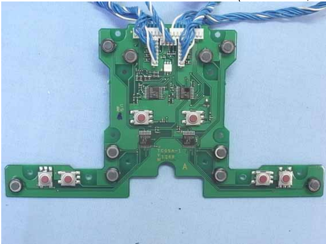
Figure 16 Internal View (TC05A-1 Board, Front View)
