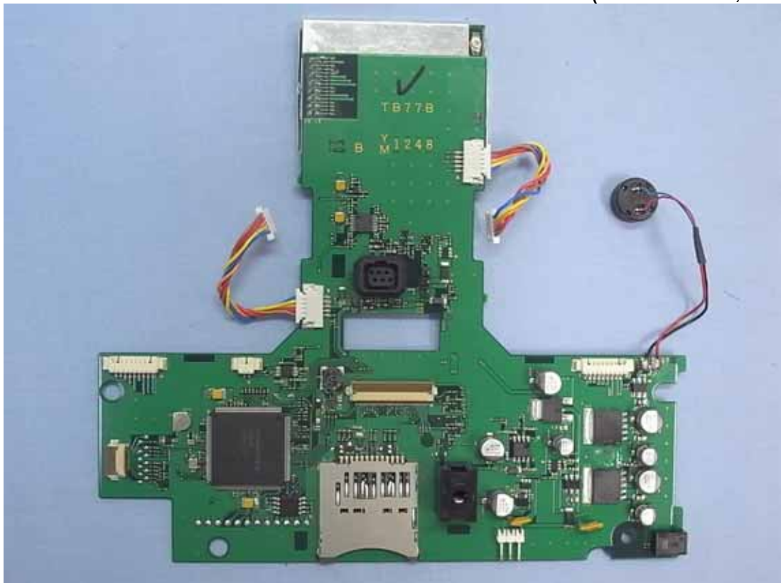
Figure 8 Internal View (TB77B Board, Front View)
