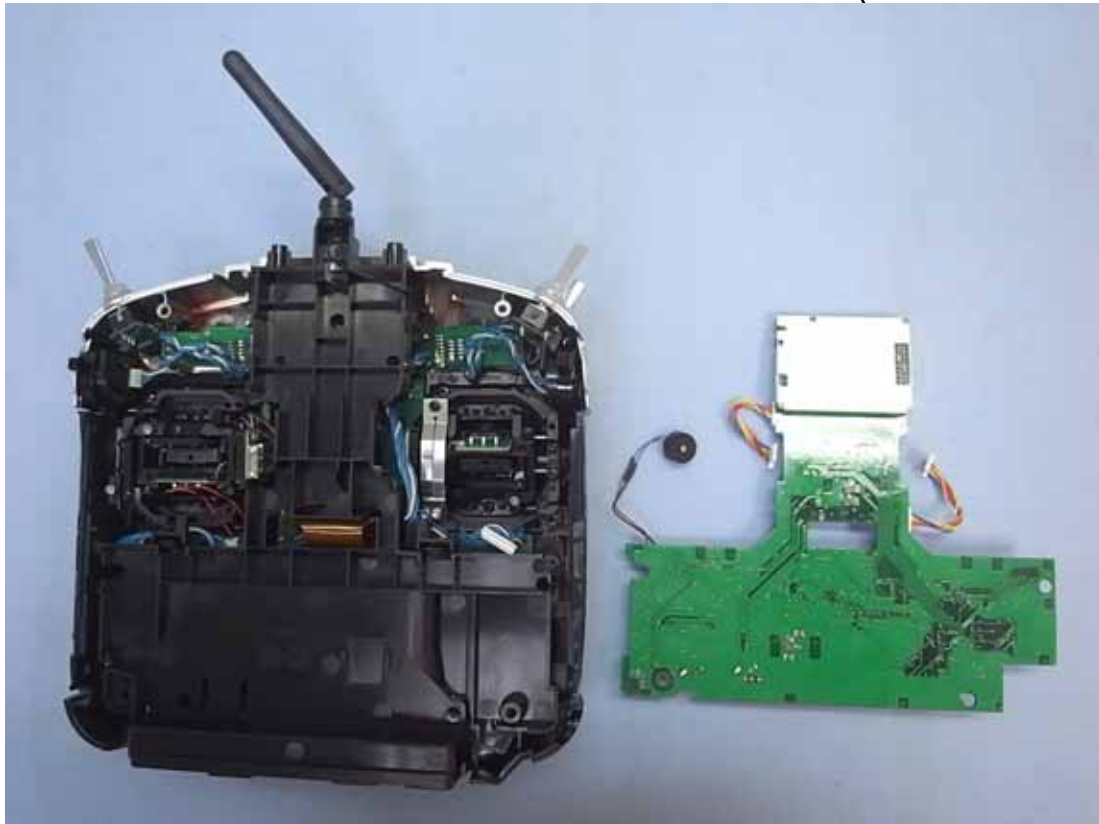
Figure 7 Internal View (Removed TB77B Board)
