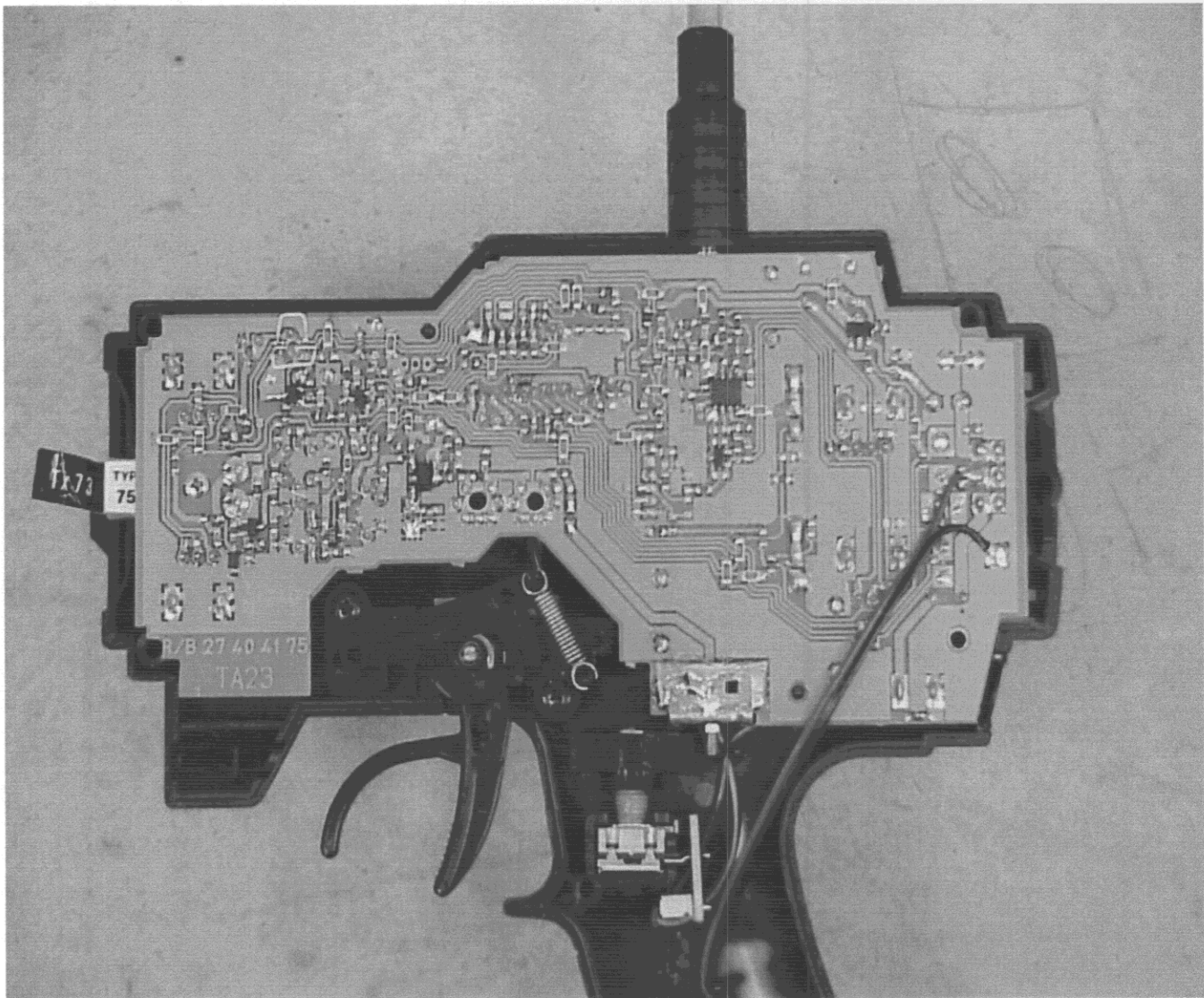
6.7 EUT with Enclosure Removed
