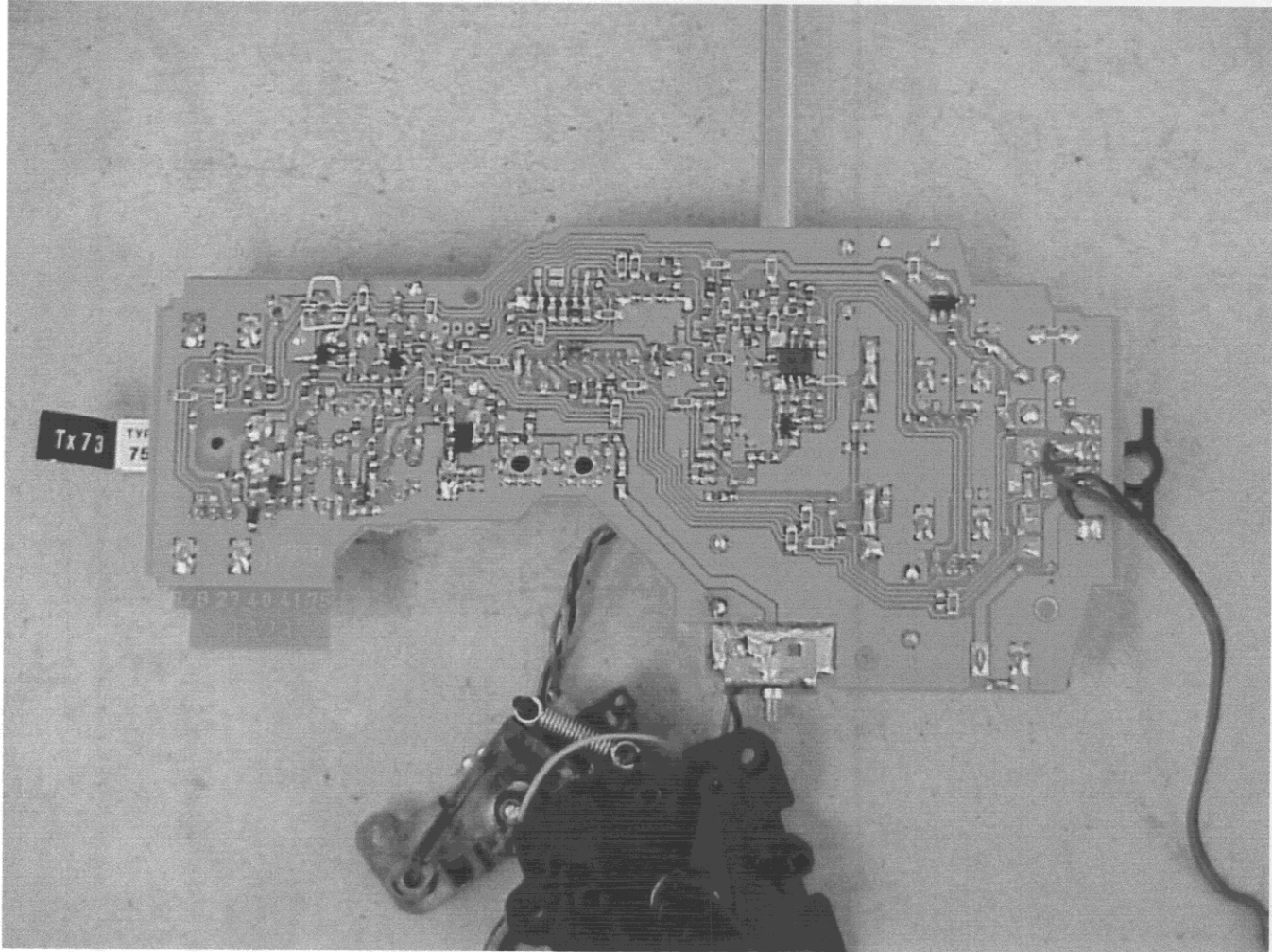
6.9 EUT PCB Layout & Components (2)
