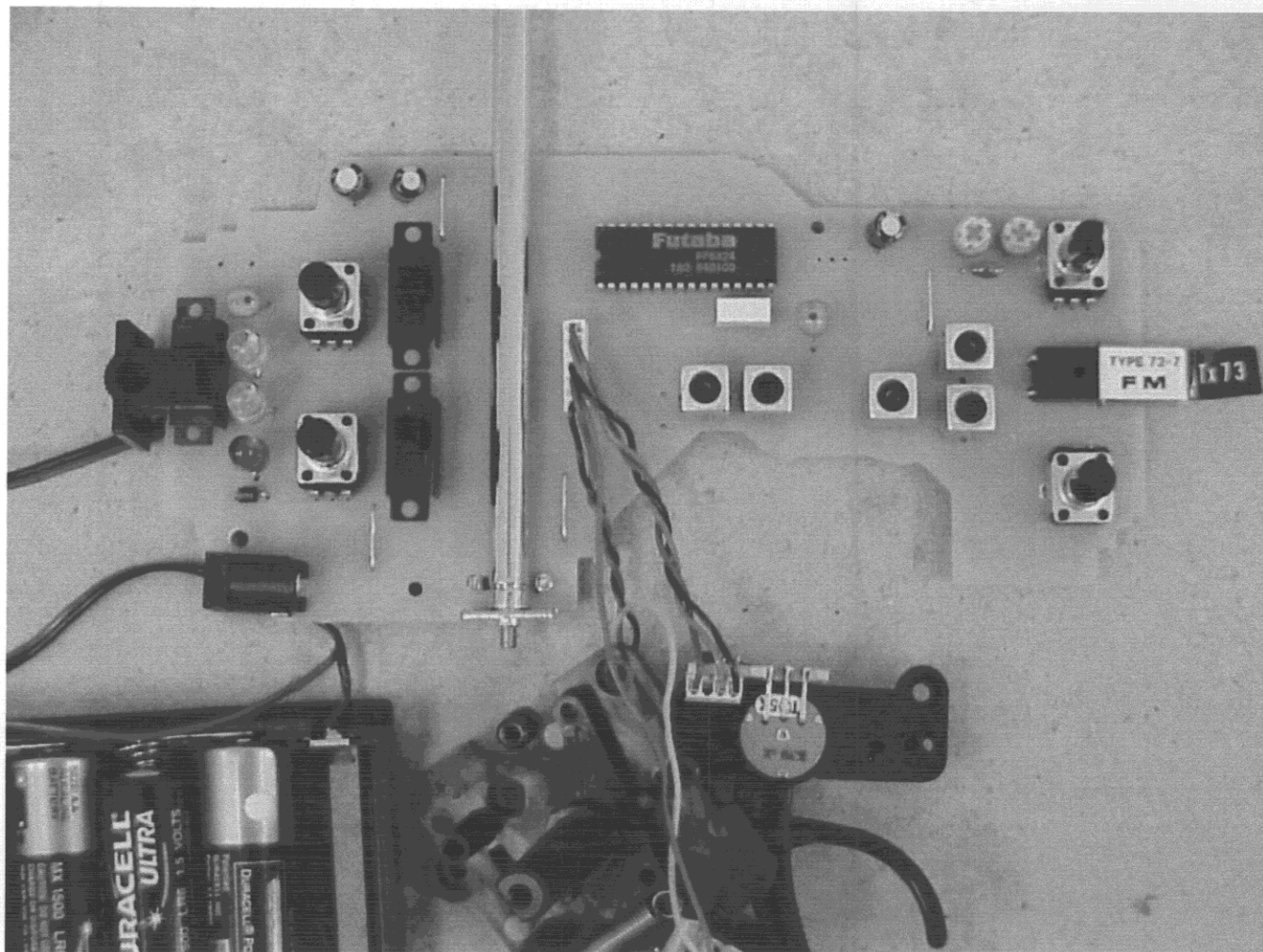
6.8 EUT PCB Layout & Components (1)
