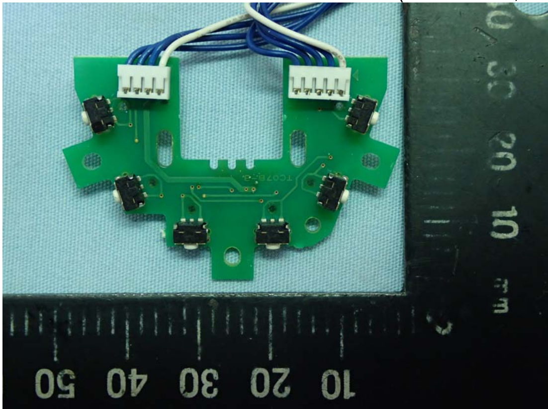
Figure 12 Internal View (TC07B-3 Board, Front View)
