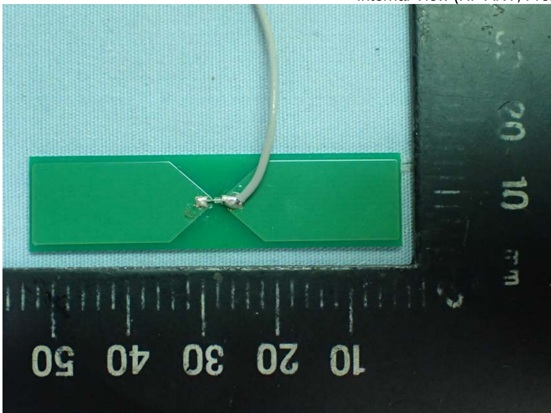
Figure 10 Internal View (RF ANT, Front View)
