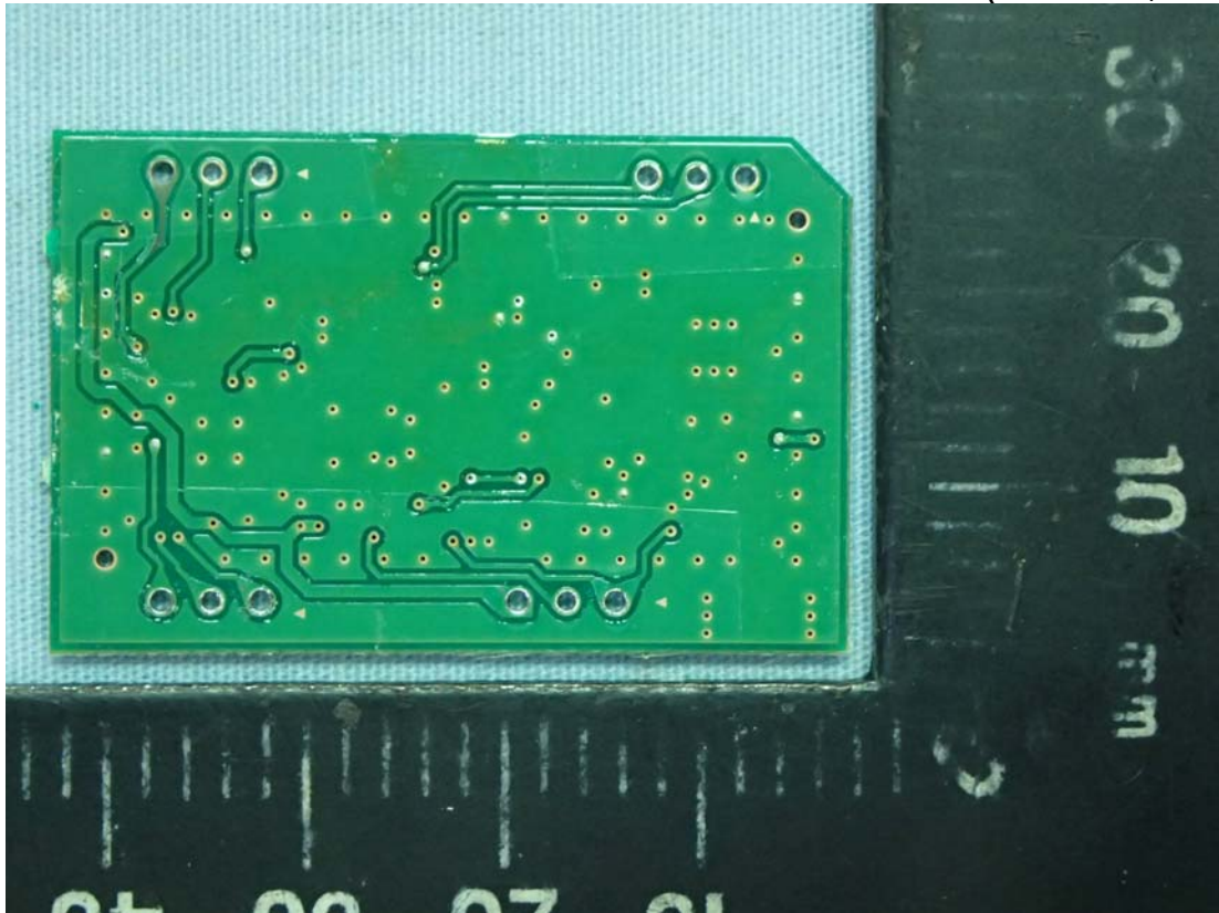
Figure 17 Internal View (RF Board, Back View)
