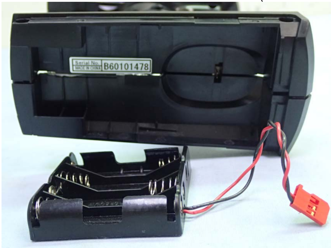
Figure 6 Internal View (Removed Battery Case)
