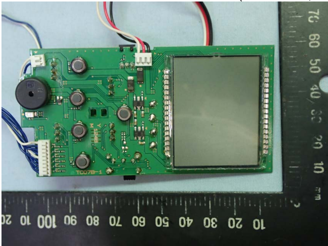
Figure 14 Internal View (TC07B-1 Board, Front View)
