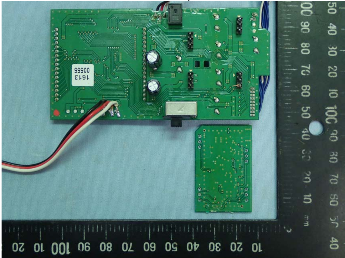
Figure 15 Internal View (TC07B-1 Board, Back View and RF Board)
