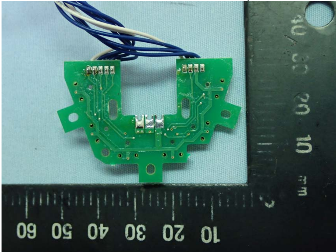
Figure 13 Internal View (TC07B-3 Board, Back View)
