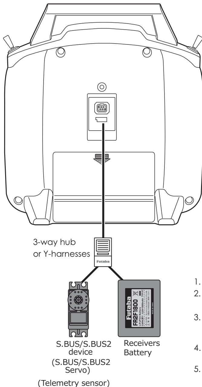
Back of T6K
