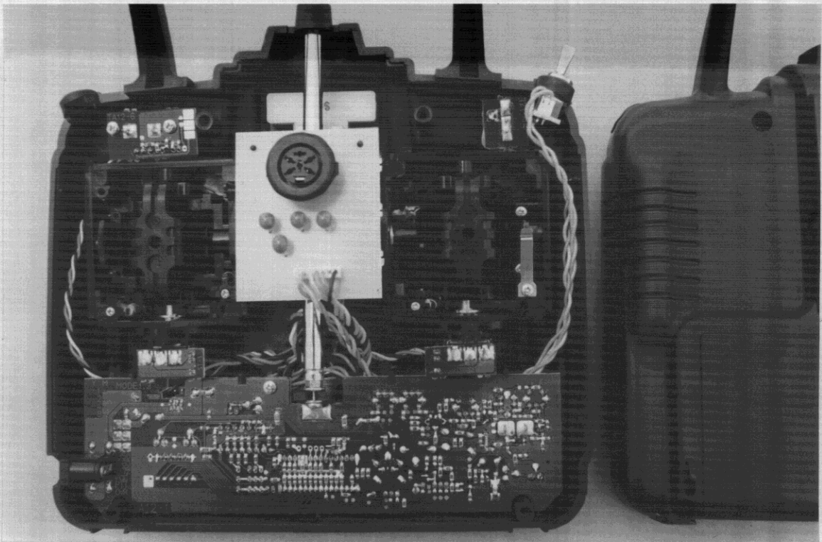
5.6 Photo: EUT with cover removed
