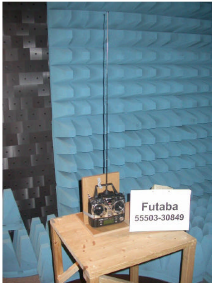
Test setup unwanted radiation 30 MHz - 1 GHz
