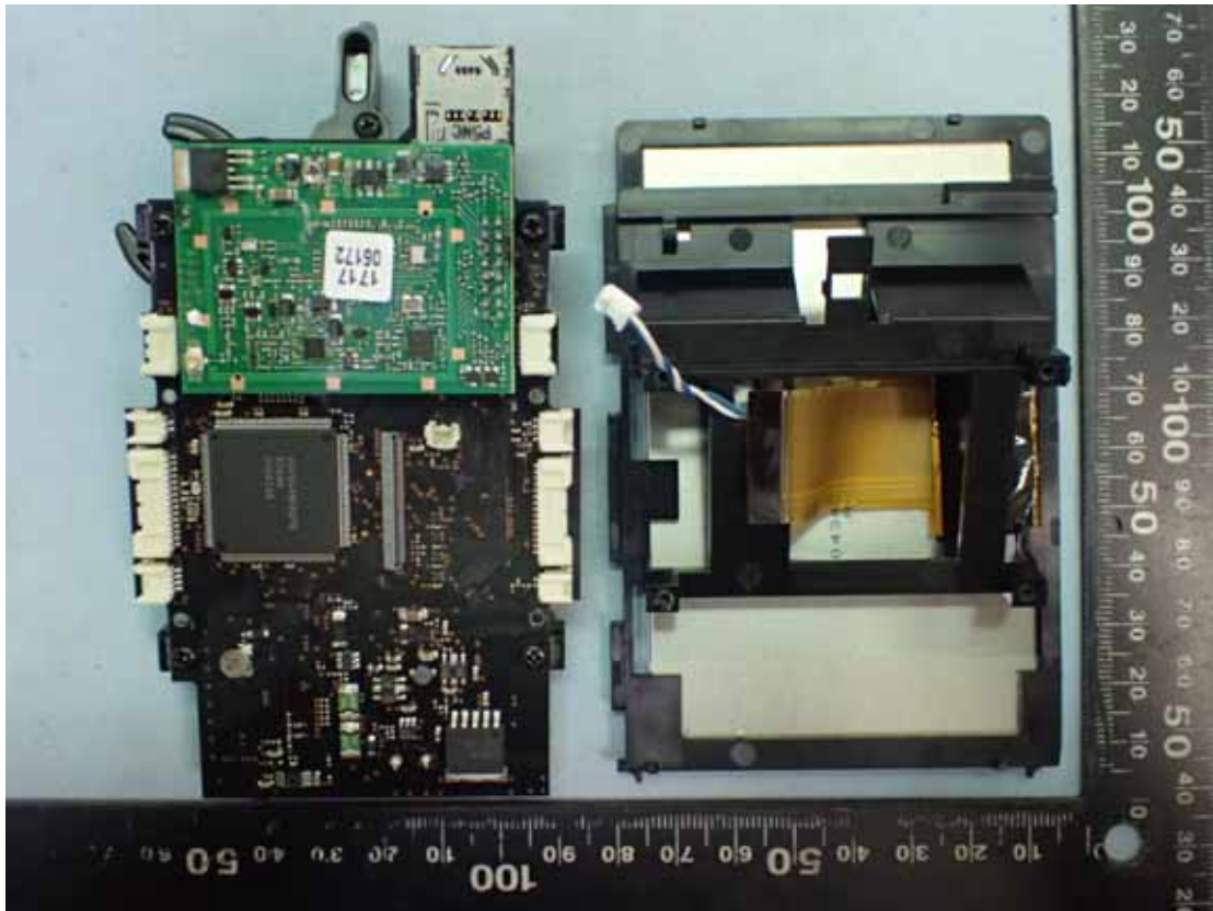
Figure 36 Internal View
