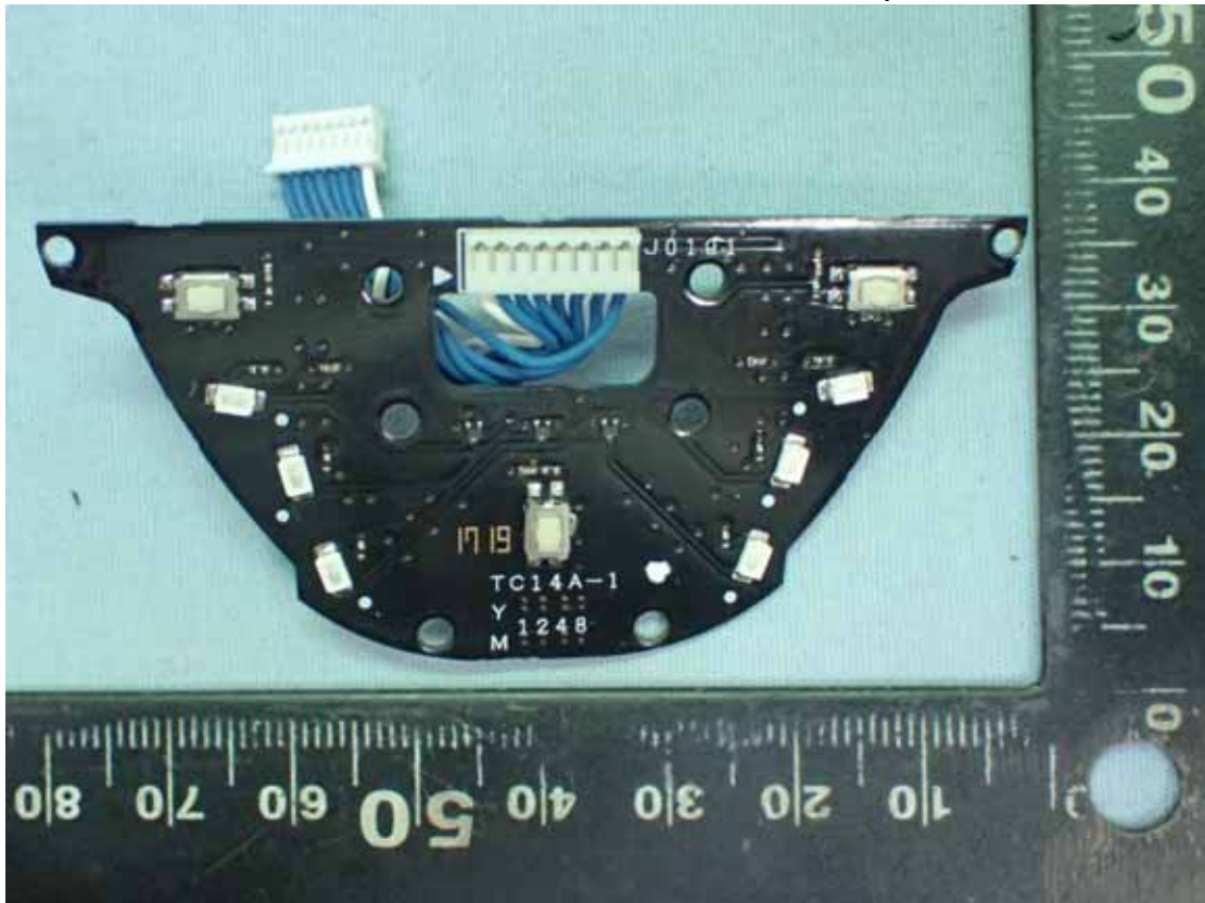
Figure 34 Internal View (Control Board, Front View)
