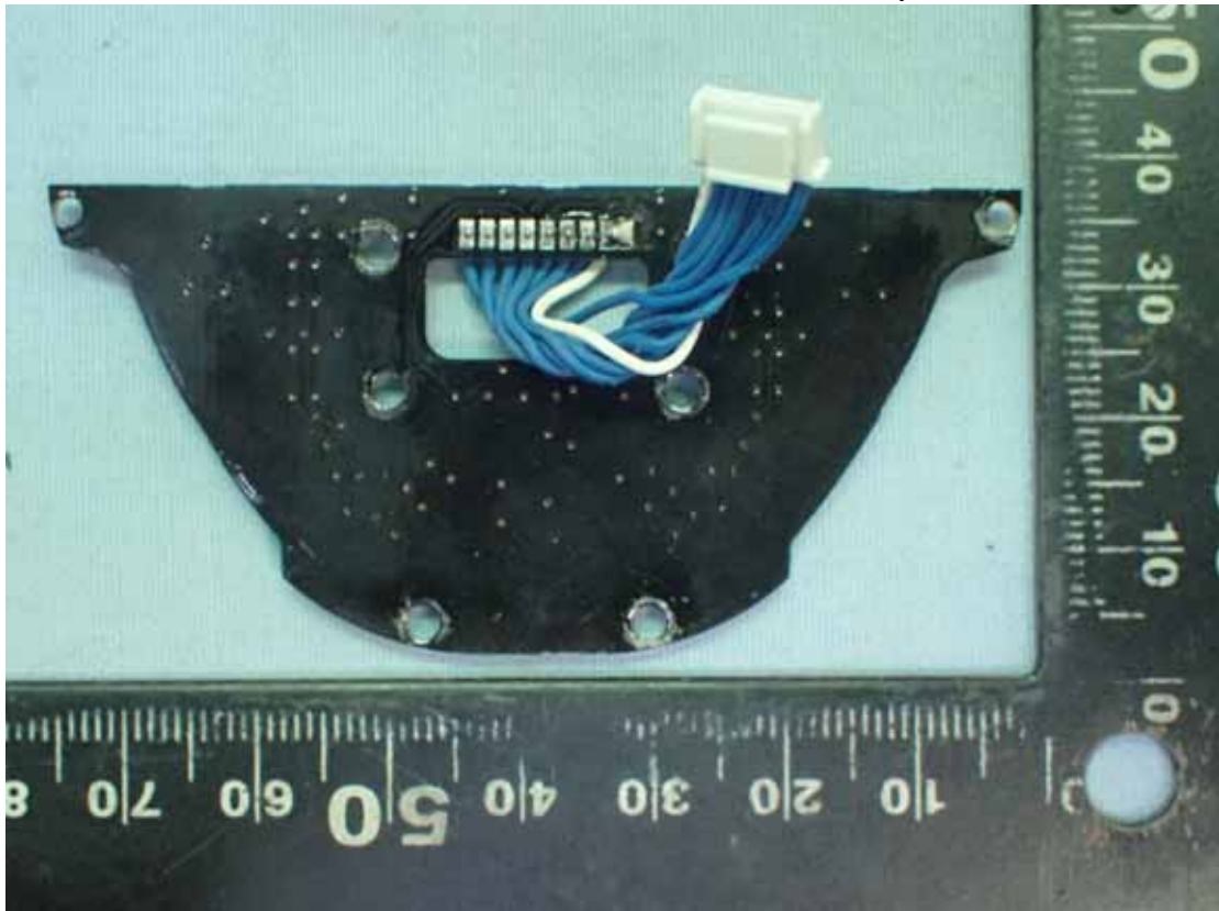
Figure 35 Internal View (Control Board, Back View)
