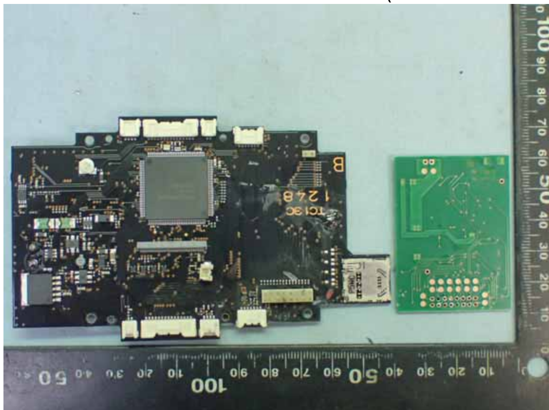
Figure 41 Internal View (Removed RF Control Board)
