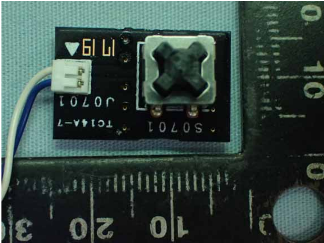
Figure 14 Internal View (Front View)
