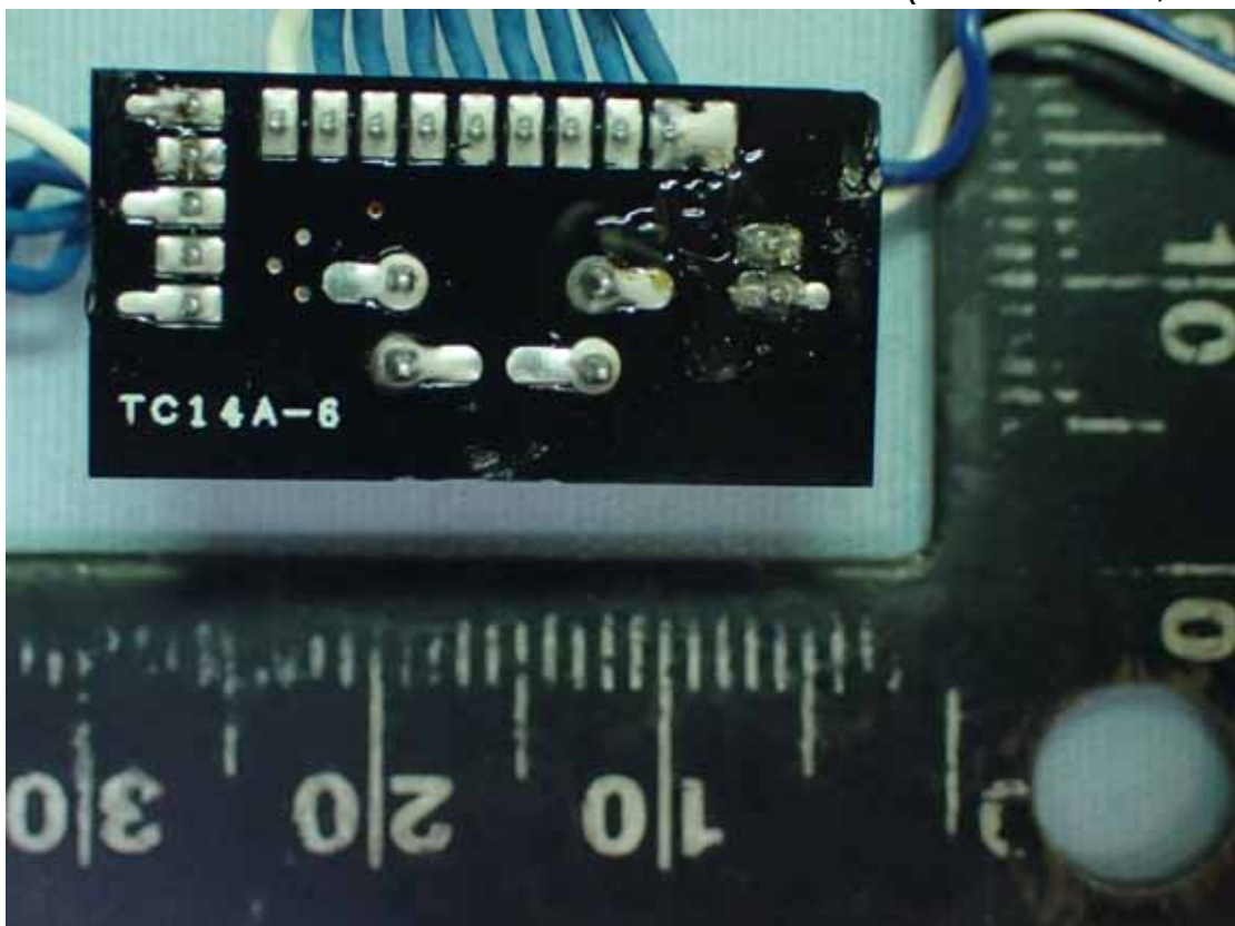
Figure 15 Internal View (Control Board, Back View)
