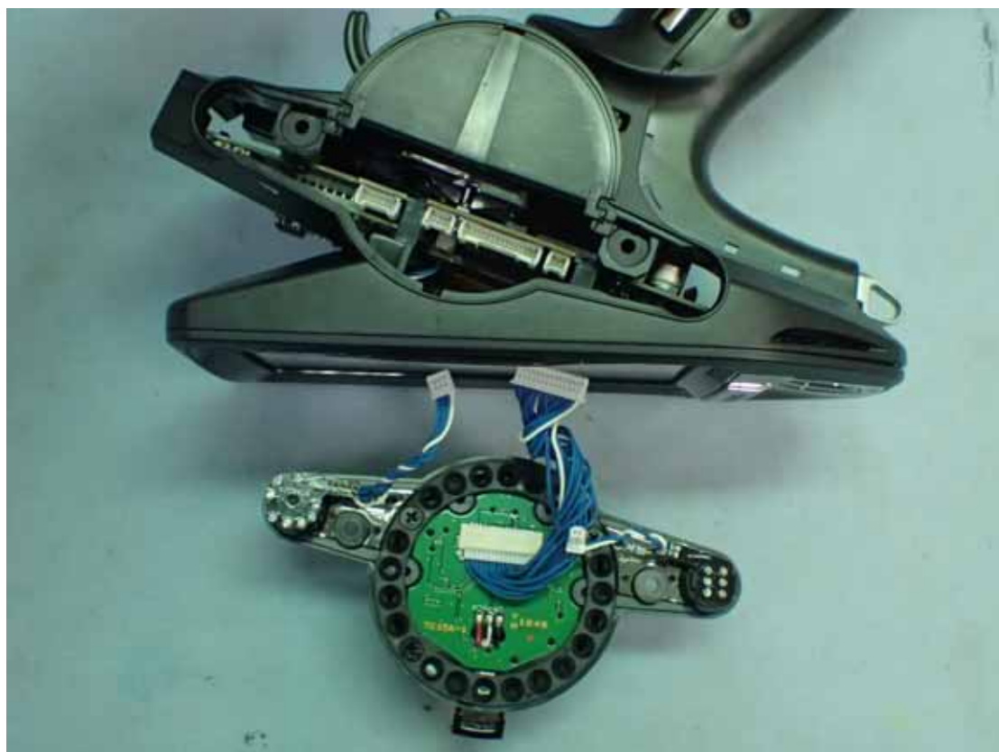
Figure 27 Internal View
