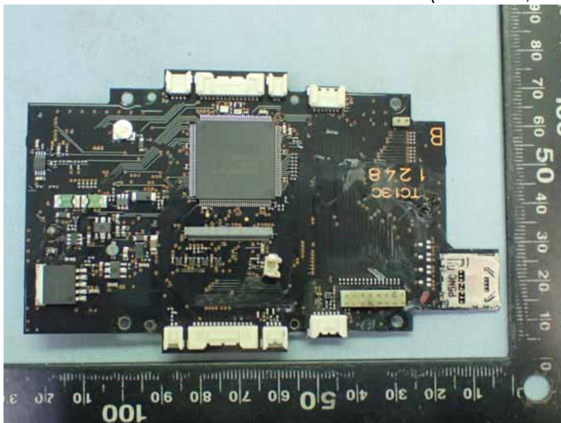
Figure 42 Internal View (Main Board, Front View)
