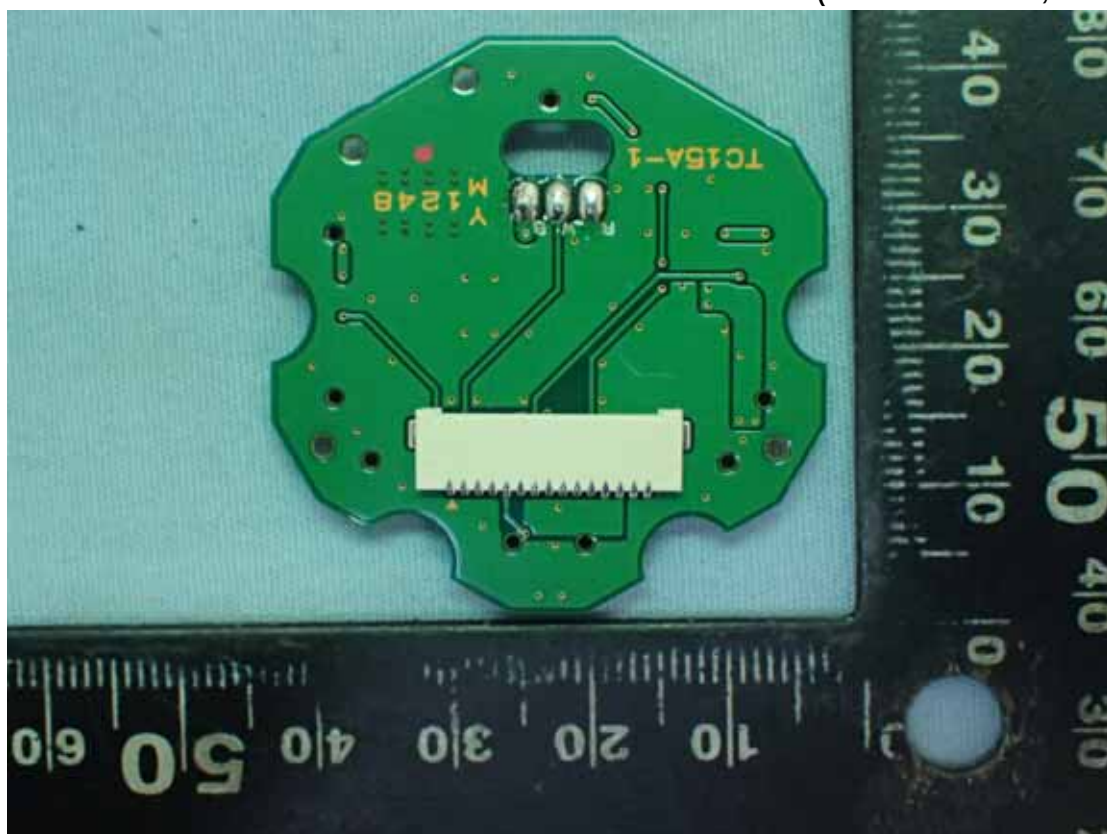
Figure 29 Internal View (Control Board, Back View)
