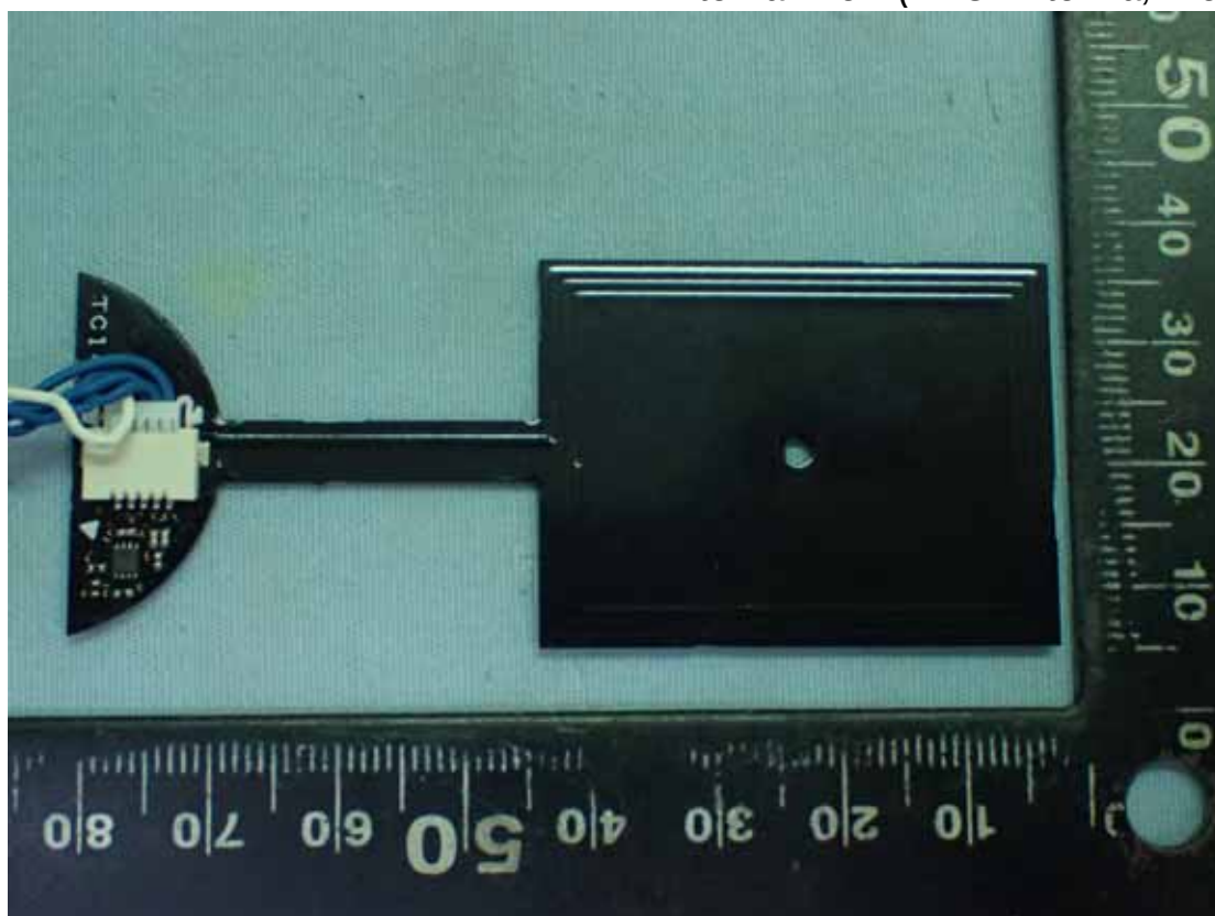
Figure 17 Internal View (NFC Antenna, Front View)
