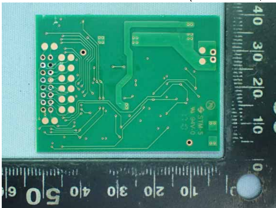
Figure 43 Internal View (RF Control Board, Back View)
