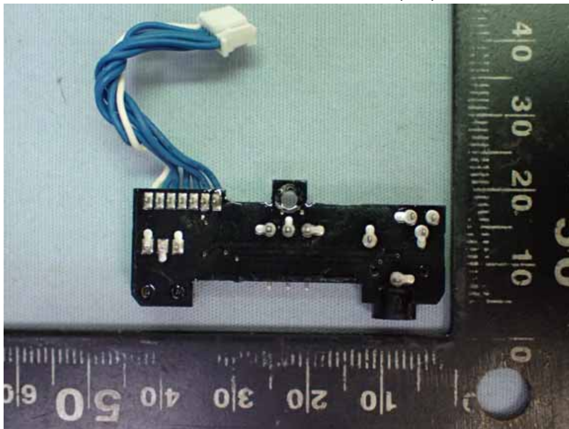
Figure 10 Internal View (Earphone Board, Back View)
