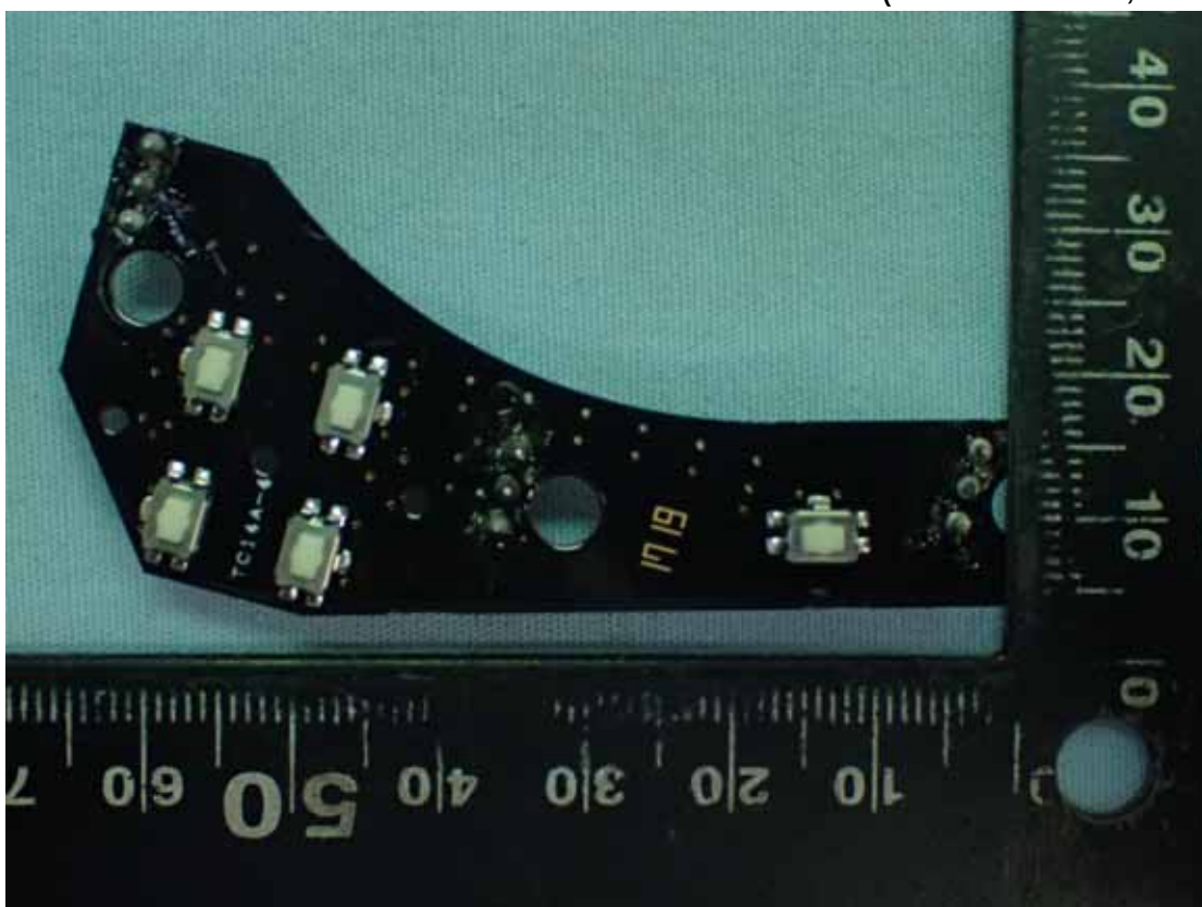
Figure 23 Internal View (Control Board, Front View)
