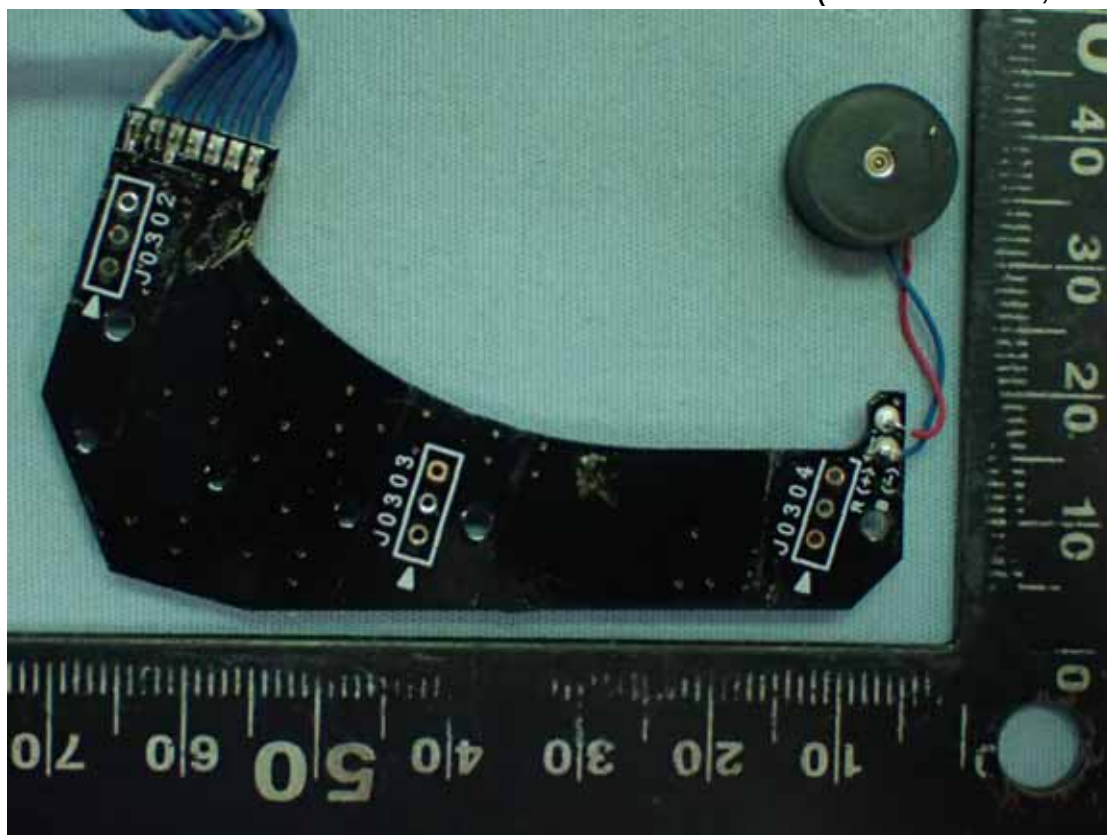
Figure 26 Internal View (Control Board, Back View)
