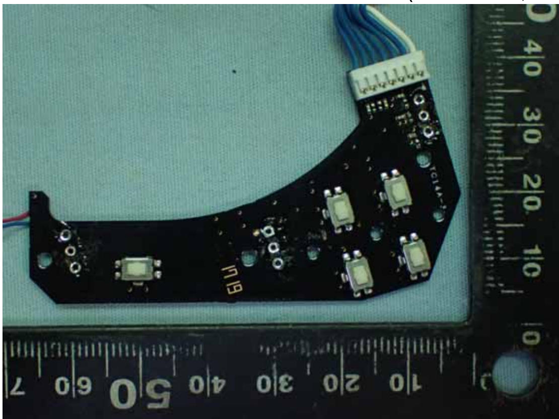
Figure 25 Internal View (Control Board, Front View)
