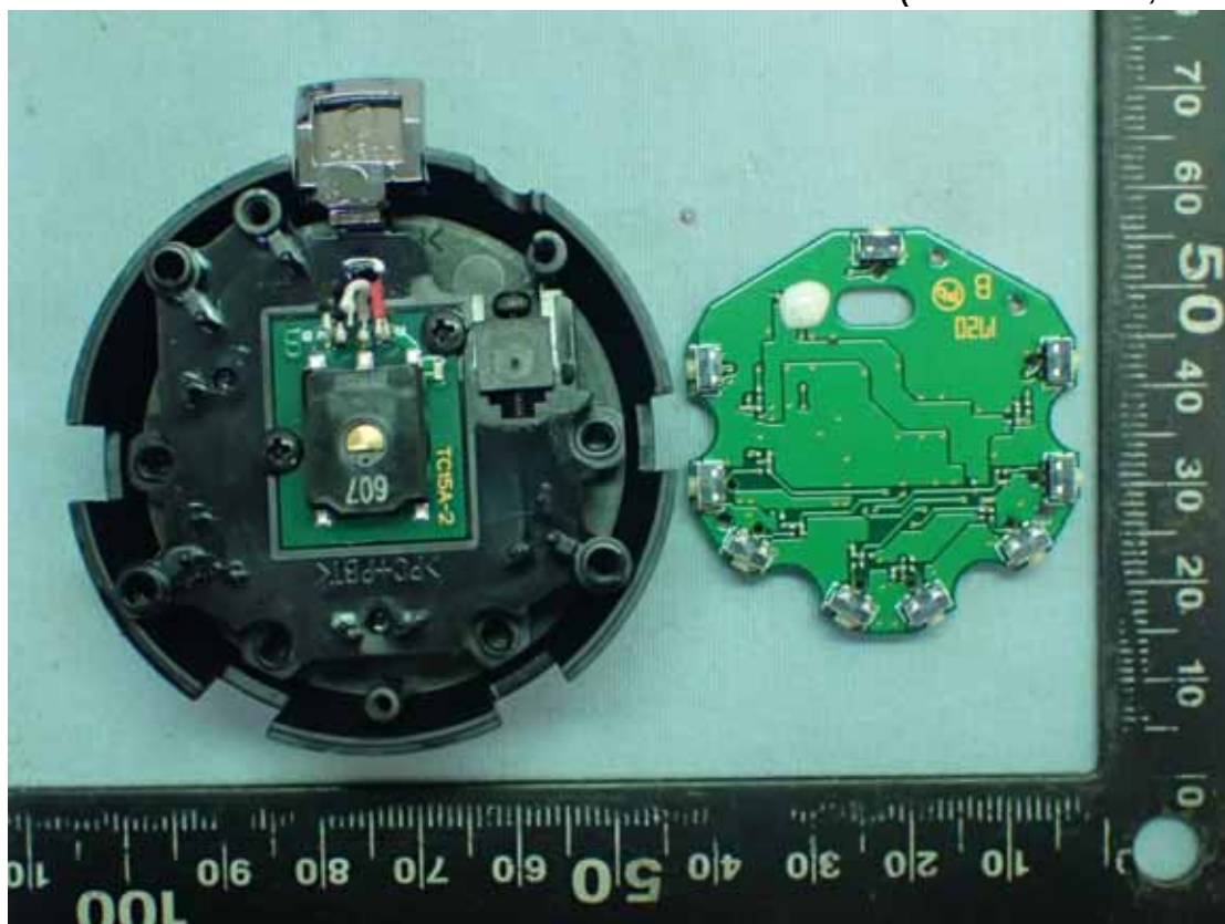
Figure 28 Internal View (Control Board, Front View)
