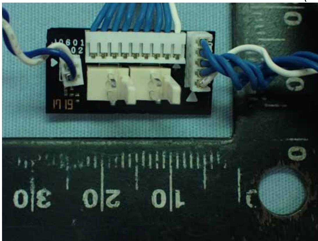
Figure 16 Internal View (Front View)
