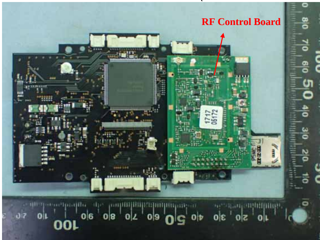
Figure 40 Internal View (Main Board and RF Control Board)
