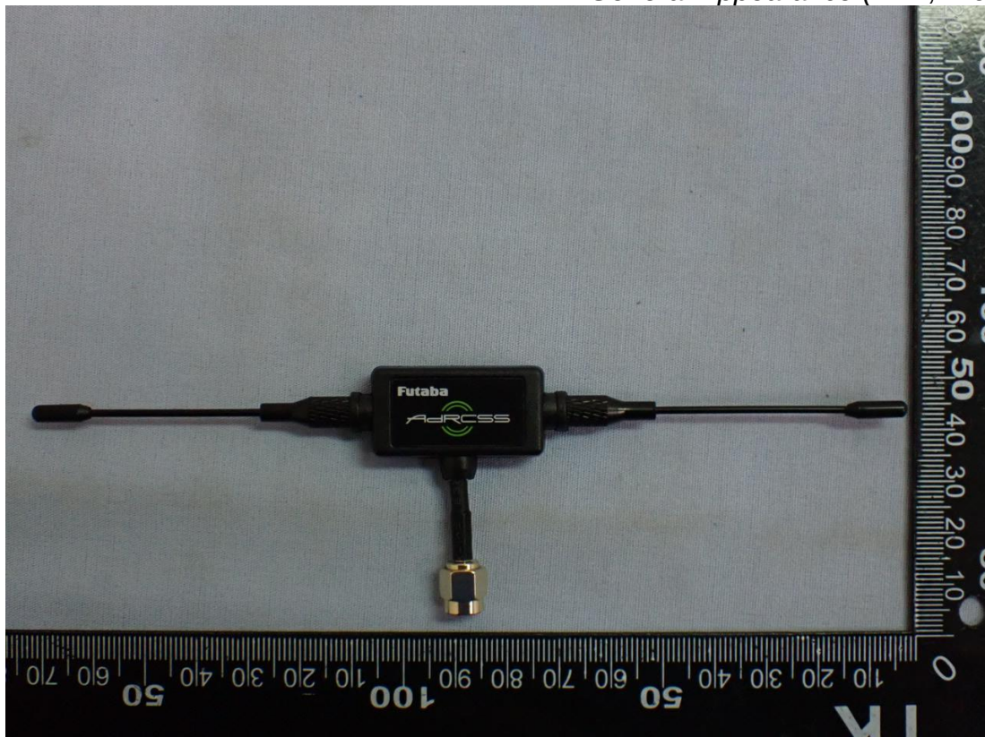
Figure 4 General Appearance (ANT, Front View)
