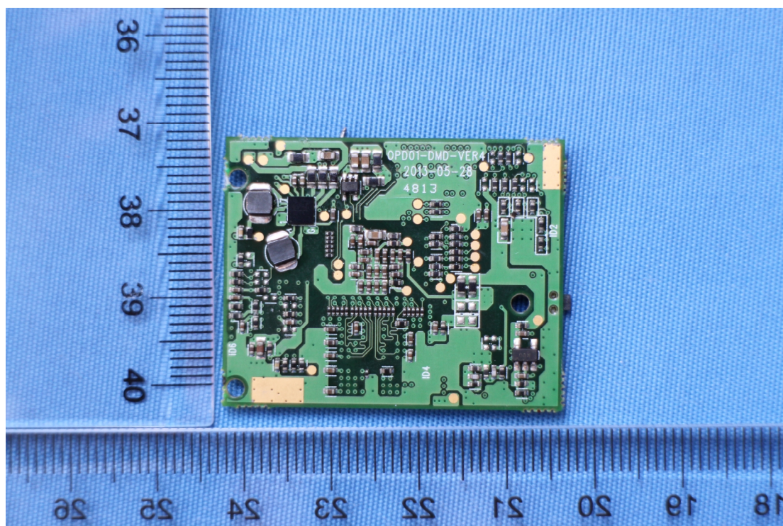
1.5 EUT – PCB Front View (3)
