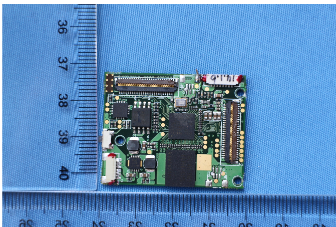
1.6 EUT – PCB Back View (4)
