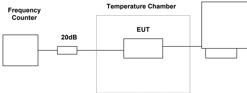
Figure 6.6.1.1-1: Frequency Stability Test Set-Up
