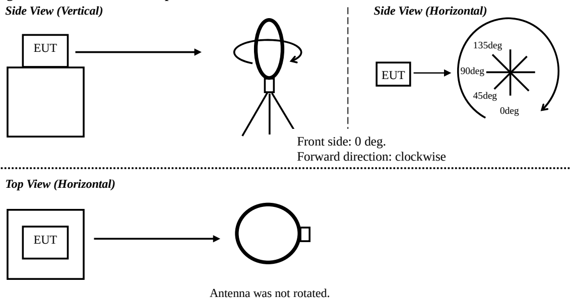
Figure 2. Antenna angle
