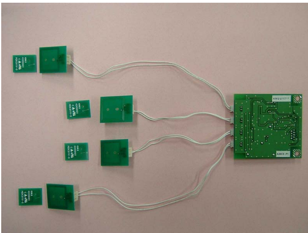
Inside view of Internal Circuit with antennas <Rear>
