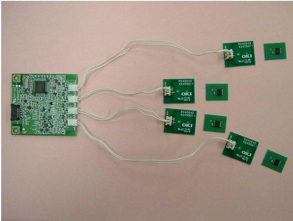
Inside view of Internal Circuit with antennas <Front>
