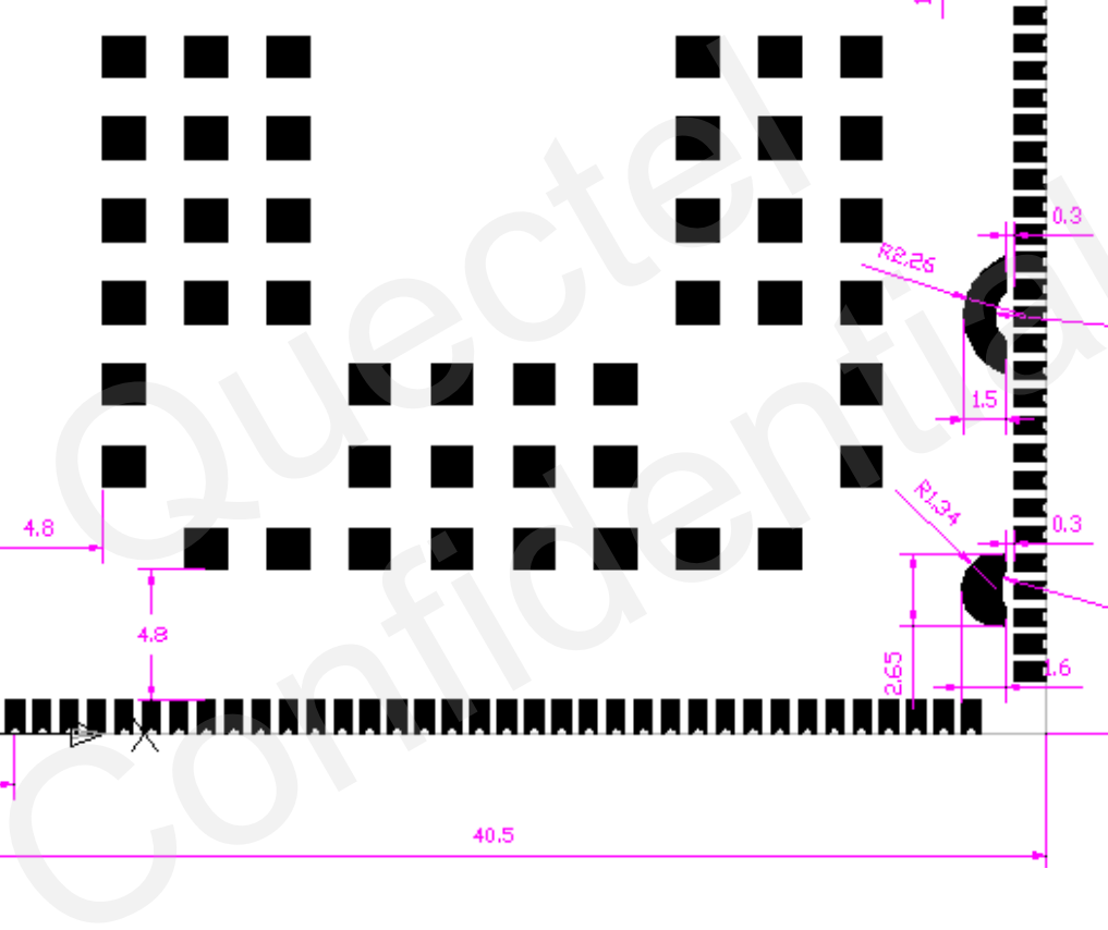
Figure 4: Module Bottom Dimensions (Top View)
