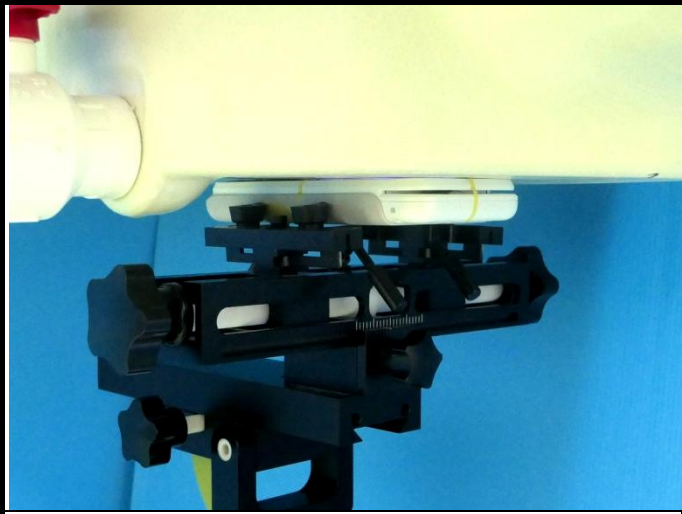
Extremity - Front Face of EUT at 0 mm
