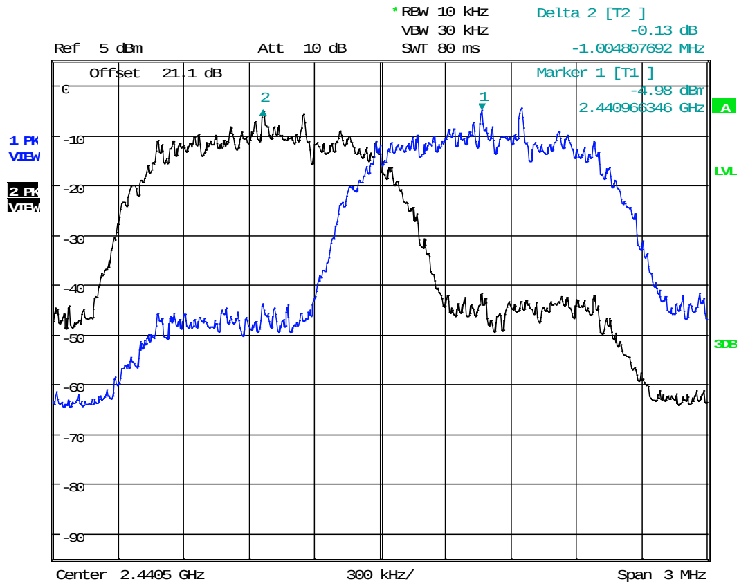
Plot 3.2– Channel Separation DPQSK
