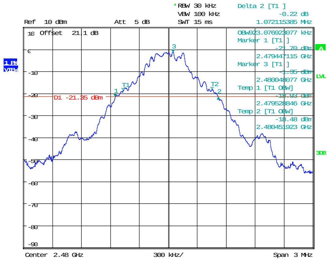
Plot 1. 3 – 20dB Bandwidth High Channel GFSK
