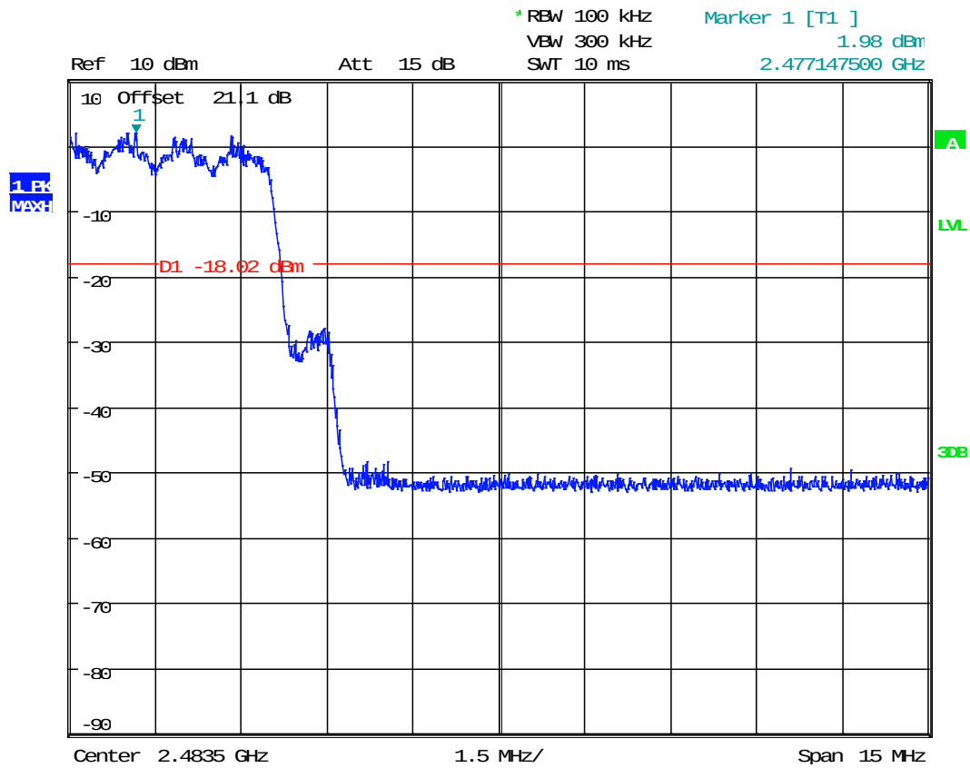
Plot 4.17 Conducted Band Edge, with \pi/4 -DQPSK (Hopping)
