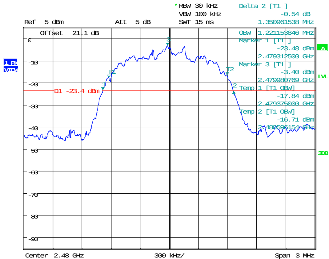
Plot 1. 9 – 20dB Bandwidth High Channel 8DPSK
