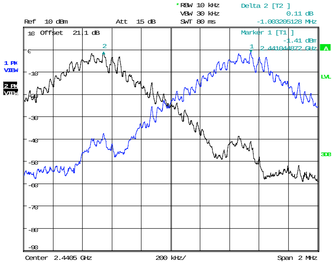
Plot 3.3– Channel Separation GFSK
