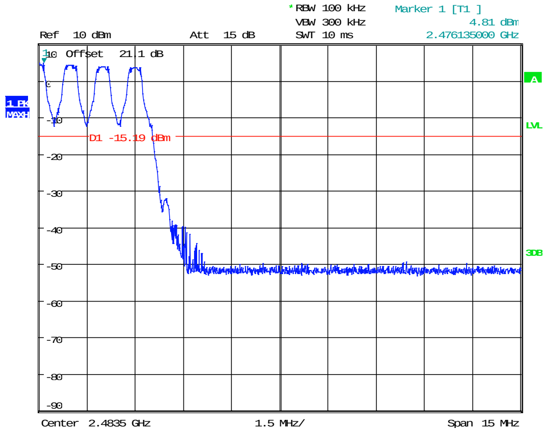
Plot 4.13 Conducted Band Edge, with GFSK (Hopping)
