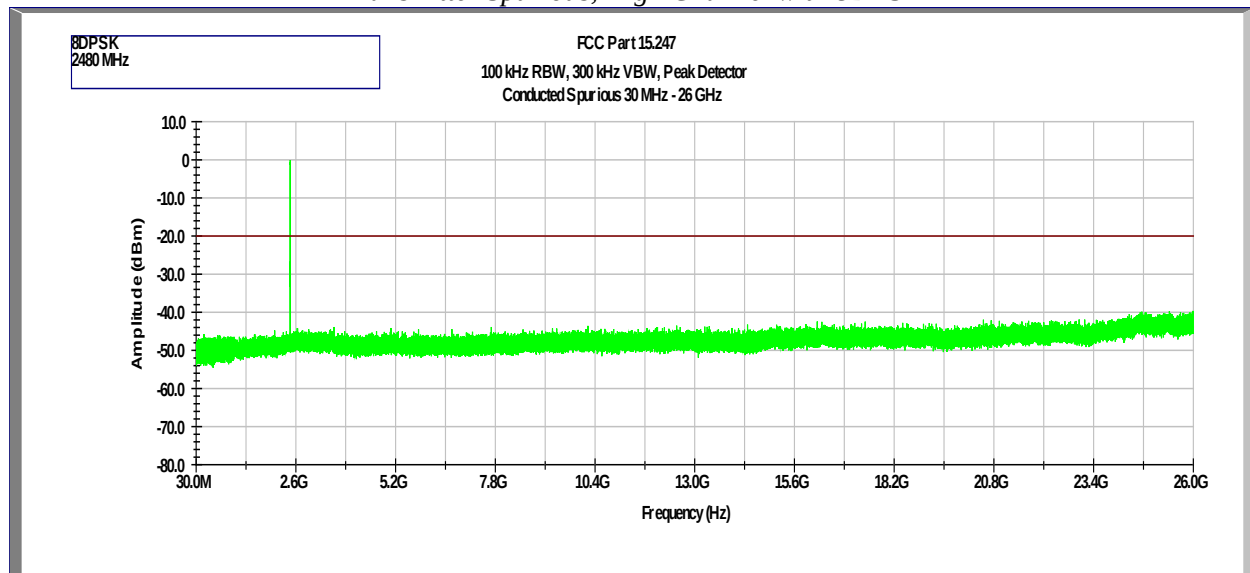
Plot 4.9 Transmitter Spurious, High Channel with 8DPSK
