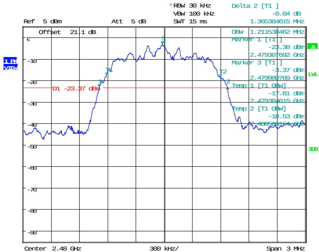
Plot 1. 6 – 20dB Bandwidth High Channel \pi/4 -DQPSK
