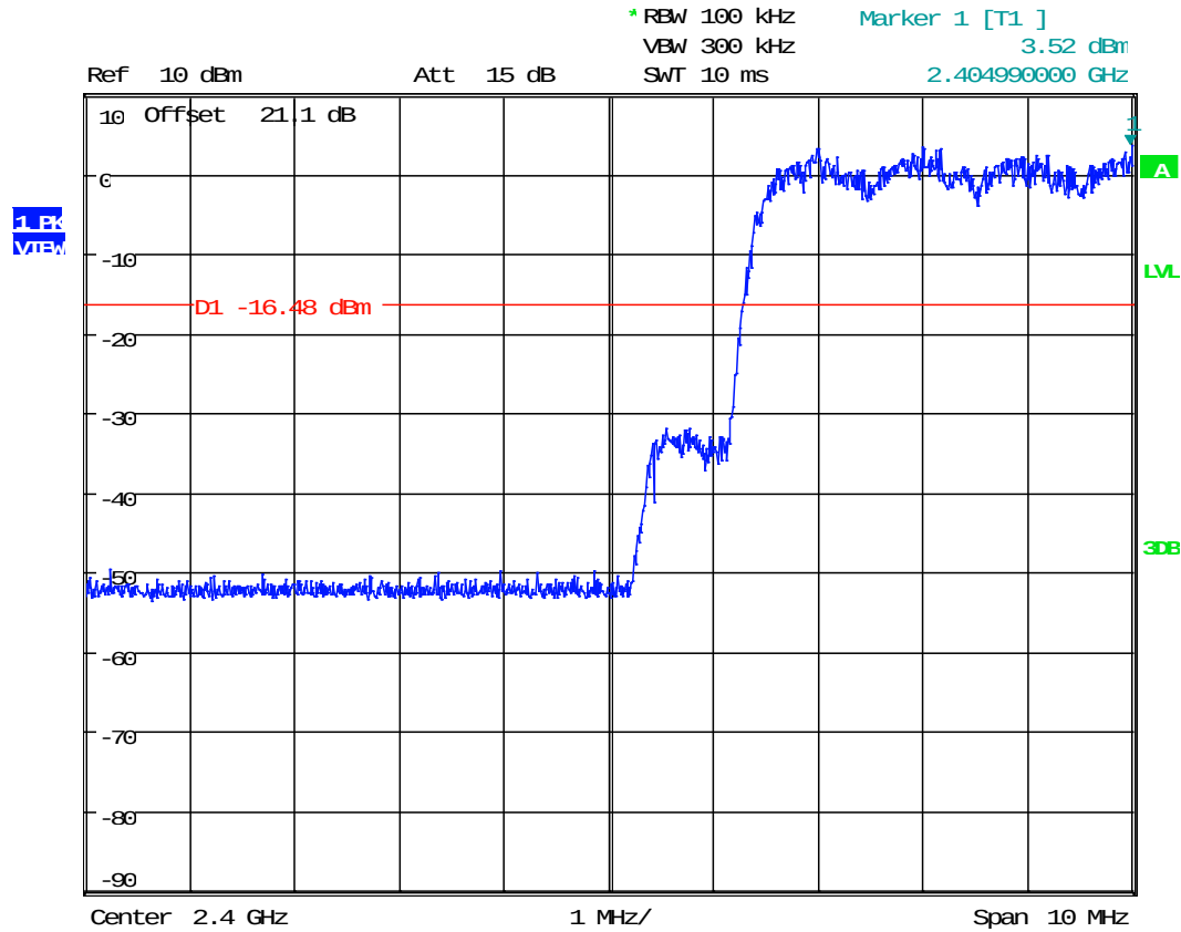
Plot 4.19 Conducted Band Edge, with 8DPSK (Hopping)
