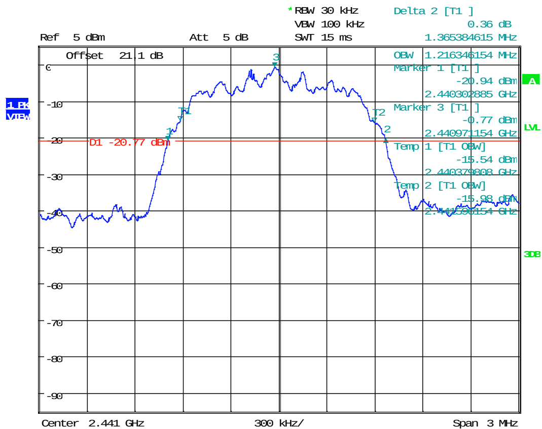
Plot 1.5 – 20dB Bandwidth Middle Channel \pi/4 -DQPSK
