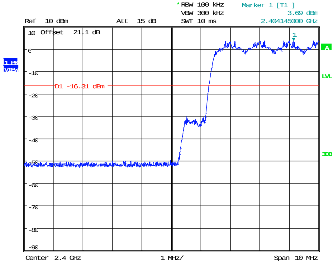
Plot 4.15 Conducted Band Edge, with \pi/4 -DQPSK (Hopping)
