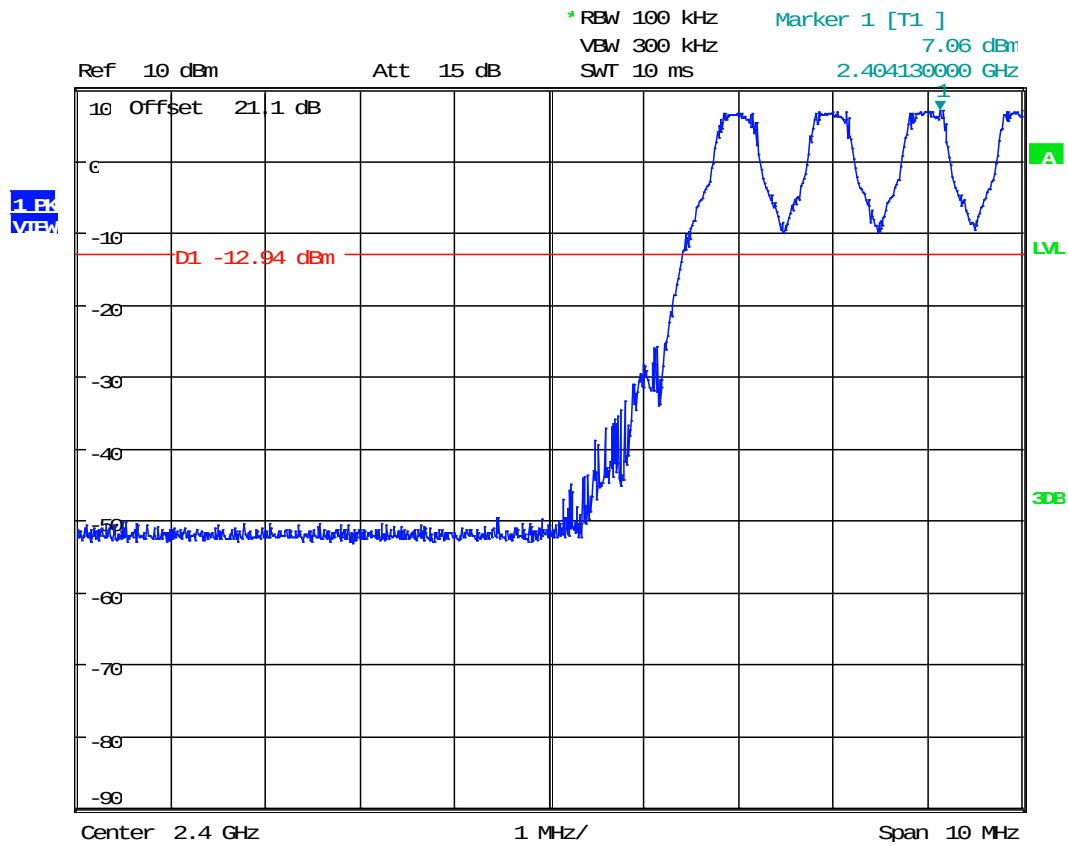
Plot 4.11 Conducted Band Edge, with GFSK (Hopping)
