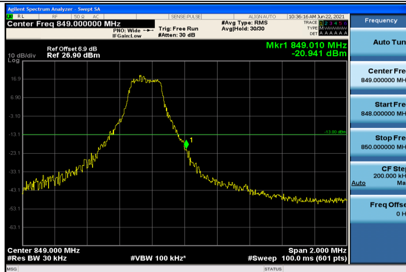
Band5-3MHz-16QAM-20635-1RB#14
