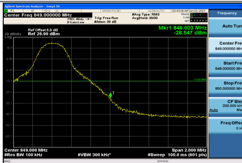
Band5-10MHz-QPSK-20600-1RB#49
