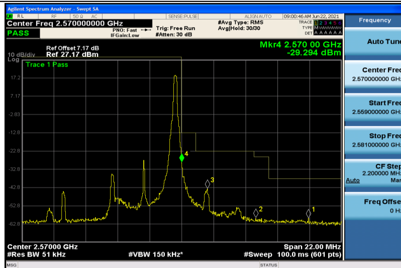
Band7-5MHz-16QAM-21425-1RB#24
