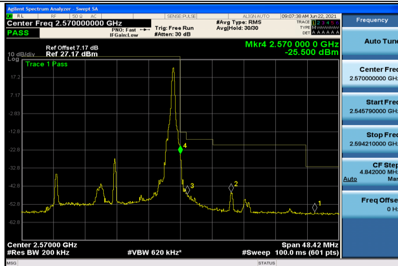
Band7-20MHz-16QAM-21350-1RB#99
