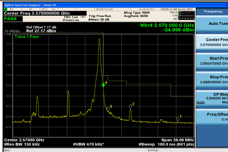
Band7-15MHz-QPSK-21375-1RB#74
