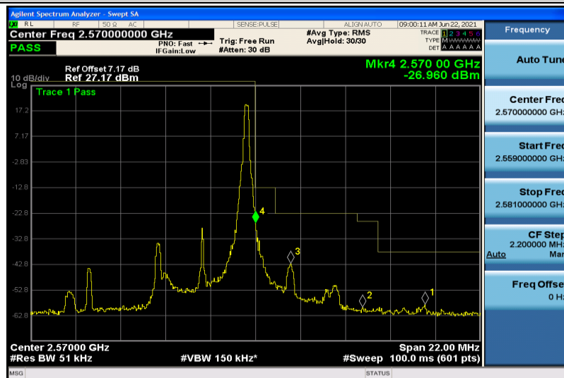
Band7-5MHz-QPSK-21425-1RB#24
