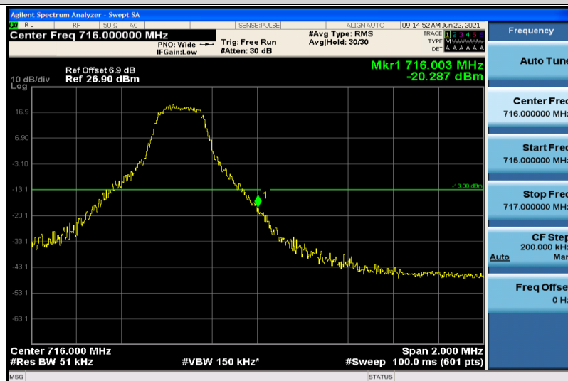
Band12-5MHz-16QAM-23155-1RB#24
