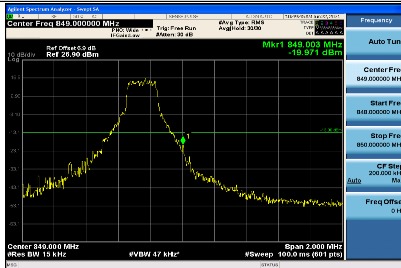
Band26-1.4MHz-16QAM-27033-1RB#5
