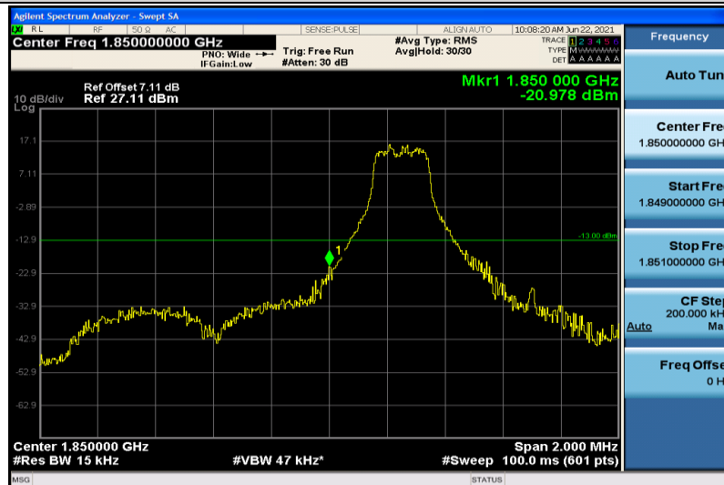
Band25-1.4MHz-16QAM-26047-1RB#0
