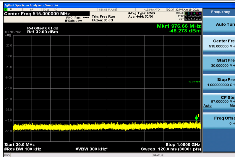
Band2-10MHz-16QAM-18900-1RB#0-30~1000MHz
