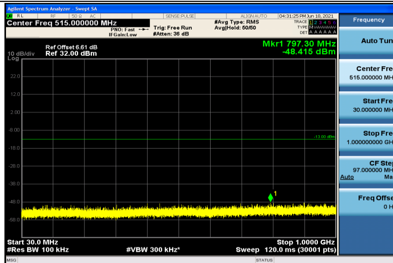
Band4-10MHz-QPSK-20175-1RB#0-30~1000MHz
