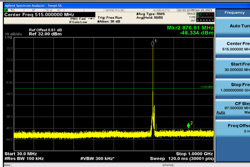
Band12-10MHz-QPSK-23095-1RB#0-30~1000MHz
