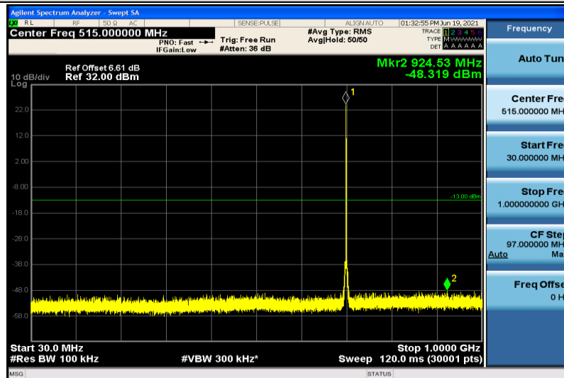
Band12-1.4MHz-QPSK-23095-1RB#0-30~1000MHz
