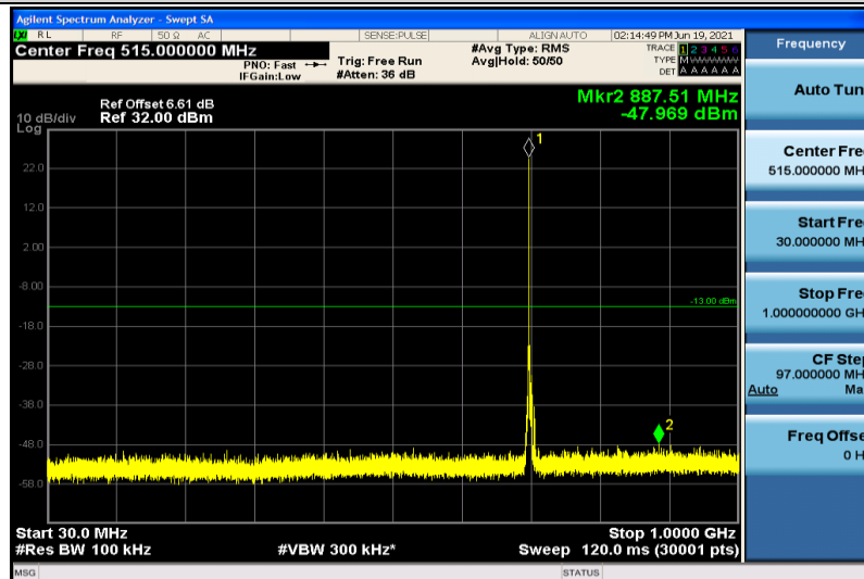
Band12-5MHz-QPSK-23095-1RB#0-30~1000MHz
