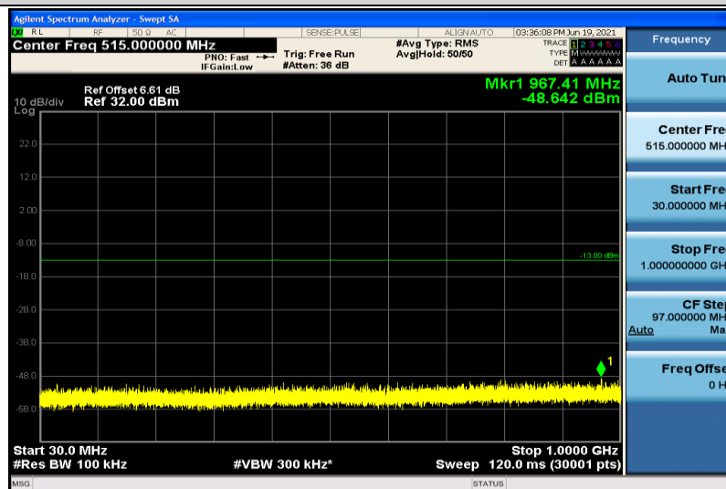
Band25-1.4MHz-16QAM-26683-1RB#0-30~1000MHz
