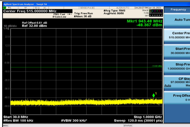
Band25-10MHz-16QAM-26640-1RB#0-30~1000MHz
