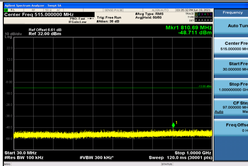
Band25-1.4MHz-QPSK-26683-1RB#0-30~1000MHz
