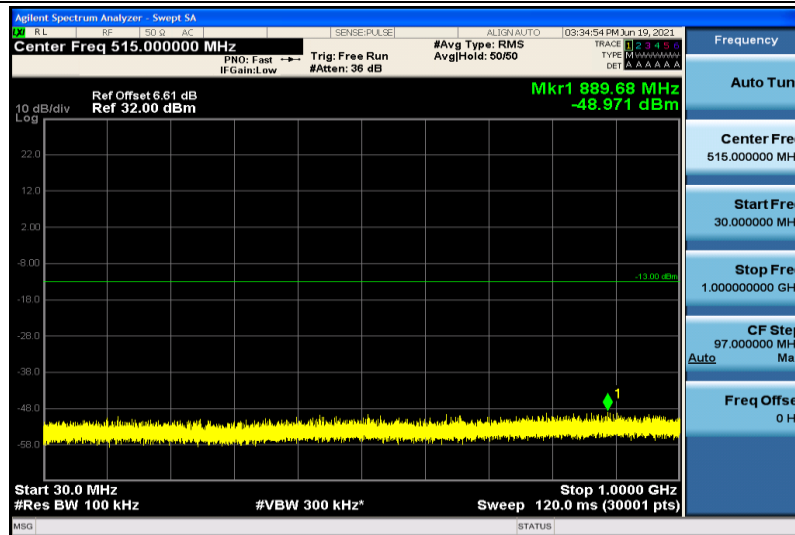
Band25-1.4MHz-16QAM-26365-1RB#0-30~1000MHz
