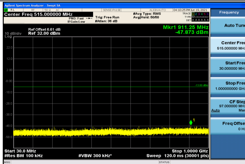
Band25-5MHz-QPSK-26665-1RB#0-30~1000MHz
