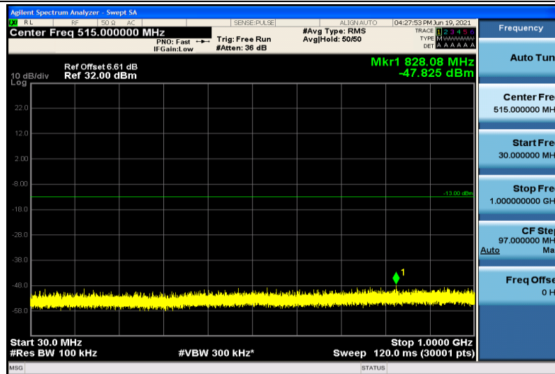
Band25-10MHz-16QAM-26365-1RB#0-30~1000MHz
