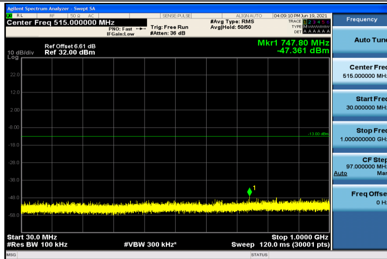
Band25-5MHz-QPSK-26365-1RB#0-30~1000MHz
