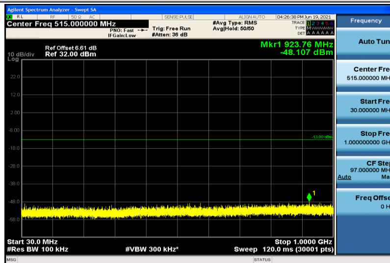
Band25-10MHz-16QAM-26090-1RB#0-30~1000MHz
