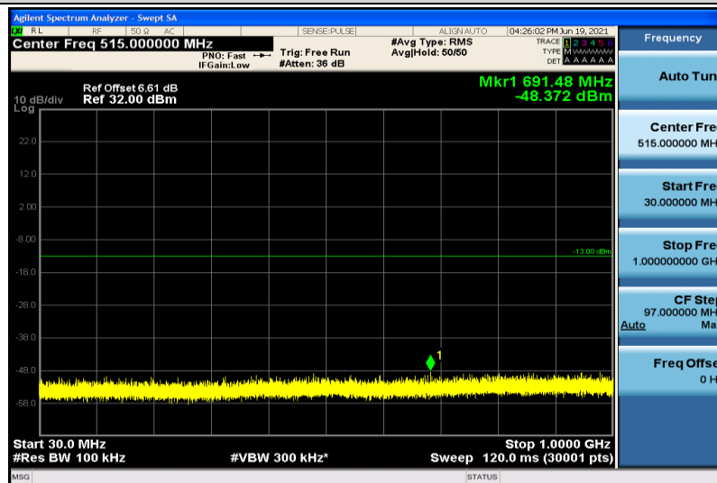
Band25-10MHz-QPSK-26090-1RB#0-30~1000MHz
