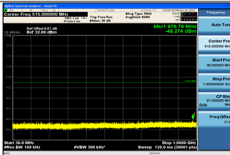
Band25-3MHz-QPSK-26675-1RB#0-30~1000MHz
