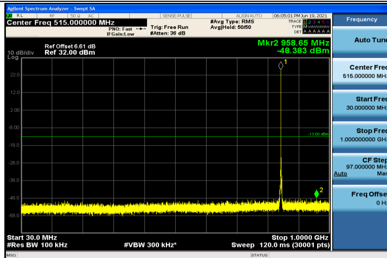
Band26-3MHz-16QAM-27025-1RB#0-30~1000MHz
