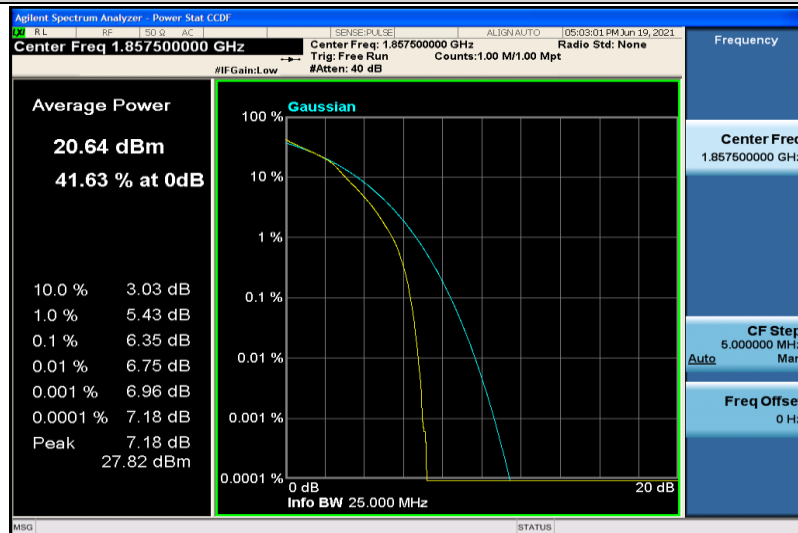
Band25-15MHz-16QAM-26115-75RB#0
