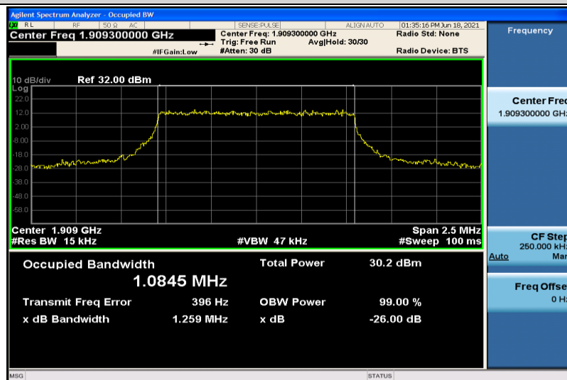
Band2-1.4MHz-QPSK-19193-6RB#0-1.0845
