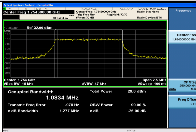
Band4-1.4MHz-16QAM-20393-6RB#0-1.0834
