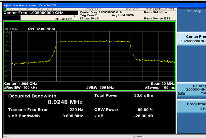
Band2-10MHz-16QAM-19150-50RB#0-8.9248
