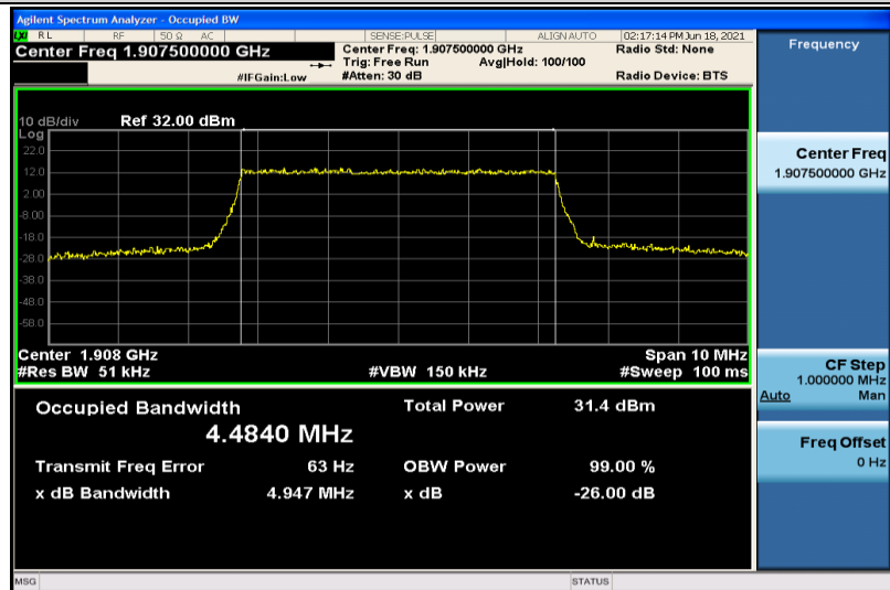
Band2-5MHz-QPSK-19175-25RB#0-4.4840
