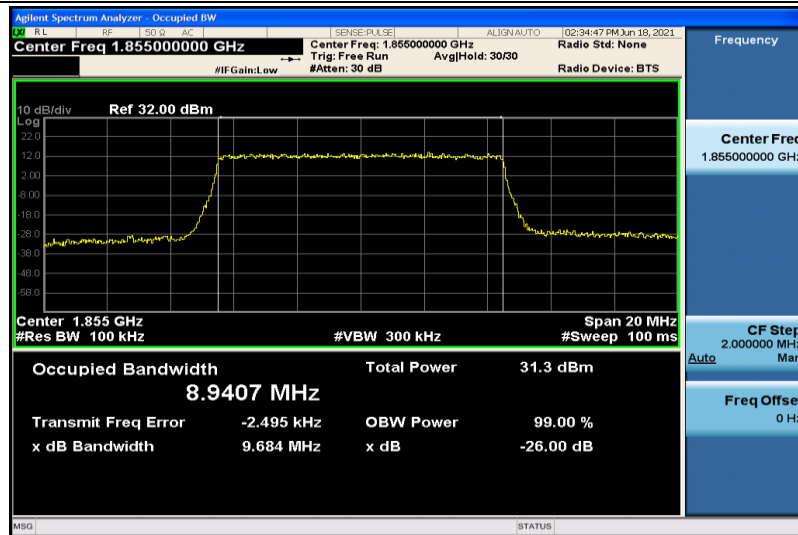
Band2-10MHz-16QAM-18650-50RB#0-8.9407
