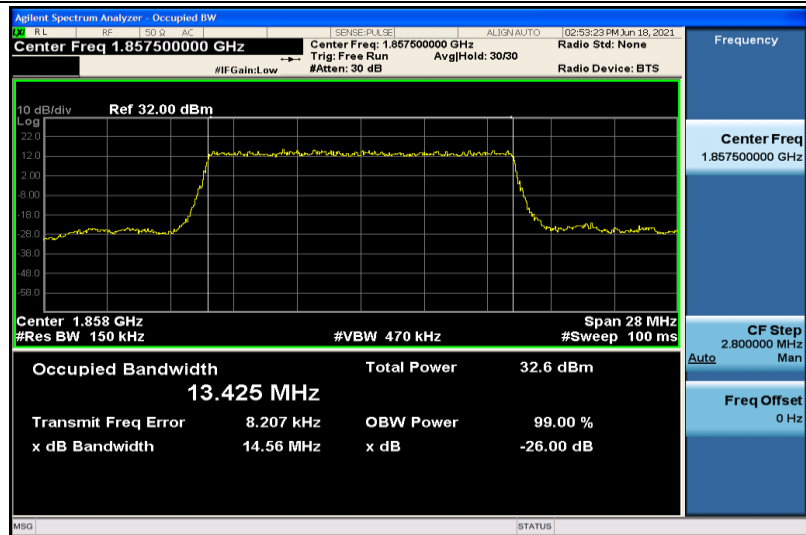
Band2-15MHz-QPSK-18675-75RB#0-13.425
