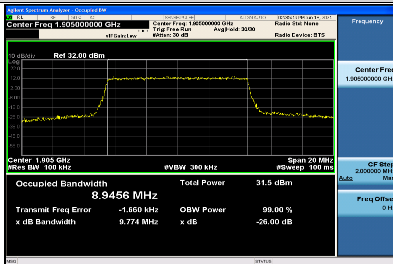
Band2-10MHz-QPSK-19150-50RB#0-8.9456
