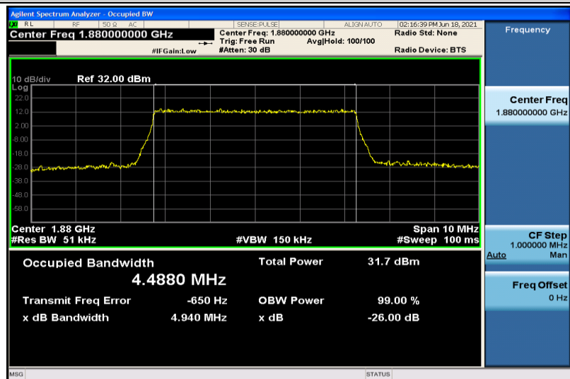
Band2-5MHz-QPSK-18900-25RB#0-4.4880
