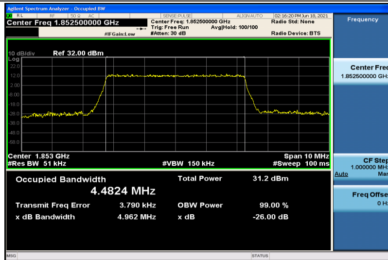
Band2-5MHz-16QAM-18625-25RB#0-4.4824
