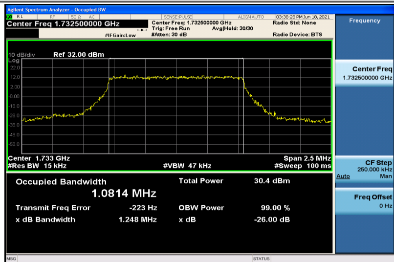
Band4-1.4MHz-QPSK-20175-6RB#0-1.0814
