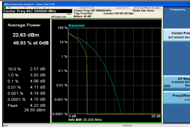
Band26-3MHz-QPSK-27025-1RB#0
