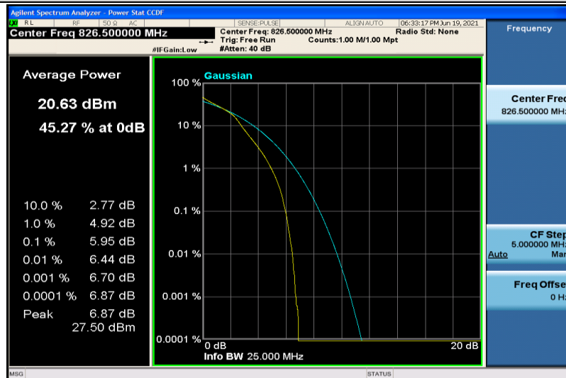
Band26-5MHz-16QAM-26815-25RB#0
