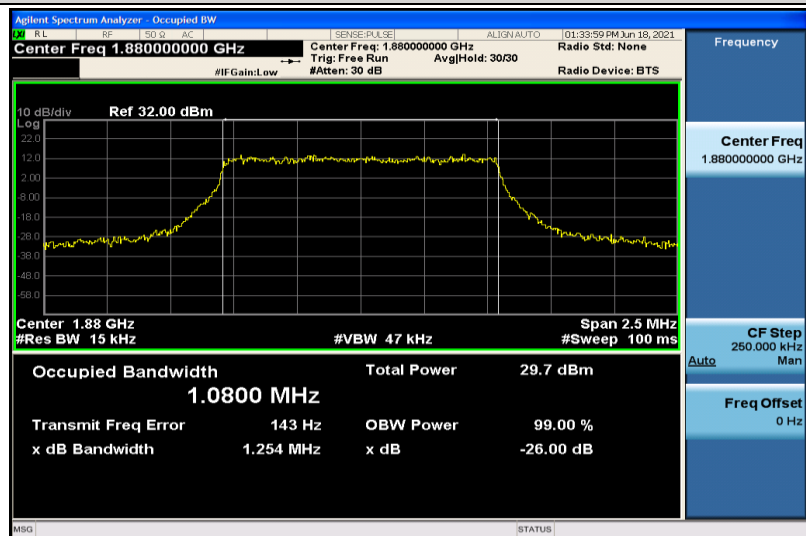
Band2-1.4MHz-16QAM-18900-6RB#0-1.0800
