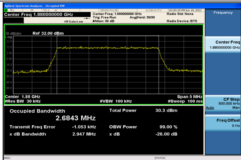
Band2-3MHz-16QAM-18900-15RB#0-2.6843
