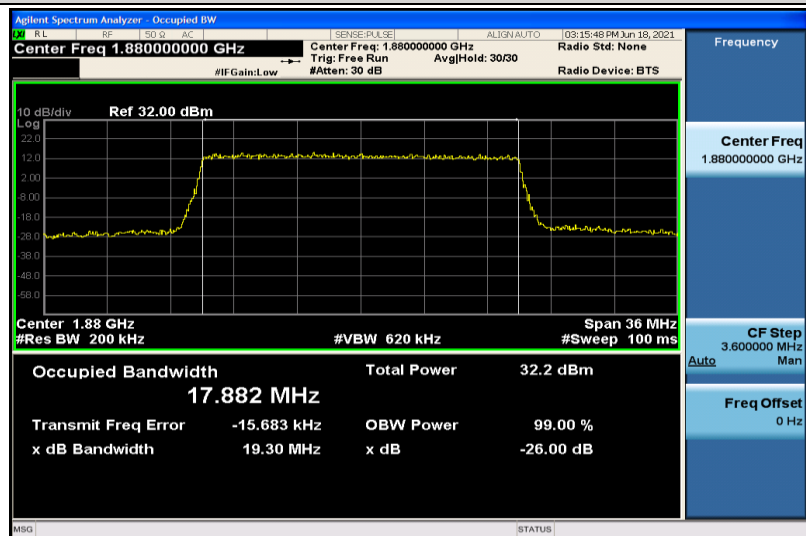
Band2-20MHz-QPSK-18900-100RB#0-17.882
