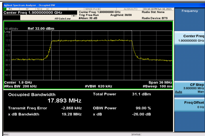
Band2-20MHz-16QAM-19100-100RB#0-17.893
