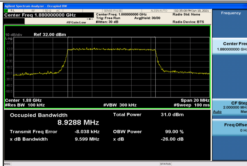
Band2-10MHz-16QAM-18900-50RB#0-8.9288
