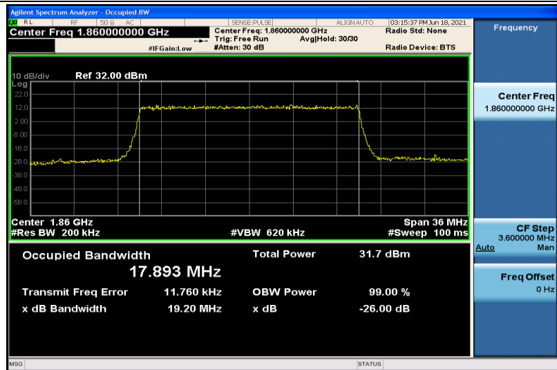
Band2-20MHz-16QAM-18700-100RB#0-17.893
