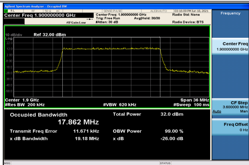
Band2-20MHz-QPSK-19100-100RB#0-17.862
