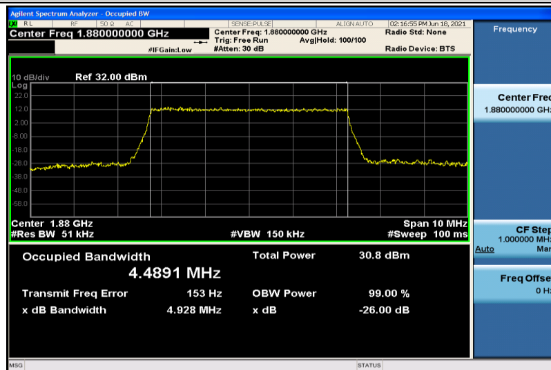
Band2-5MHz-16QAM-18900-25RB#0-4.4891
