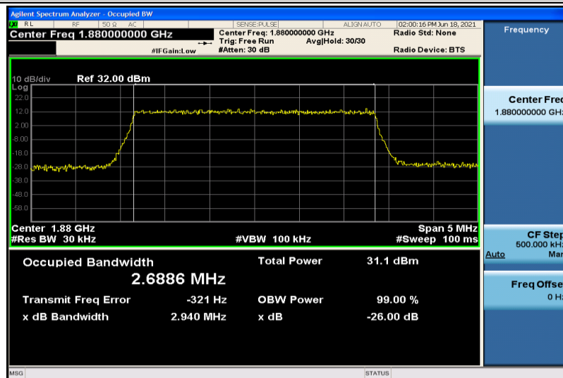
Band2-3MHz-QPSK-18900-15RB#0-2.6886
