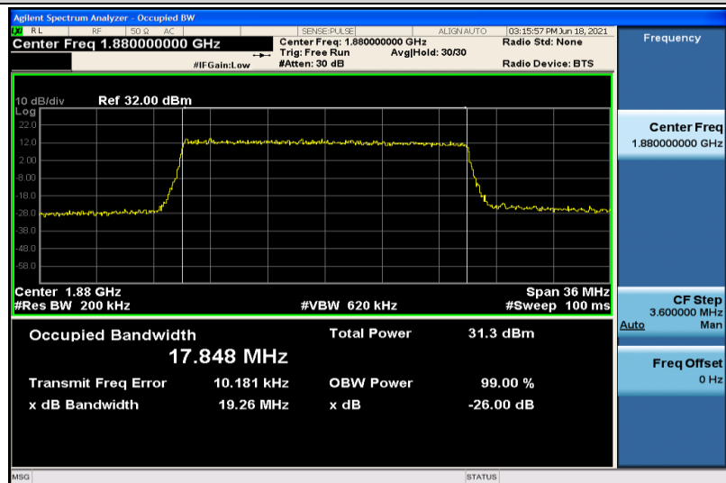
Band2-20MHz-16QAM-18900-100RB#0-17.848
