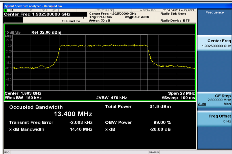
Band2-15MHz-QPSK-19125-75RB#0-13.400
