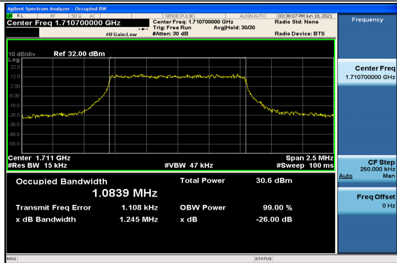
Band4-1.4MHz-QPSK-19957-6RB#0-1.0839
