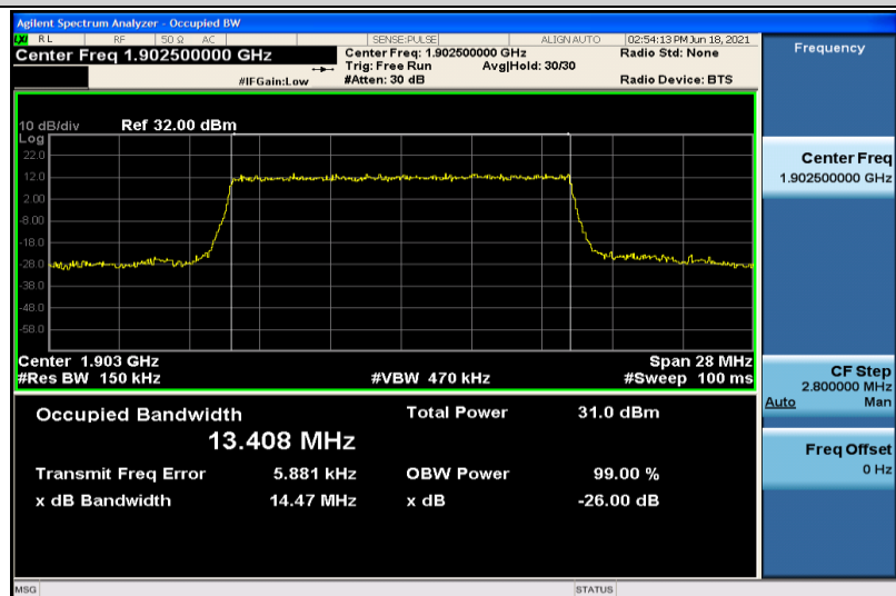
Band2-15MHz-16QAM-19125-75RB#0-13.408
