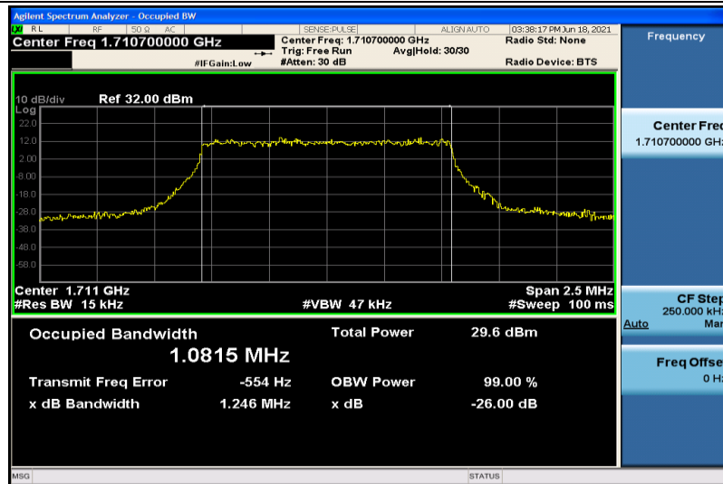
Band4-1.4MHz-16QAM-19957-6RB#0-1.0815
