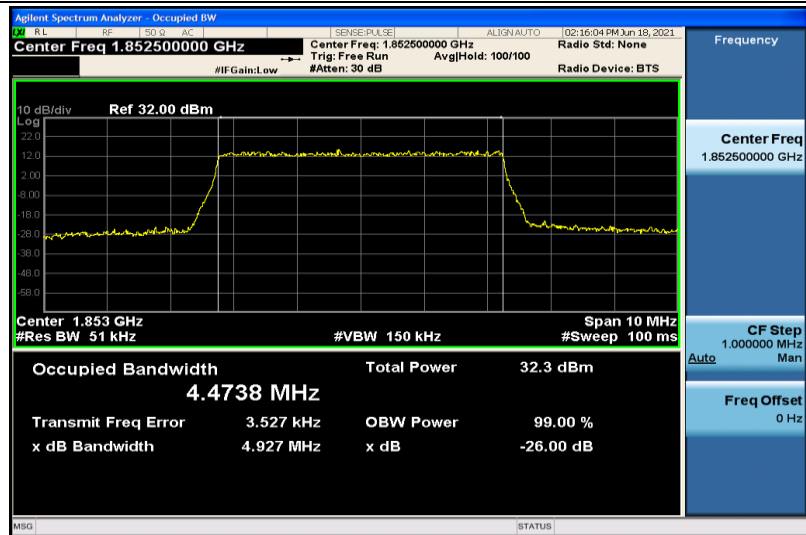
Band2-5MHz-QPSK-18625-25RB#0-4.4738
