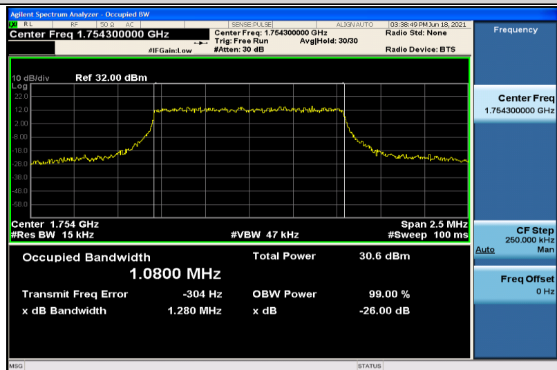
Band4-1.4MHz-QPSK-20393-6RB#0-1.0800
