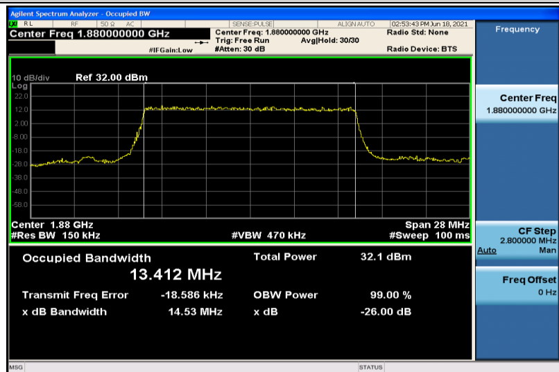
Band2-15MHz-QPSK-18900-75RB#0-13.412
