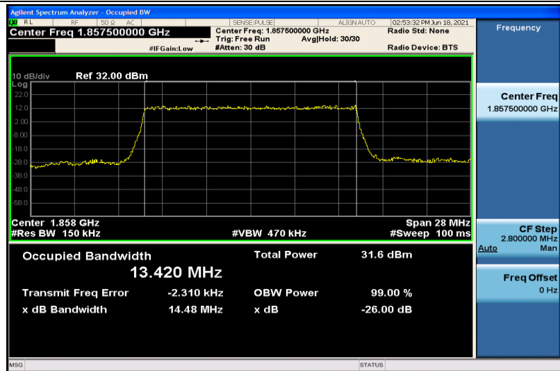
Band2-15MHz-16QAM-18675-75RB#0-13.420
