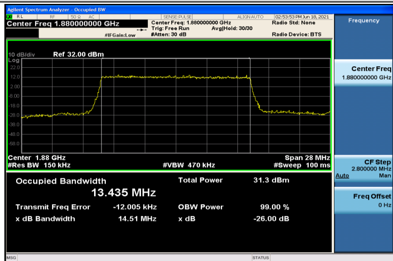
Band2-15MHz-16QAM-18900-75RB#0-13.435
