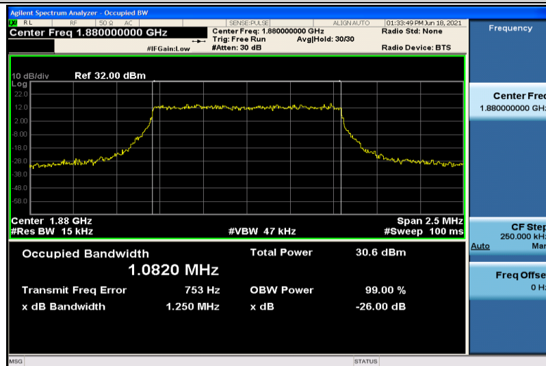
Band2-1.4MHz-QPSK-18900-6RB#0-1.0820
