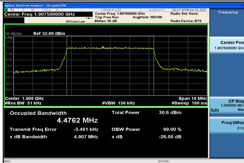
Band2-5MHz-16QAM-19175-25RB#0-4.4762
