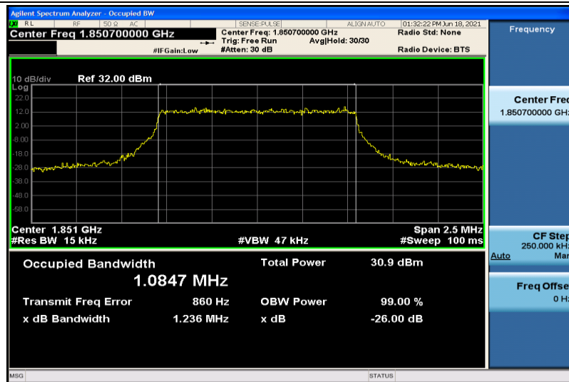
Band2-1.4MHz-QPSK-18607-6RB#0-1.0847
