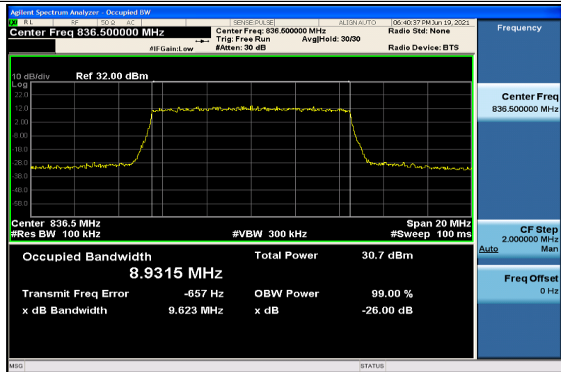
Band26-10MHz-QPSK-26915-50RB#0-8.9315
