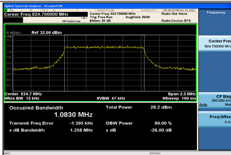
Band26-1.4MHz-16QAM-26797-6RB#0-1.0830
