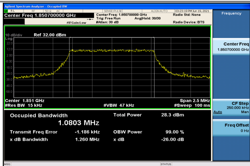
Band25-1.4MHz-16QAM-26047-6RB#0-1.0803
