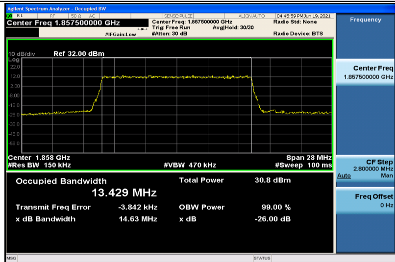
Band25-15MHz-QPSK-26115-75RB#0-13.429
