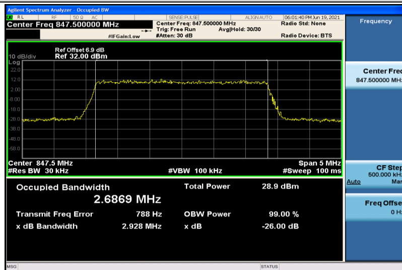
Band26-3MHz-16QAM-27025-15RB#0-2.6869
