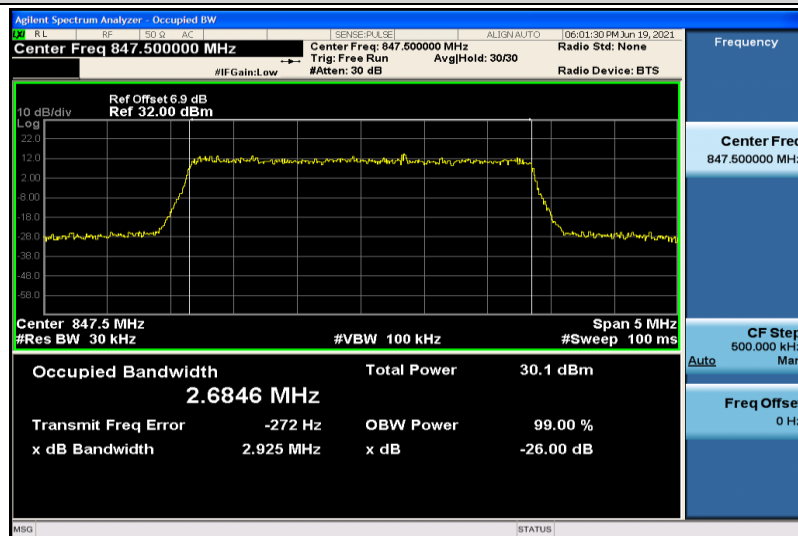
Band26-3MHz-QPSK-27025-15RB#0-2.6846
