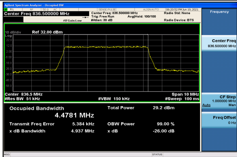
Band26-5MHz-16QAM-26915-25RB#0-4.4781
