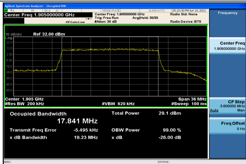
Band25-20MHz-16QAM-26590-100RB#0-17.841
