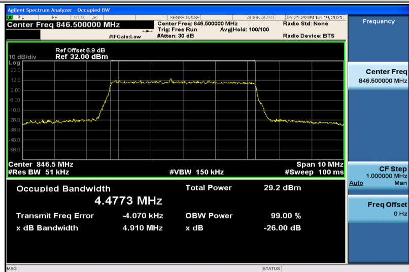
Band26-5MHz-16QAM-27015-25RB#0-4.4773
