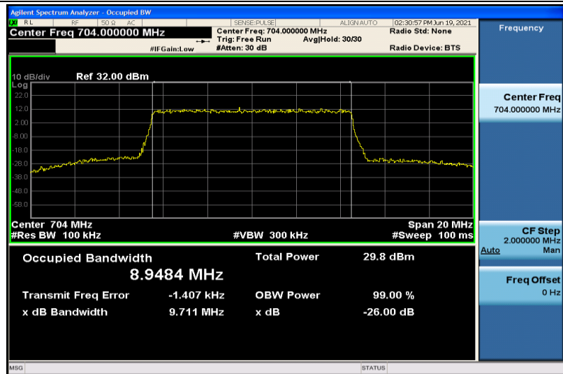
Band12-10MHz-16QAM-23060-50RB#0-8.9484
