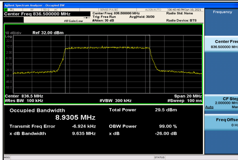
Band26-10MHz-16QAM-26915-50RB#0-8.9305
