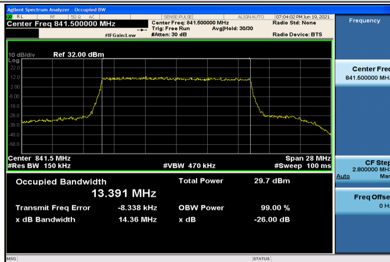
Band26-15MHz-16QAM-26965-75RB#0-13.391
