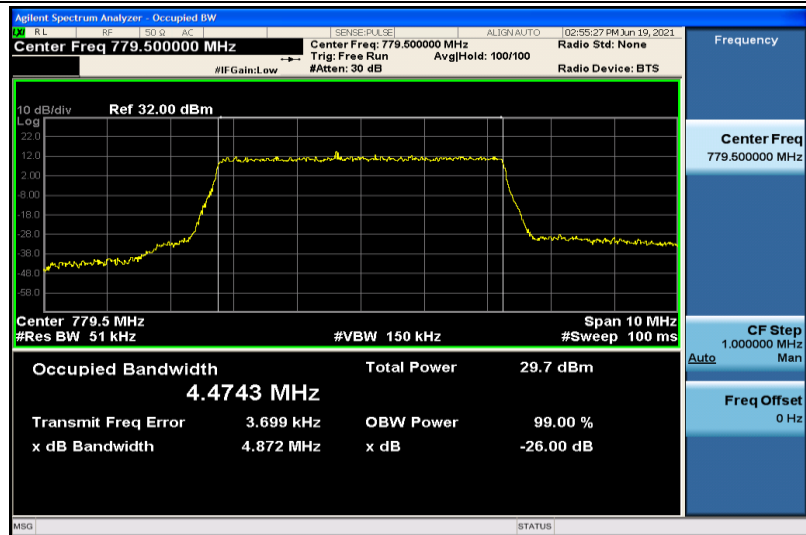
Band13-5MHz-16QAM-23205-25RB#0-4.4743
