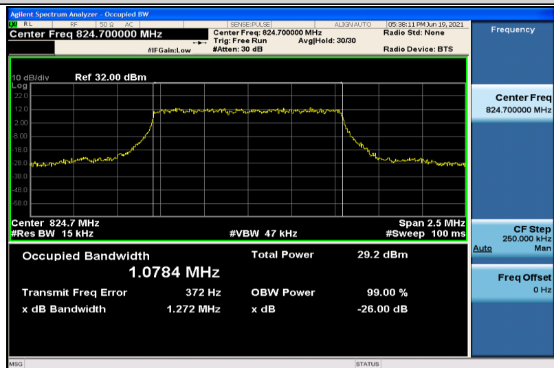
Band26-1.4MHz-QPSK-26797-6RB#0-1.0784
