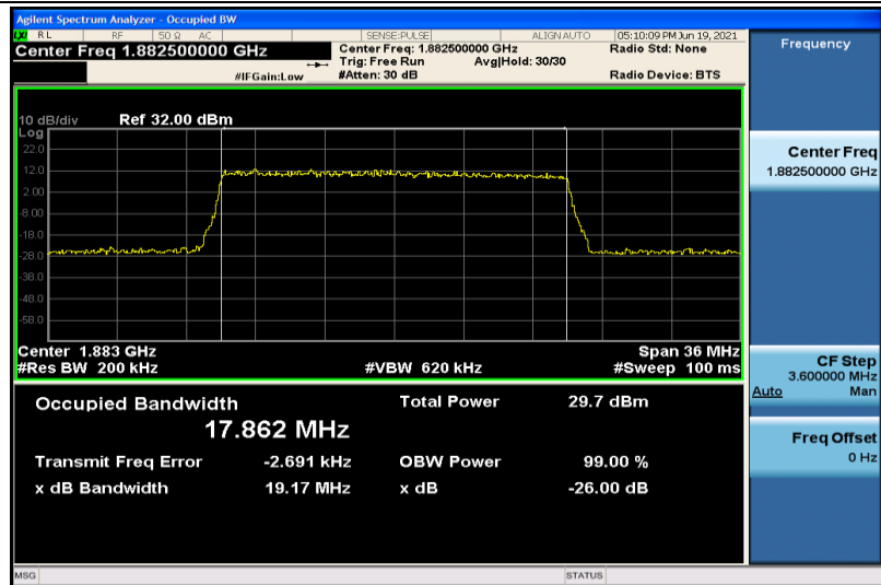
Band25-20MHz-16QAM-26365-100RB#0-17.862
