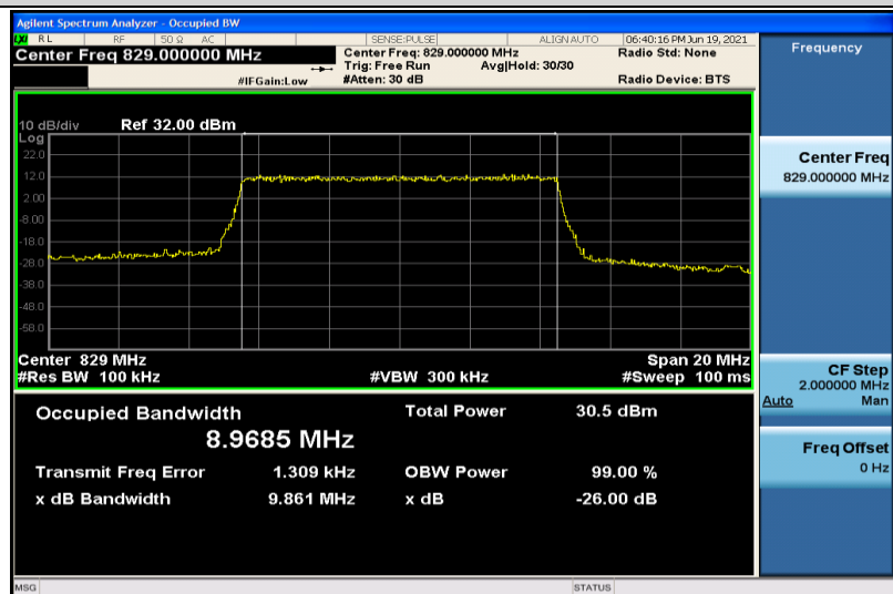
Band26-10MHz-QPSK-26840-50RB#0-8.9685
