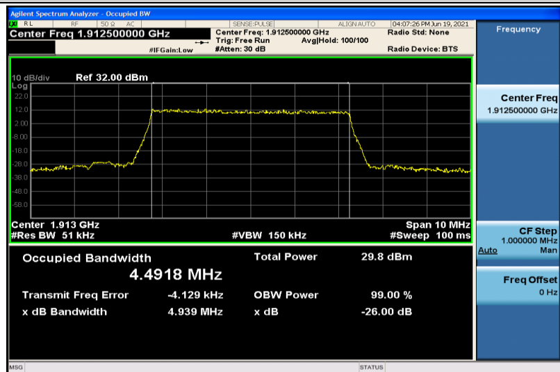
Band25-5MHz-QPSK-26665-25RB#0-4.4918
