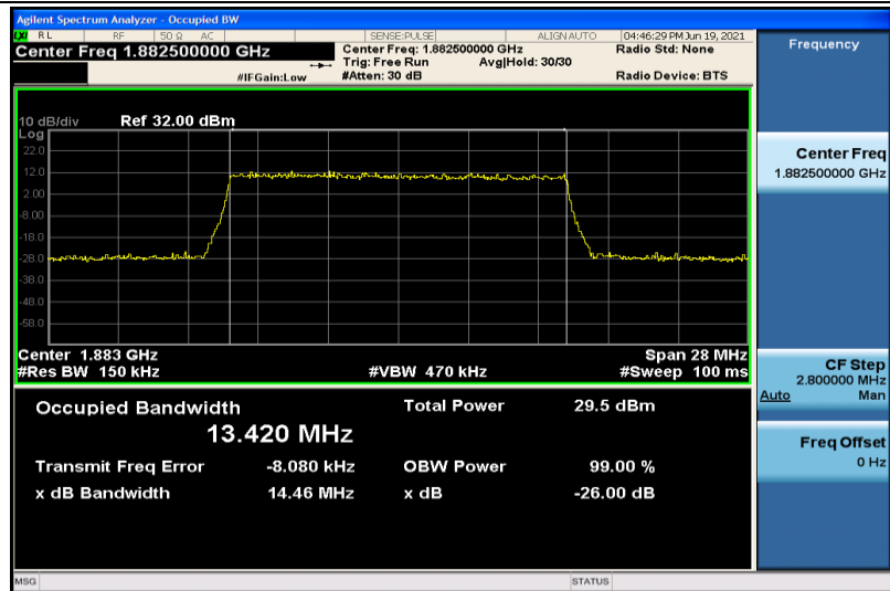
Band25-15MHz-16QAM-26365-75RB#0-13.420
