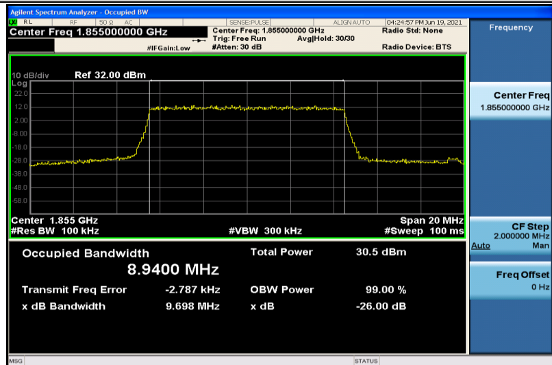
Band25-10MHz-QPSK-26090-50RB#0-8.9400
