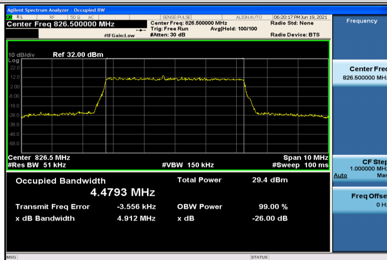
Band26-5MHz-16QAM-26815-25RB#0-4.4793
