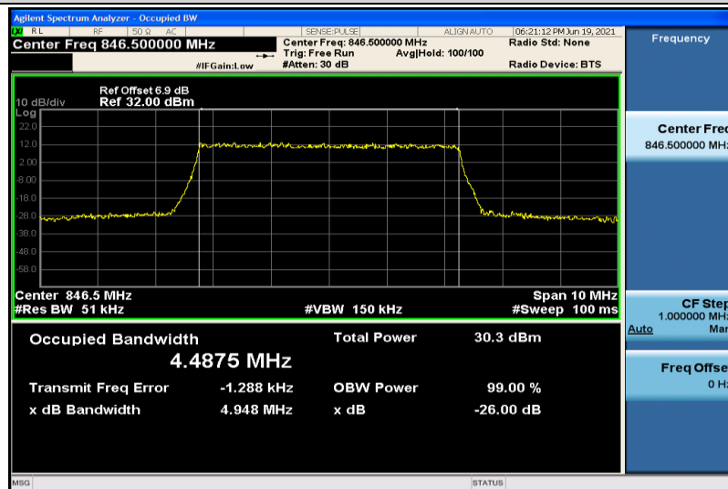
Band26-5MHz-QPSK-27015-25RB#0-4.4875
