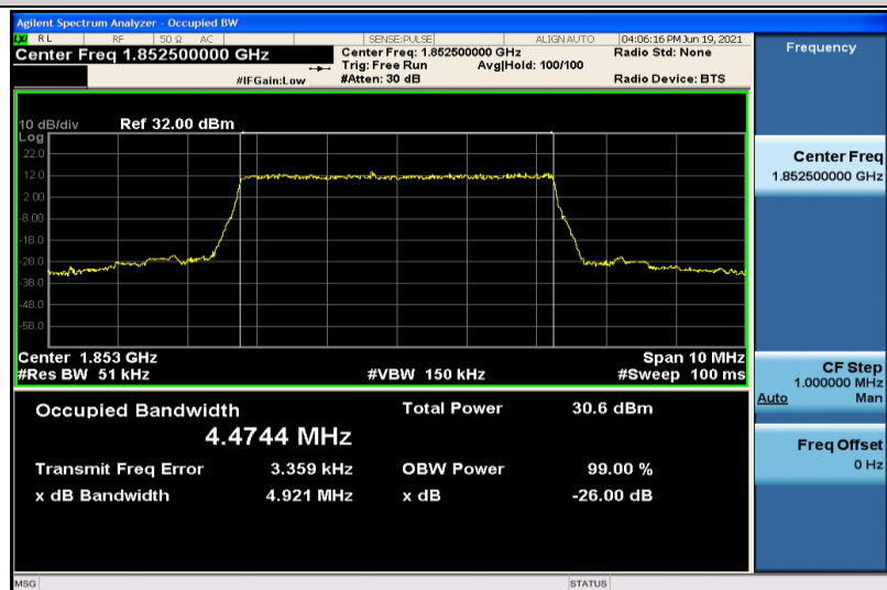
Band25-5MHz-QPSK-26065-25RB#0-4.4744
