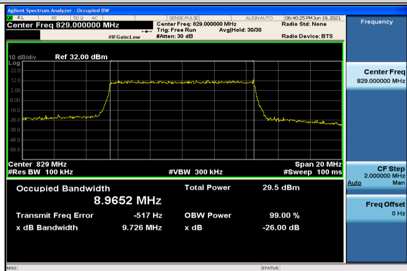
Band26-10MHz-16QAM-26840-50RB#0-8.9652
