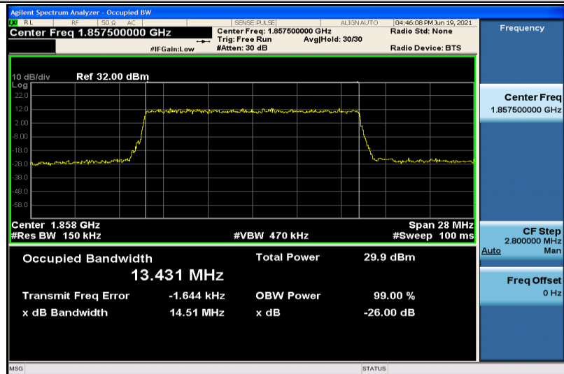
Band25-15MHz-16QAM-26115-75RB#0-13.431
