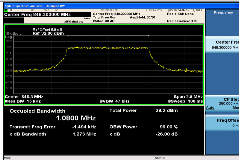
Band26-1.4MHz-QPSK-27033-6RB#0-1.0800
