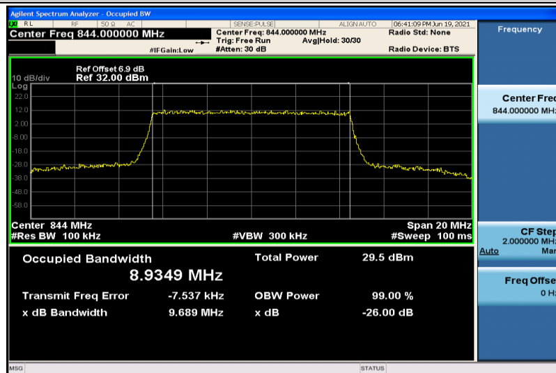
Band26-10MHz-16QAM-26990-50RB#0-8.9349
