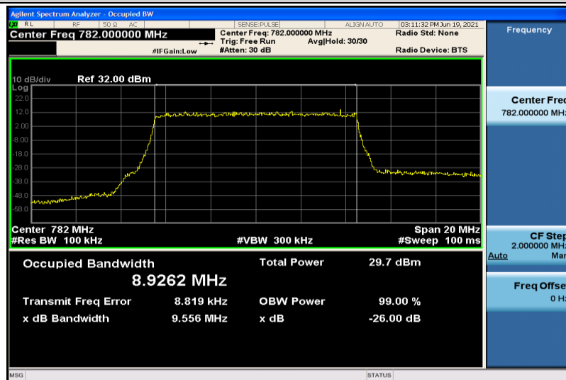
Band13-10MHz-16QAM-23230-50RB#0-8.9262
