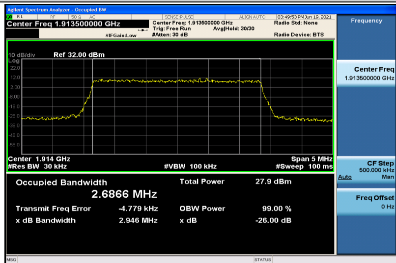
Band25-3MHz-16QAM-26675-15RB#0-2.6866
