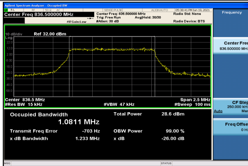
Band26-1.4MHz-16QAM-26915-6RB#0-1.0811
