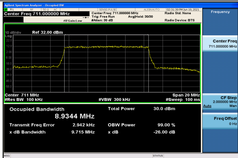
Band12-10MHz-16QAM-23130-50RB#0-8.9344
