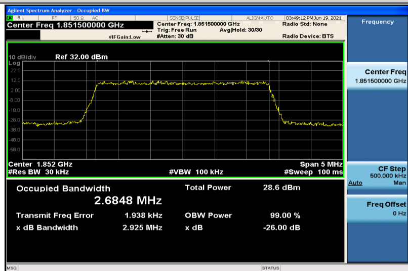
Band25-3MHz-16QAM-26055-15RB#0-2.6848
