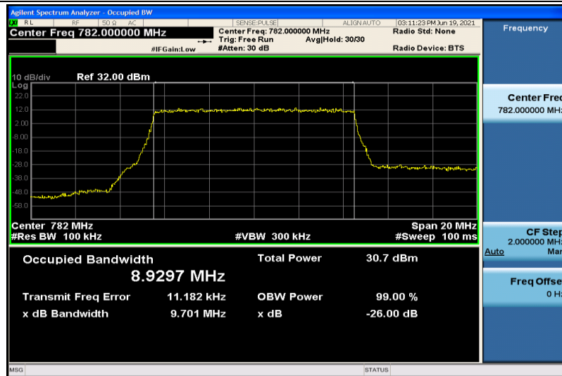
Band13-10MHz-QPSK-23230-50RB#0-8.9297
