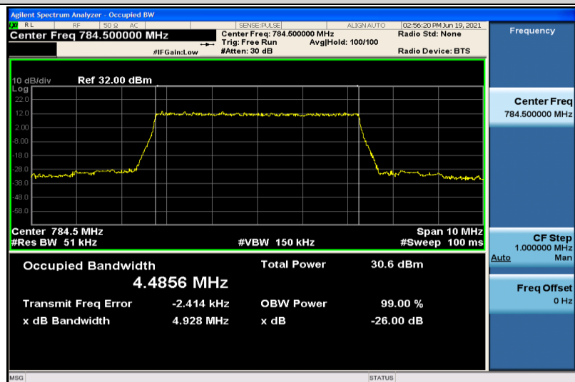
Band13-5MHz-QPSK-23255-25RB#0-4.4856
