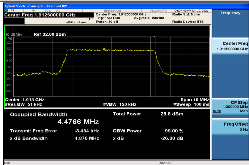
Band25-5MHz-16QAM-26665-25RB#0-4.4766
