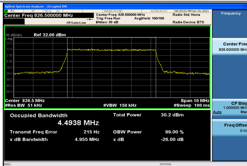
Band26-5MHz-QPSK-26815-25RB#0-4.4938
