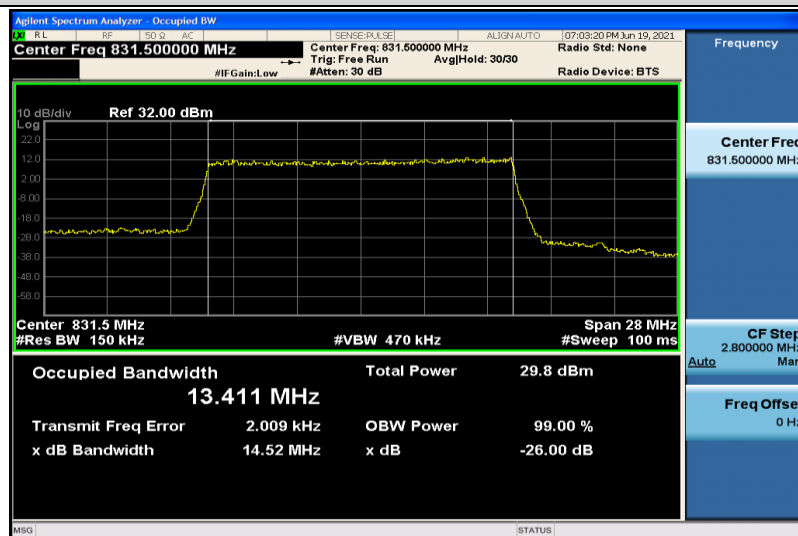
Band26-15MHz-16QAM-26865-75RB#0-13.411
