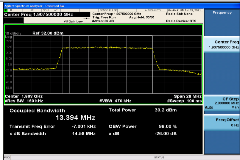
Band25-15MHz-QPSK-26615-75RB#0-13.394
