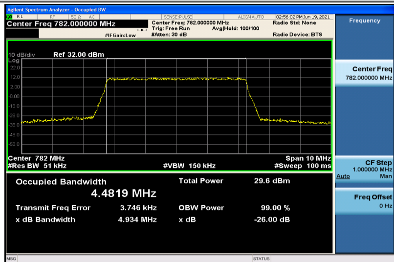
Band13-5MHz-16QAM-23230-25RB#0-4.4819
