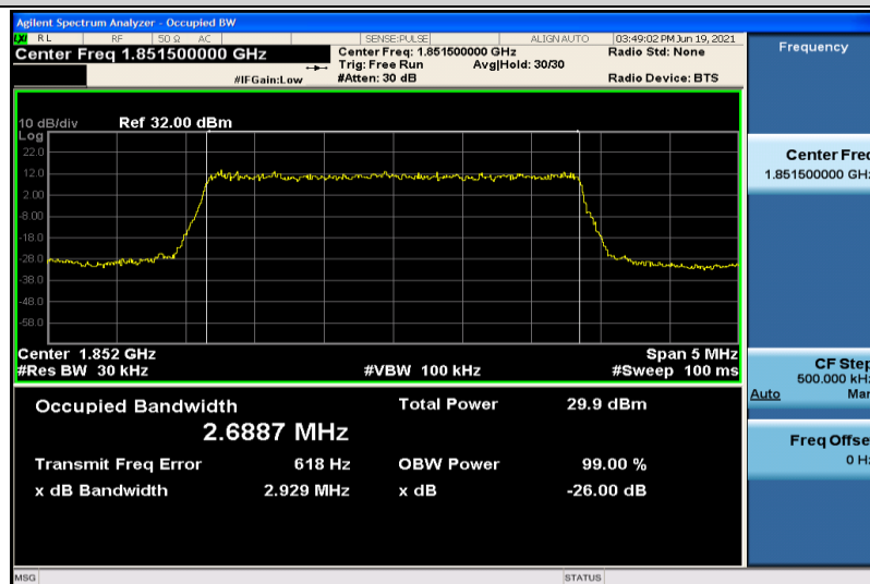
Band25-3MHz-QPSK-26055-15RB#0-2.6887
