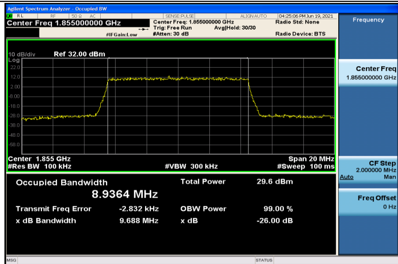
Band25-10MHz-16QAM-26090-50RB#0-8.9364
