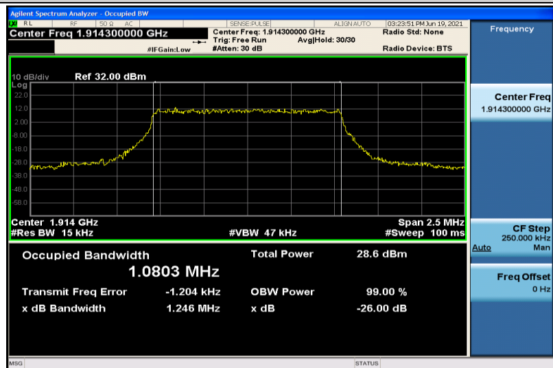
Band25-1.4MHz-QPSK-26683-6RB#0-1.0803
