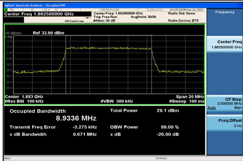
Band25-10MHz-16QAM-26365-50RB#0-8.9336
