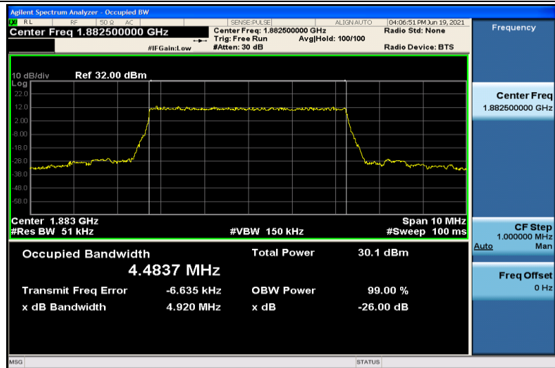
Band25-5MHz-QPSK-26365-25RB#0-4.4837
