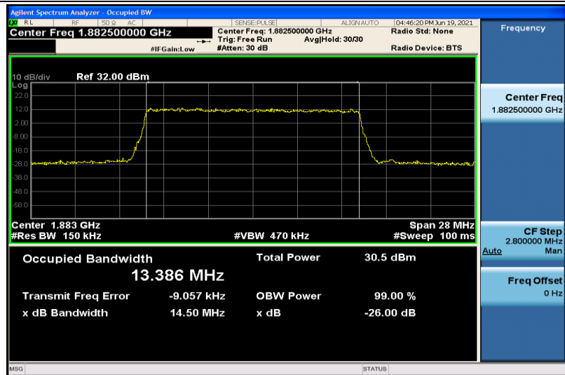
Band25-15MHz-QPSK-26365-75RB#0-13.386
