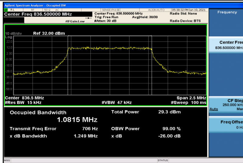
Band26-1.4MHz-QPSK-26915-6RB#0-1.0815
