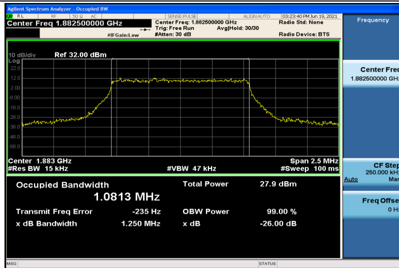
Band25-1.4MHz-16QAM-26365-6RB#0-1.0813
