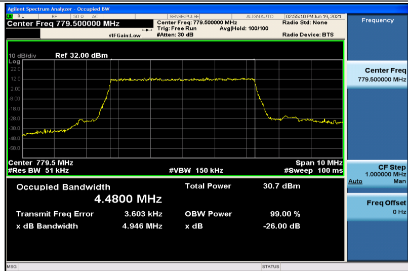
Band13-5MHz-QPSK-23205-25RB#0-4.4800
