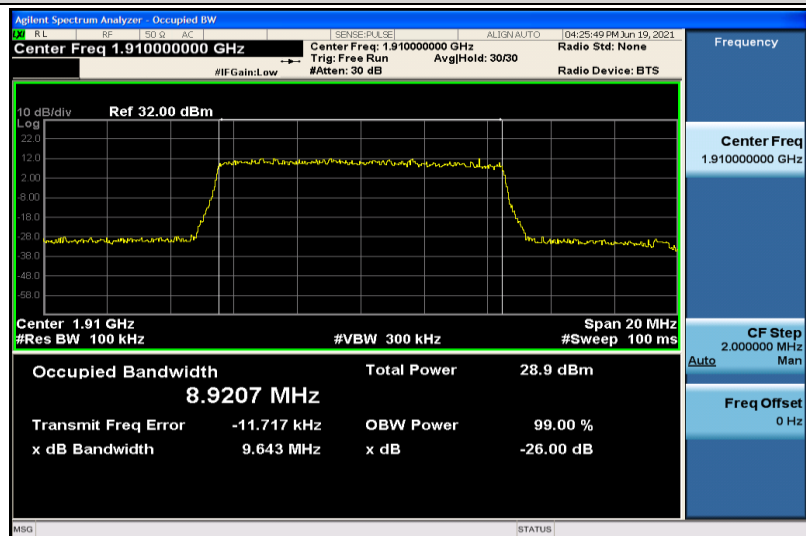
Band25-10MHz-16QAM-26640-50RB#0-8.9207
