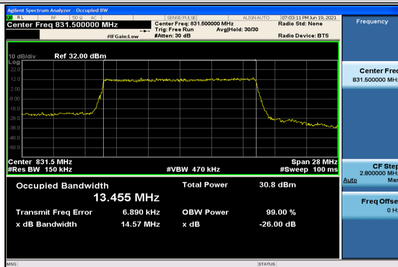
Band26-15MHz-QPSK-26865-75RB#0-13.455
