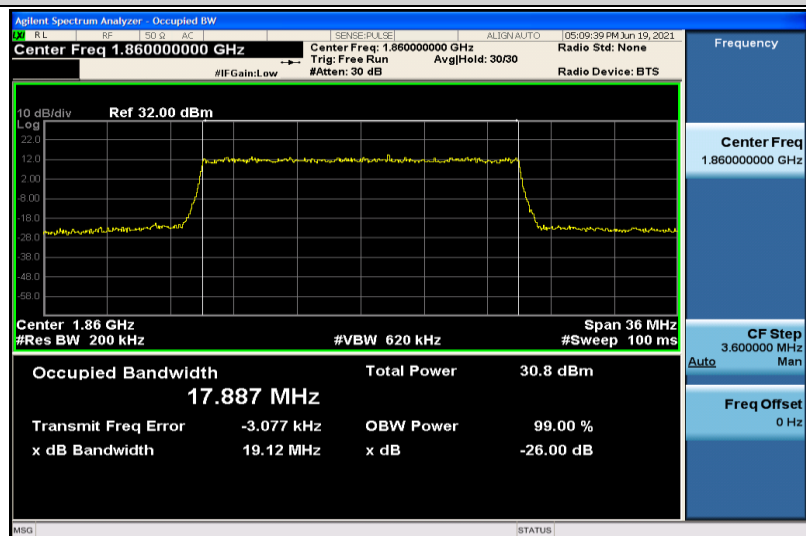
Band25-20MHz-QPSK-26140-100RB#0-17.887
