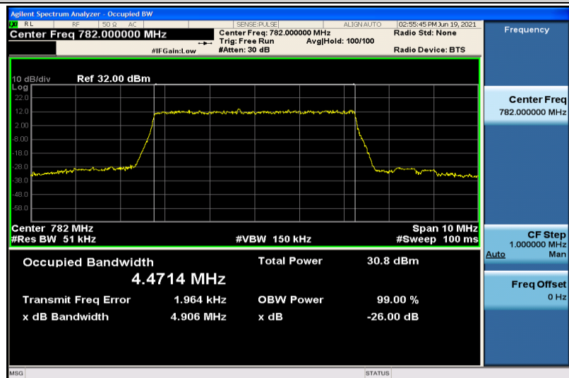
Band13-5MHz-QPSK-23230-25RB#0-4.4714
