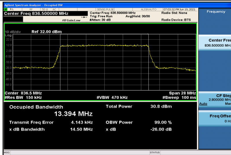
Band26-15MHz-QPSK-26915-75RB#0-13.394
