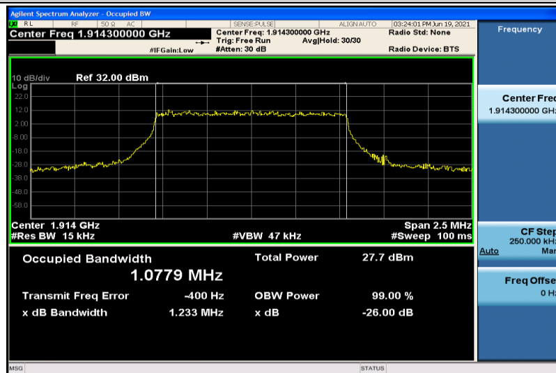
Band25-1.4MHz-16QAM-26683-6RB#0-1.0779
