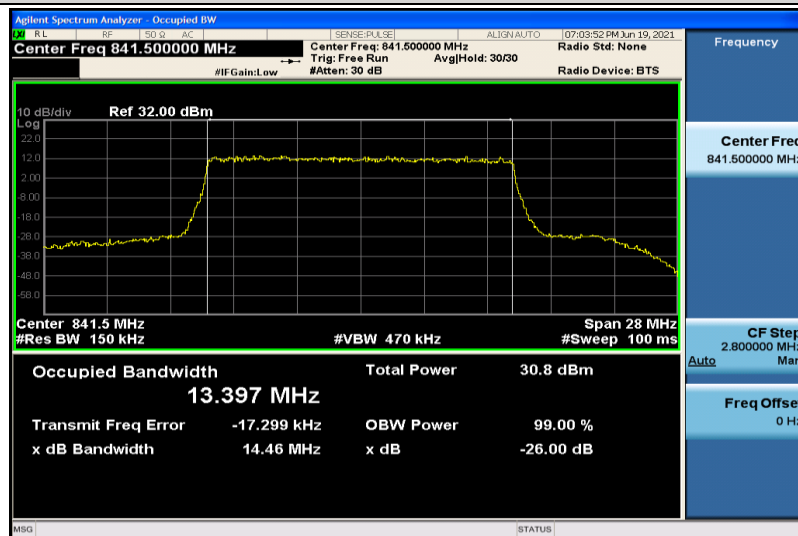
Band26-15MHz-QPSK-26965-75RB#0-13.397
