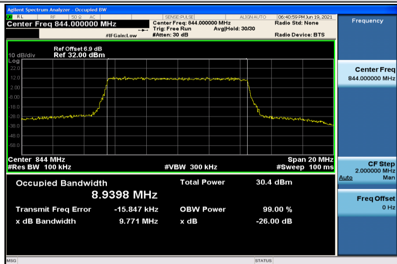
Band26-10MHz-QPSK-26990-50RB#0-8.9398
