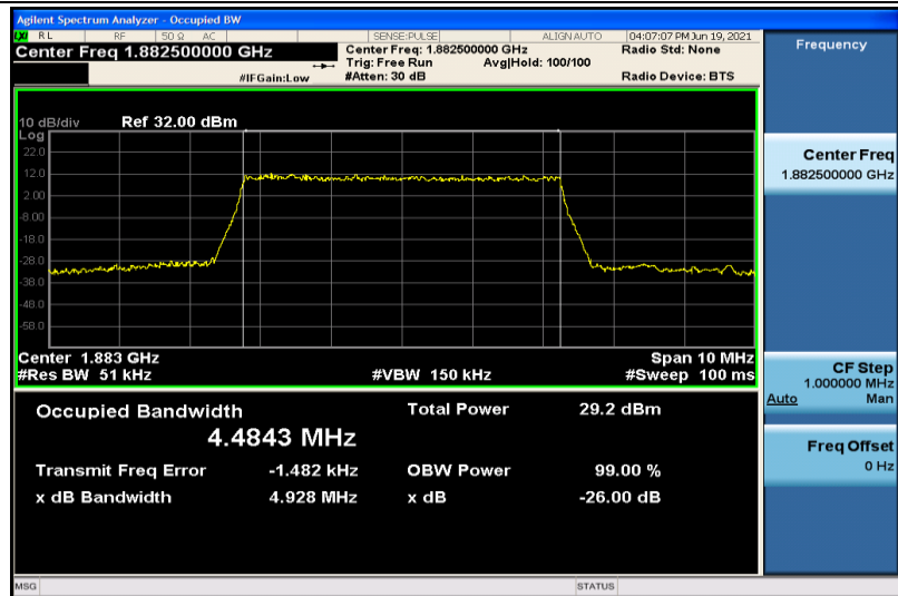
Band25-5MHz-16QAM-26365-25RB#0-4.4843
