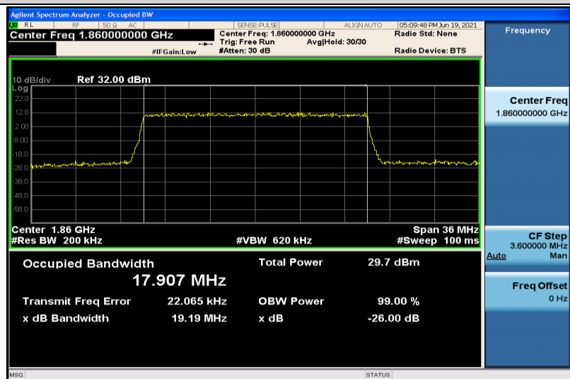
Band25-20MHz-16QAM-26140-100RB#0-17.907
