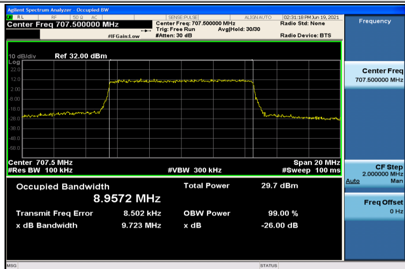
Band12-10MHz-16QAM-23095-50RB#0-8.9572
