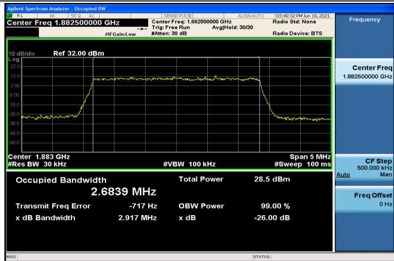
Band25-3MHz-16QAM-26365-15RB#0-2.6839
