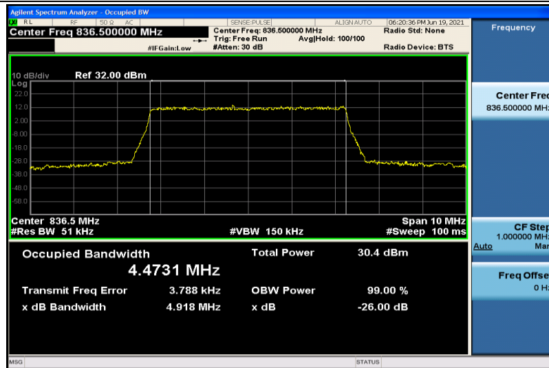
Band26-5MHz-QPSK-26915-25RB#0-4.4731
