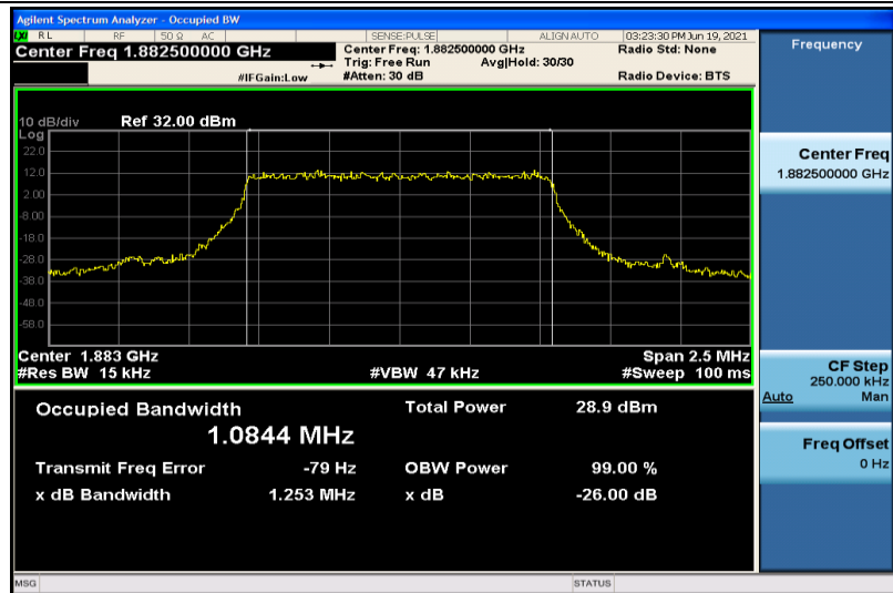
Band25-1.4MHz-QPSK-26365-6RB#0-1.0844
