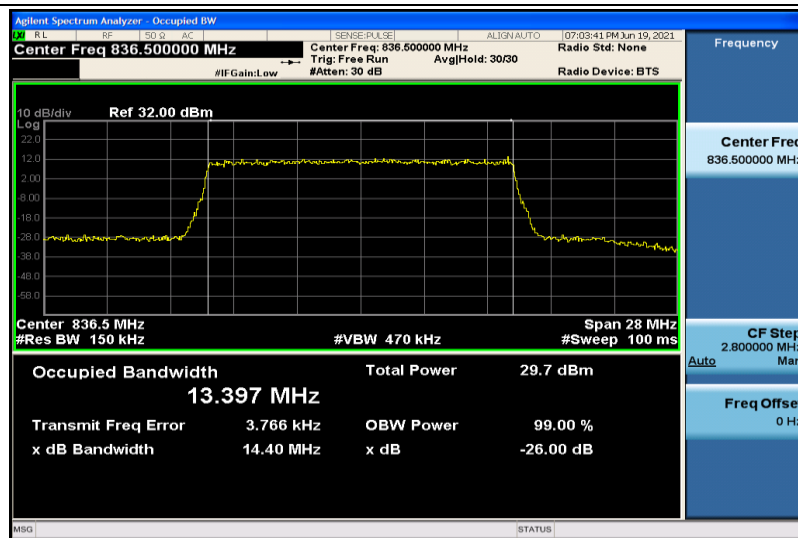
Band26-15MHz-16QAM-26915-75RB#0-13.397
