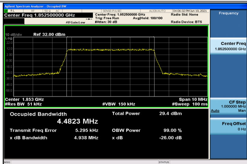
Band25-5MHz-16QAM-26065-25RB#0-4.4823
