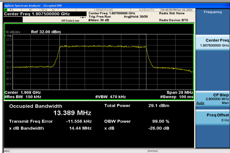
Band25-15MHz-16QAM-26615-75RB#0-13.389
