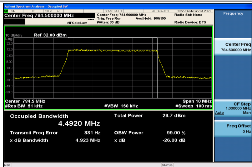
Band13-5MHz-16QAM-23255-25RB#0-4.4920
