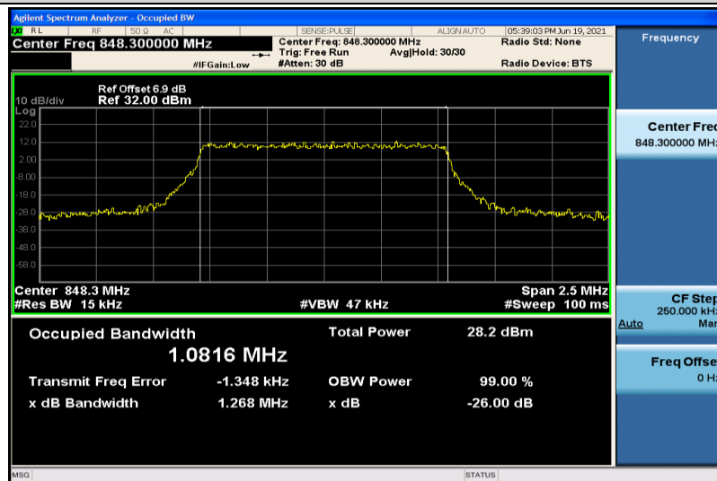
Band26-1.4MHz-16QAM-27033-6RB#0-1.0816
