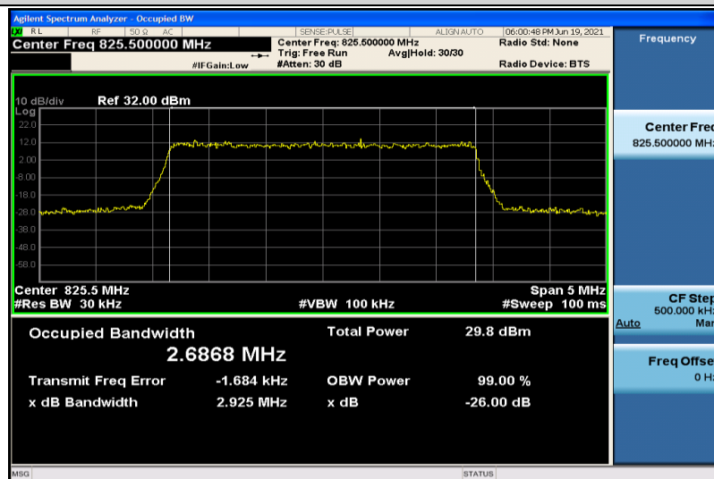
Band26-3MHz-QPSK-26805-15RB#0-2.6868
